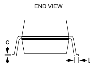
Package Dimensions for SC70-5
