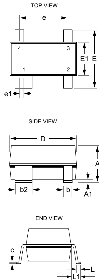
Package Dimensions for SOT143.
