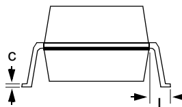
Package Dimensions for SC70-3.
