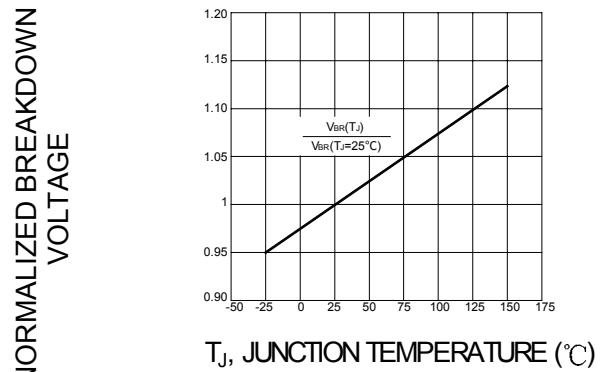
FIG.2- RELATIVE VARIATION OF BREAKDOWN VOLTAGE vs JUNCTION TEMPERATURE
