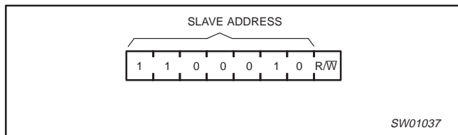
Figure 3. Slave address — PCA9553-1
