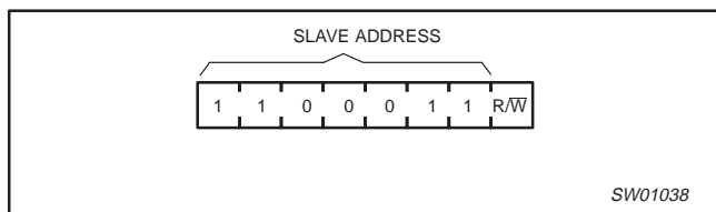
Figure 4. Slave address — PCA9553-2
