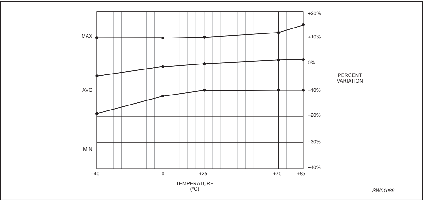
Figure 15. Typical frequency variation over process at V_{DD} = 3.0\text{ V to }5.5\text{ V}
