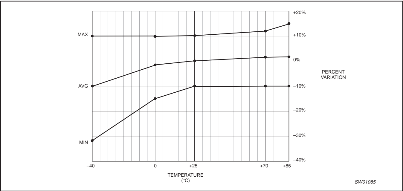
Figure 14. Typical frequency variation over process at V_{DD} = 2.3\text{ V to }3.0\text{ V}
