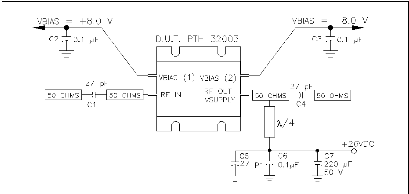
Test Circuit Schematic
