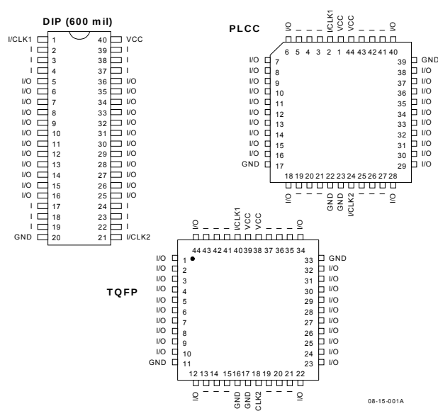
Figure 1. Pin Configuration
