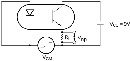
*5 Test Circuit for V_{CM}
