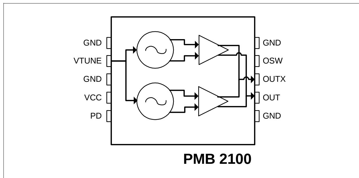
Figure 2-2 Block Diagram
