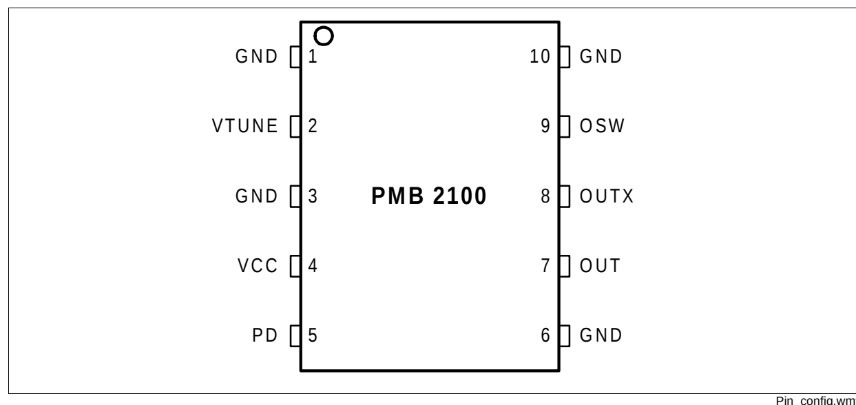
Figure 2-1 Pin Configuration
