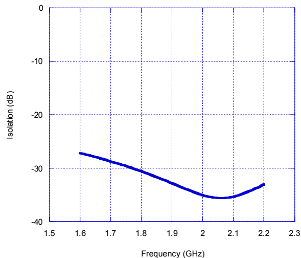
Figure 12. Output to Output Isolation – High Band Common Input
