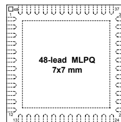
Figure 2. Package Type
