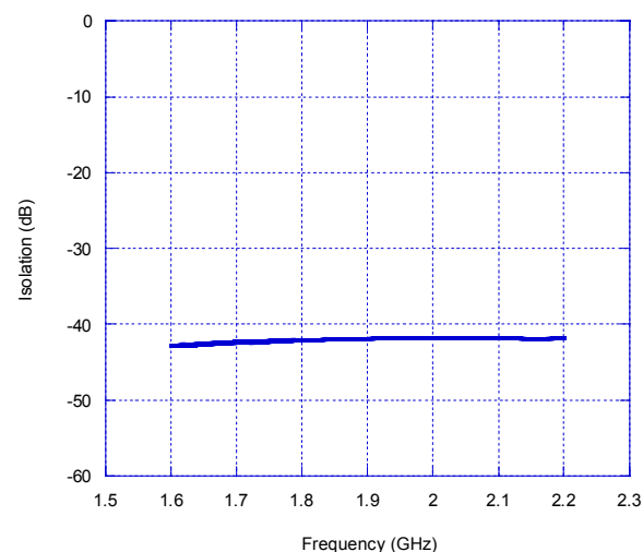
Figure 14. Input to Input Isolation – High Band to High Band
