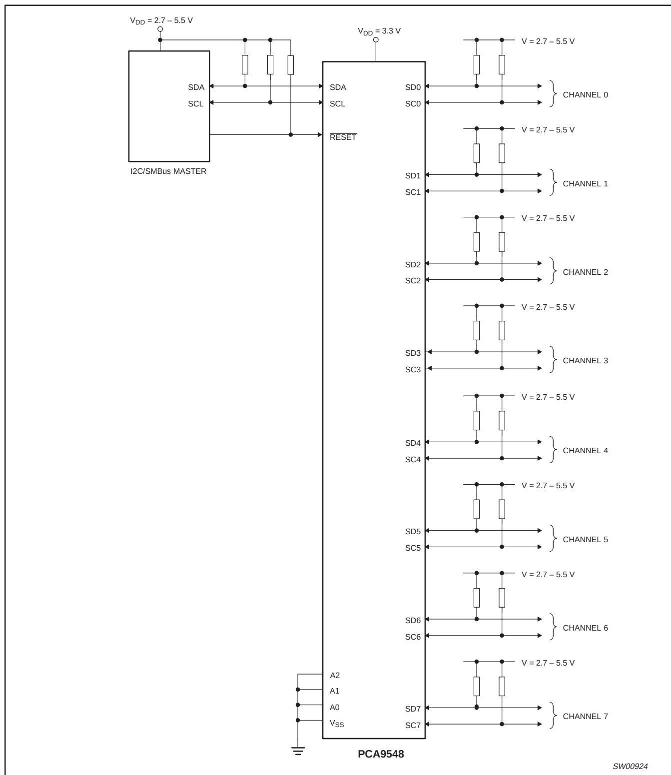
Figure 12. Typical application
