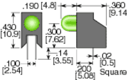
Series PCT230 Figure 1. Standard Projection
