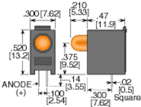
Series PCT240 Figure 2. Low Projection
