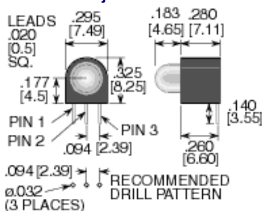
Pin-Out Information
