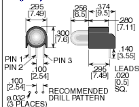
Pin-Out Information
