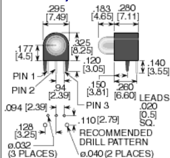
Pin-Out Information
