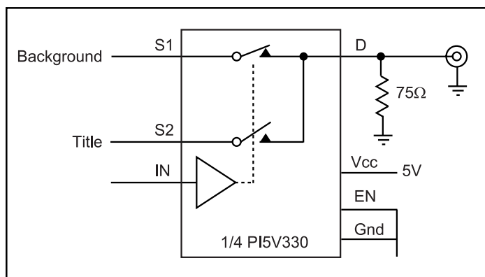
Figure 1. Picture-In-Picture Switch
