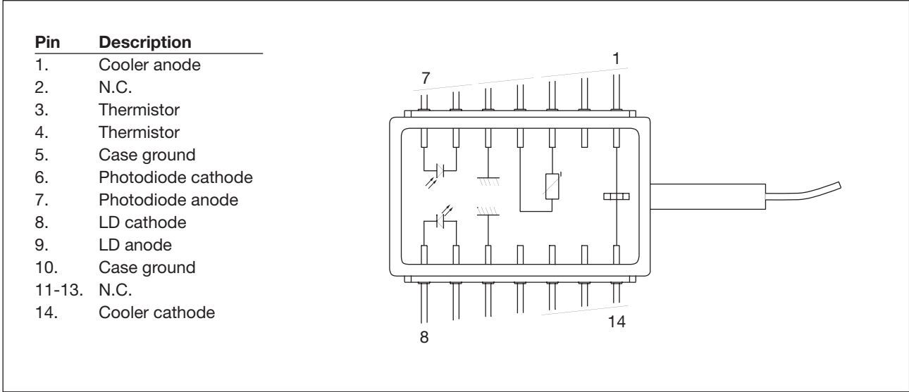
Figure 2. Pin description
