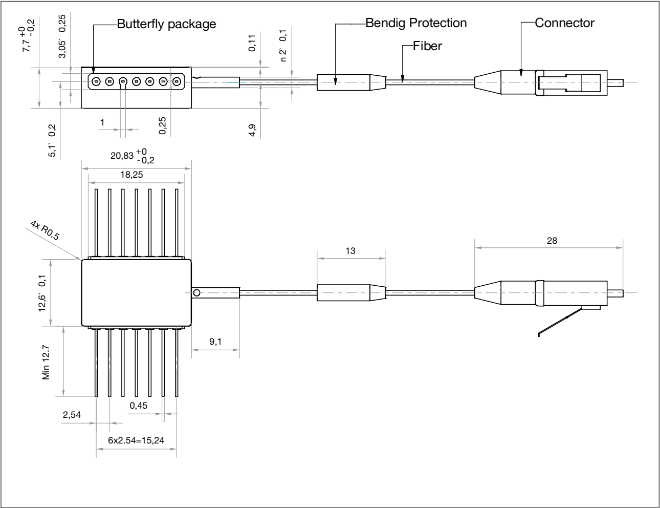
Figure 1. Mechanical outline
