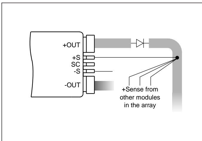
Figure 12—OR'ing diodes connections.
