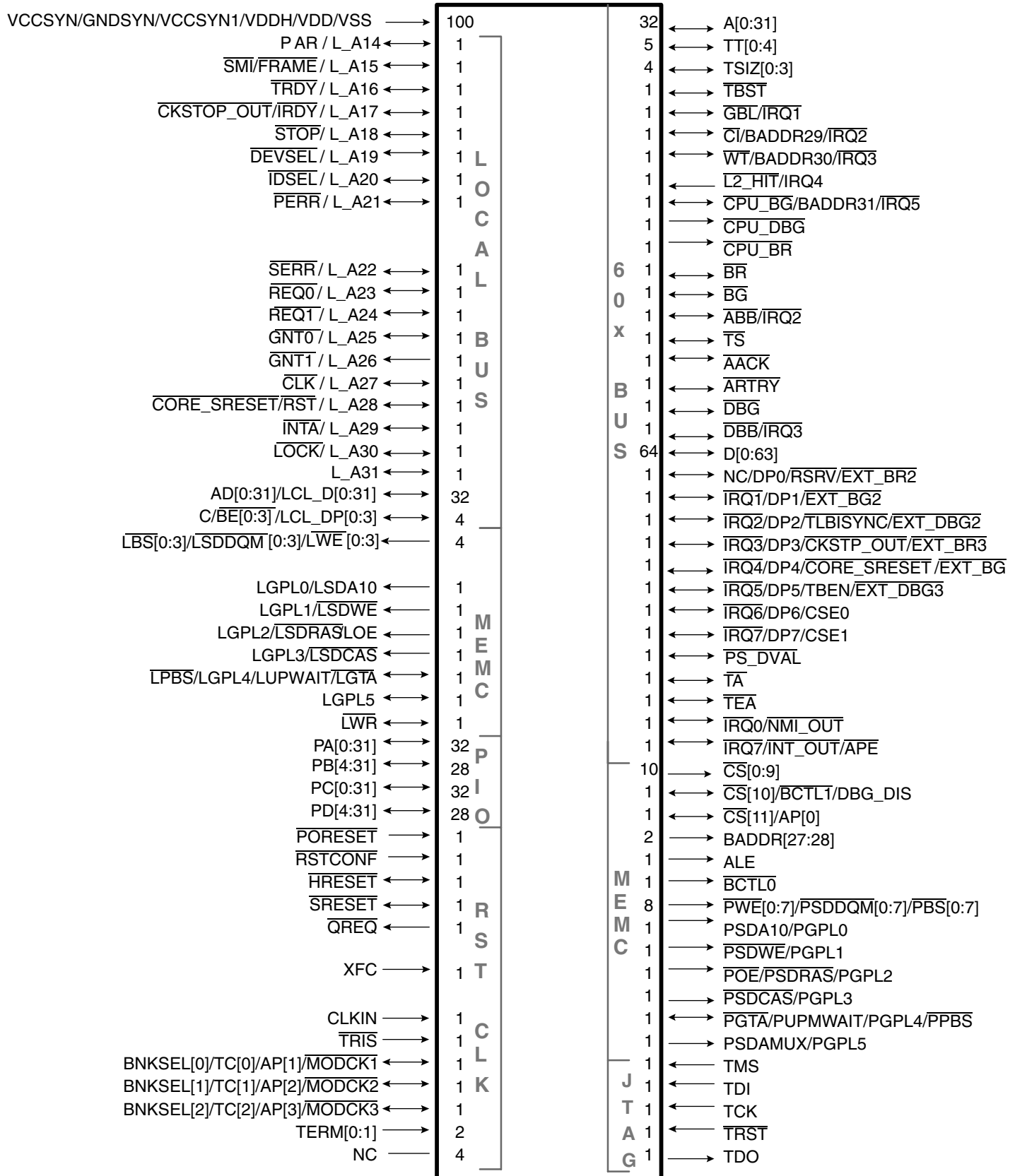
Figure 2. PowerQUICC II External Signals
