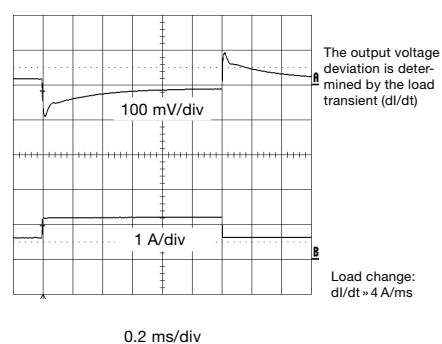
Dynamic load response (typ) @ +25^\circ\text{C}
