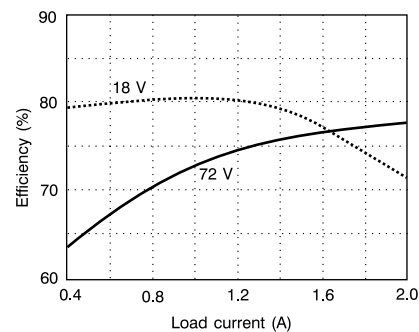
Efficiency (typ) @ T_A = +25^\circ\text{C}
