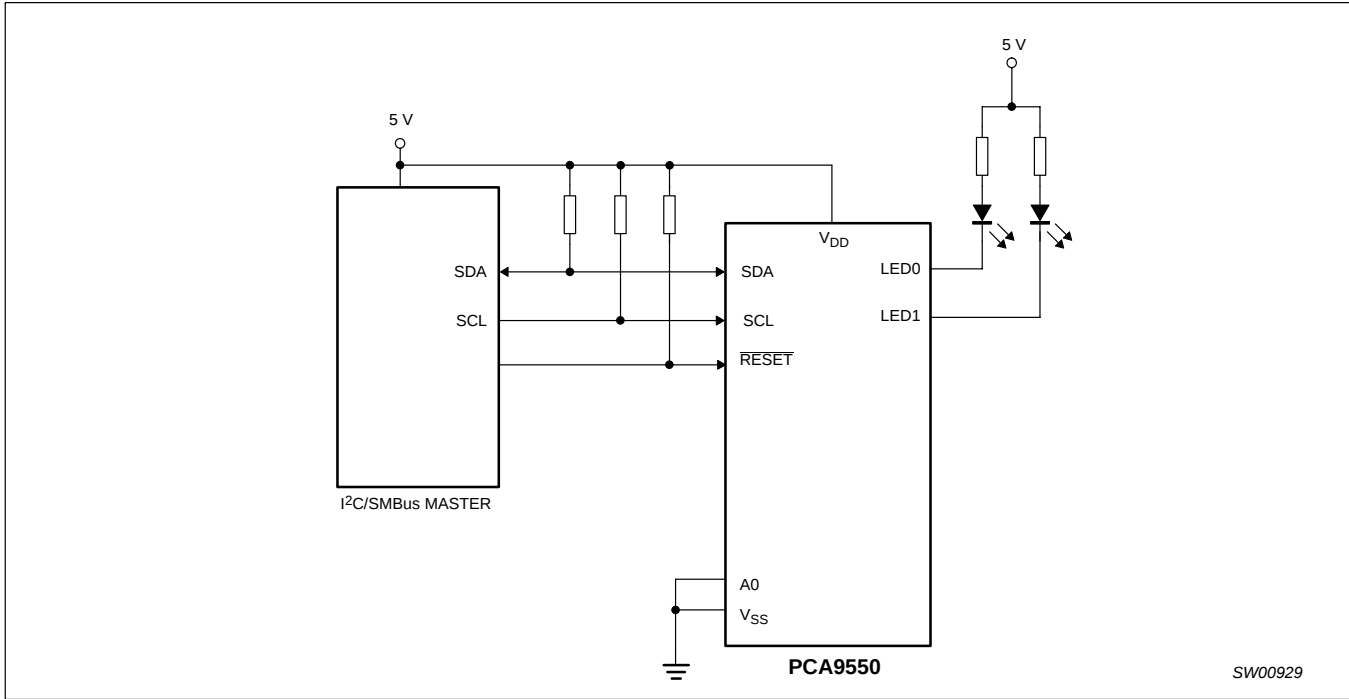
Figure 12. Typical application
