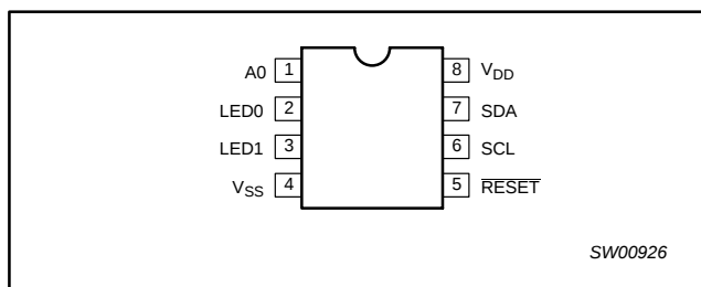
Figure 1. Pin configuration
