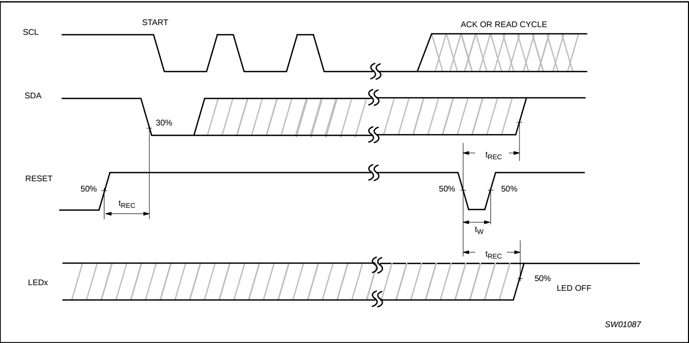
Figure 17. Definition of \overline{\text{RESET}} timing
