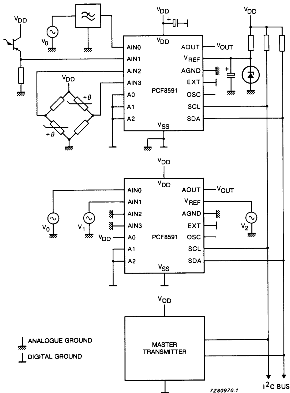
Fig.20 Application diagram.
