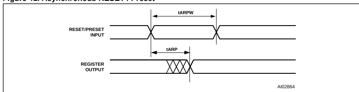
Figure 41. Asynchronous \overline{\text{RESET}} / Preset
