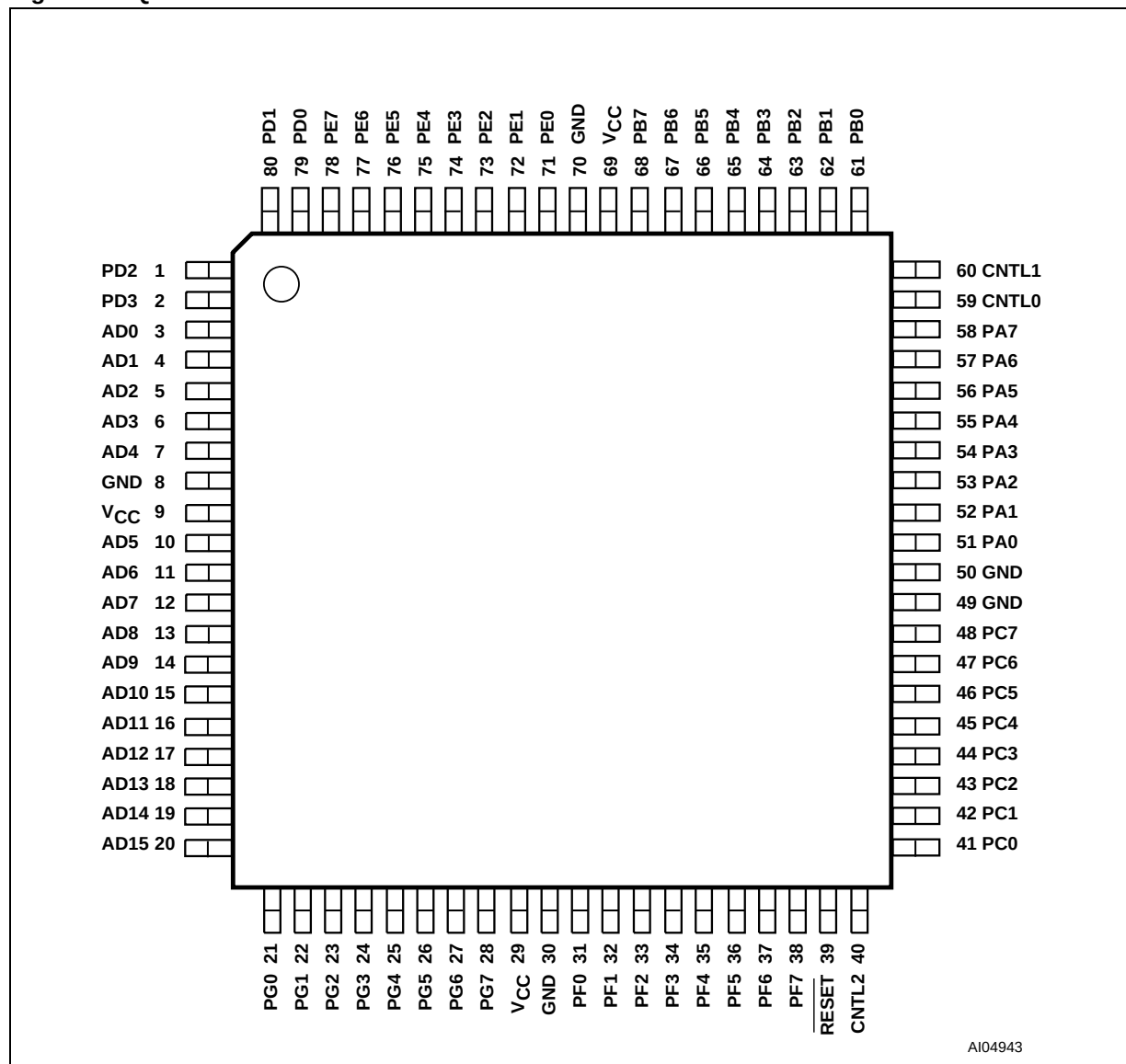
Figure 3. TQFP80 Connections
