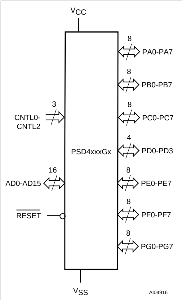
Figure 2. Logic Diagram
