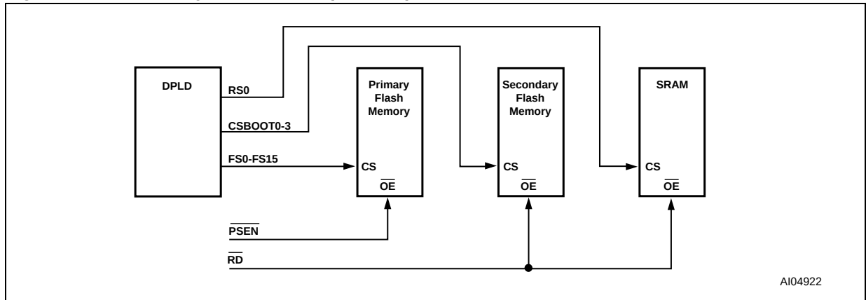
Figure 9. 8031 Memory Modules – Separate Space
