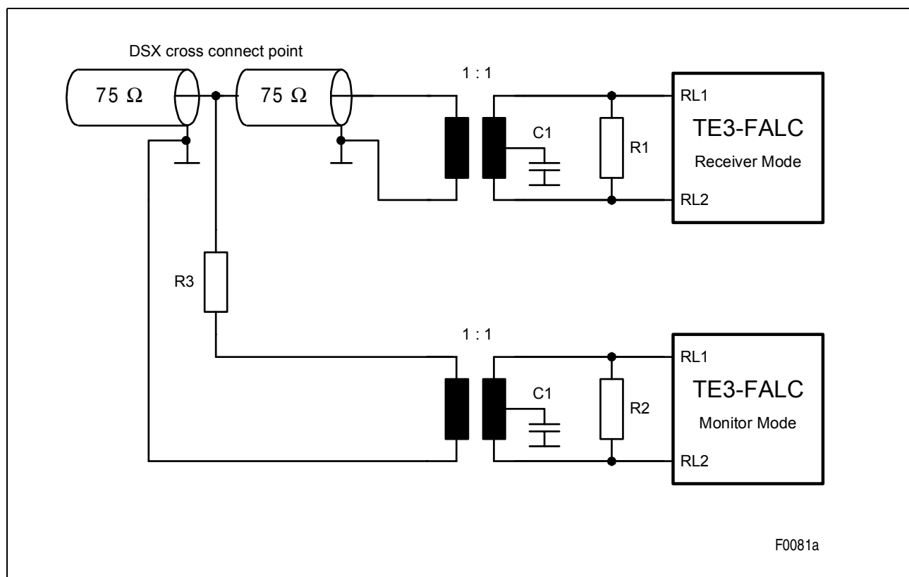
Figure 16 DS3 Line Monitoring
