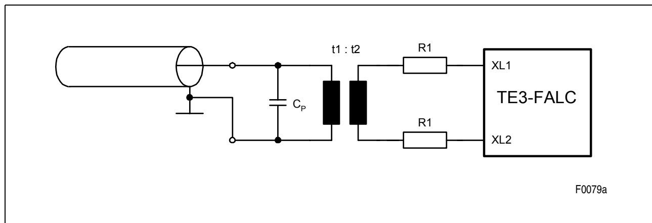
Figure 21 Transmitter Configuration
