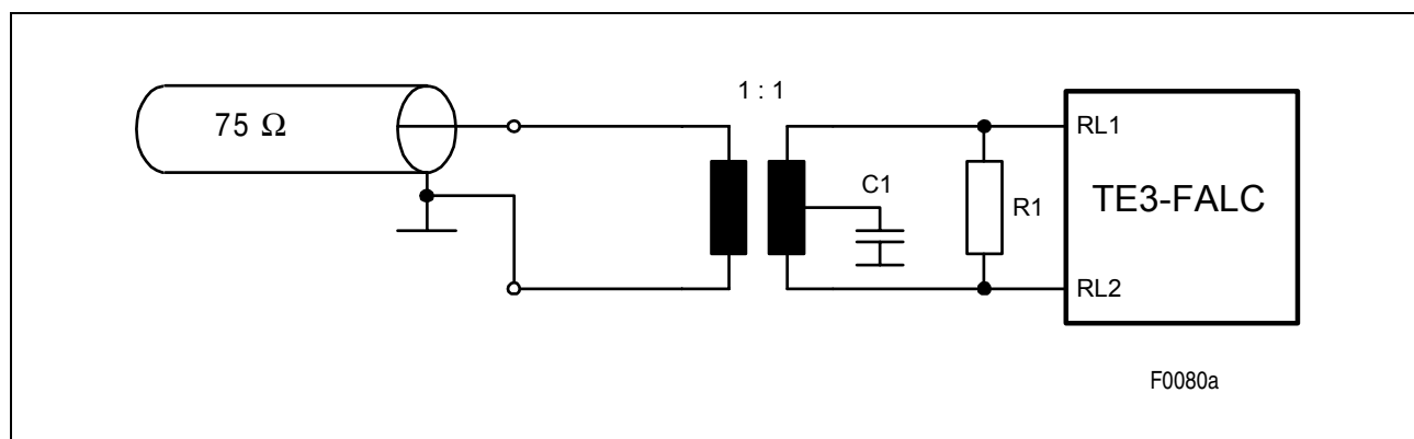
Figure 15 Standard Receiver Configuration
