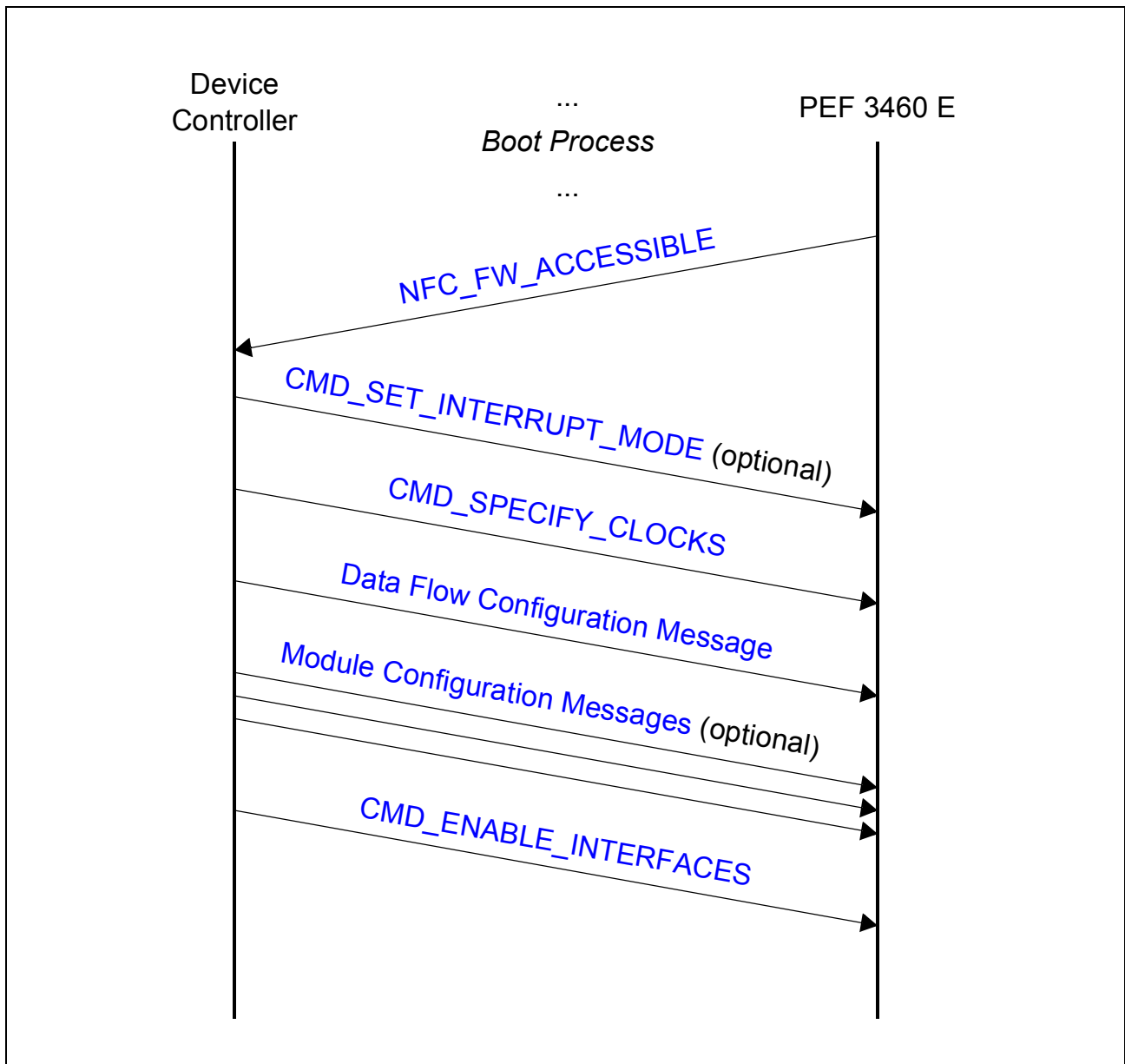
Figure 13 Minimum Initialization Message Flow
