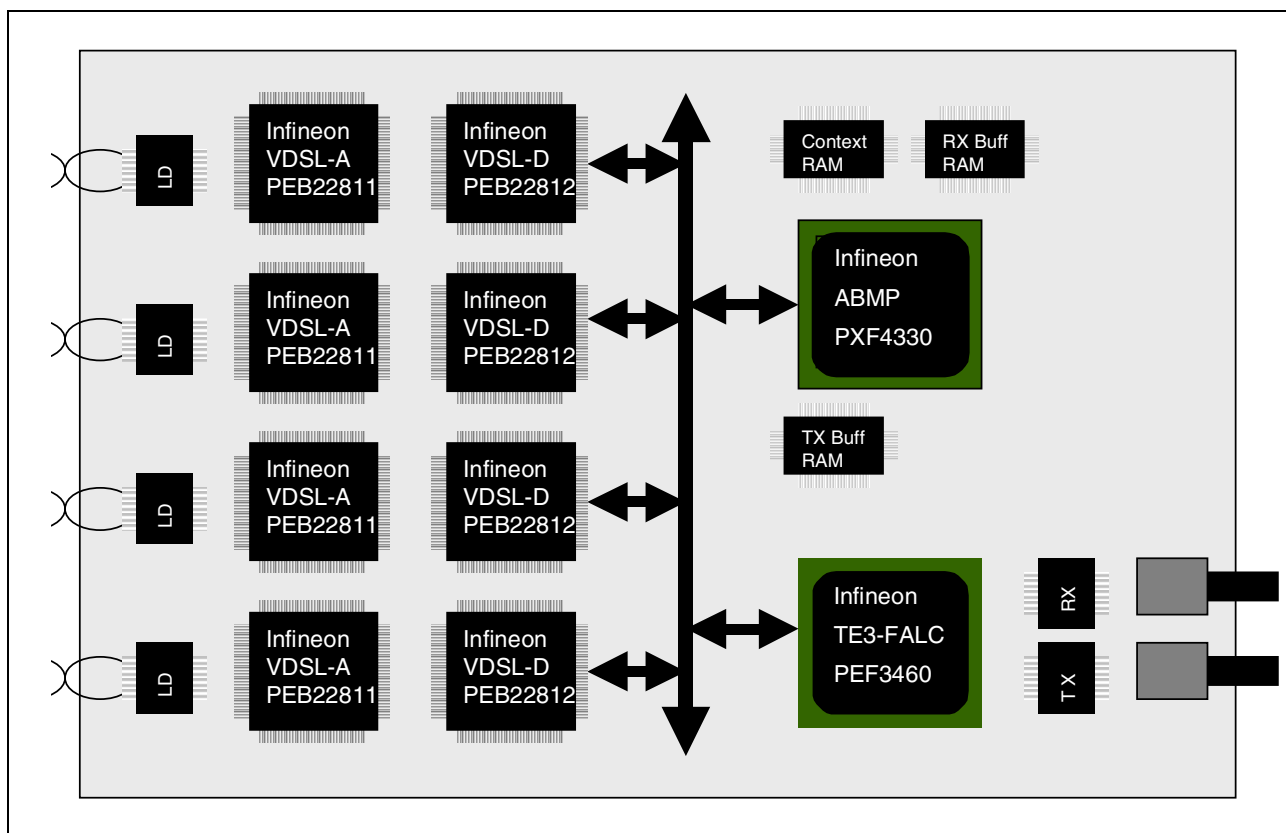
Figure 4 Customer based MDU with T3/E3 uplink
