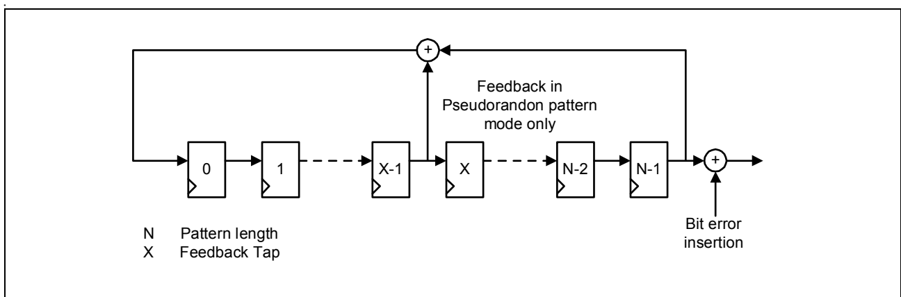
Figure 8 Pattern Generator
