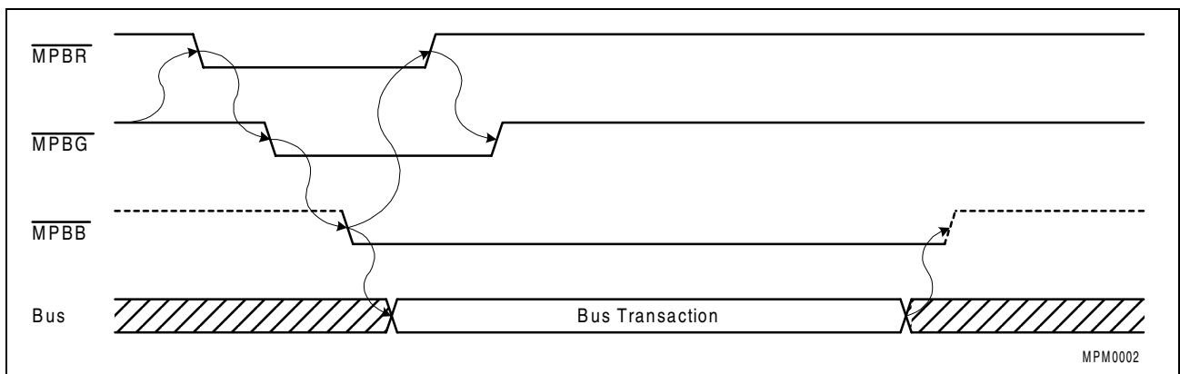
Figure 26 Motorola Arbitration
