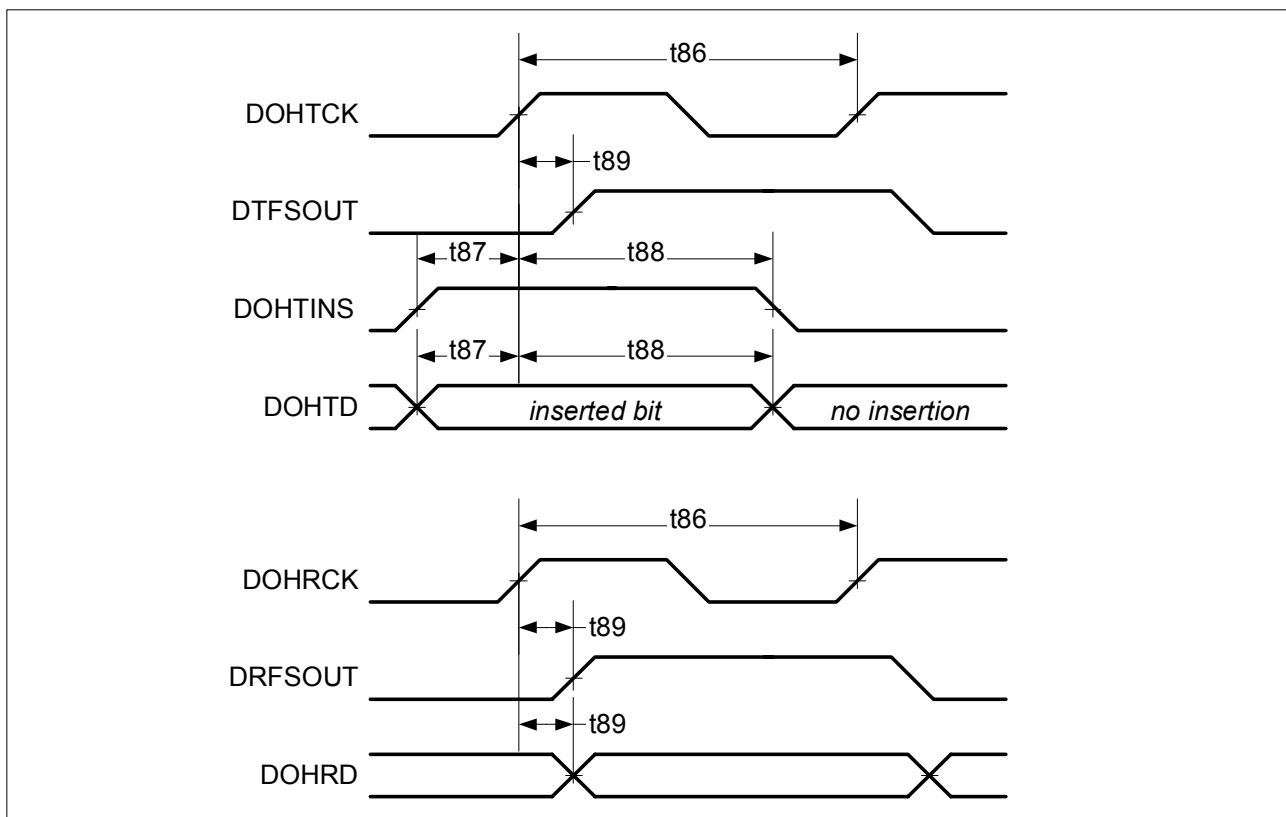
Figure 39 Overhead Access Interface Timing
