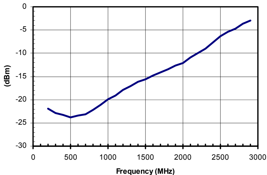
Figure 3. Typical RF Input Sensitivity
