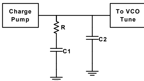
Figure 7. Typical PE3239 Loop Filter Application Example
