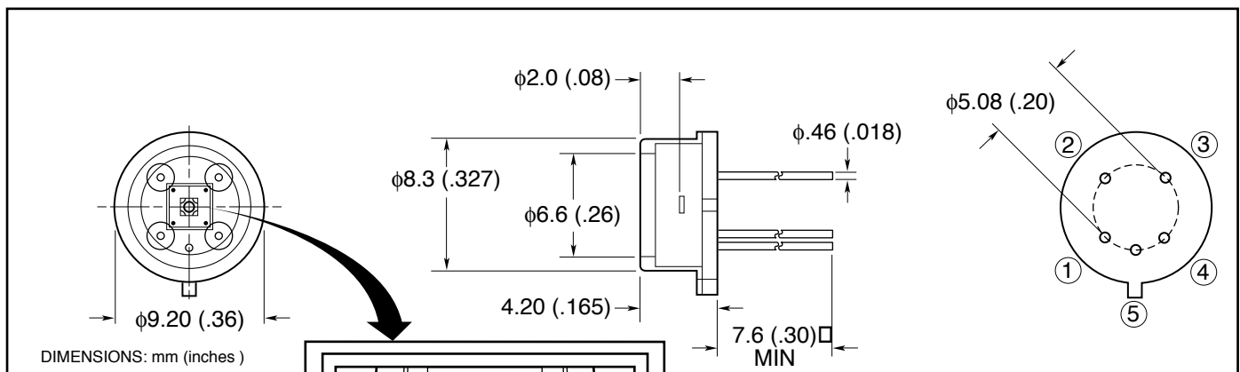
OUTLINE DIMENSIONS
