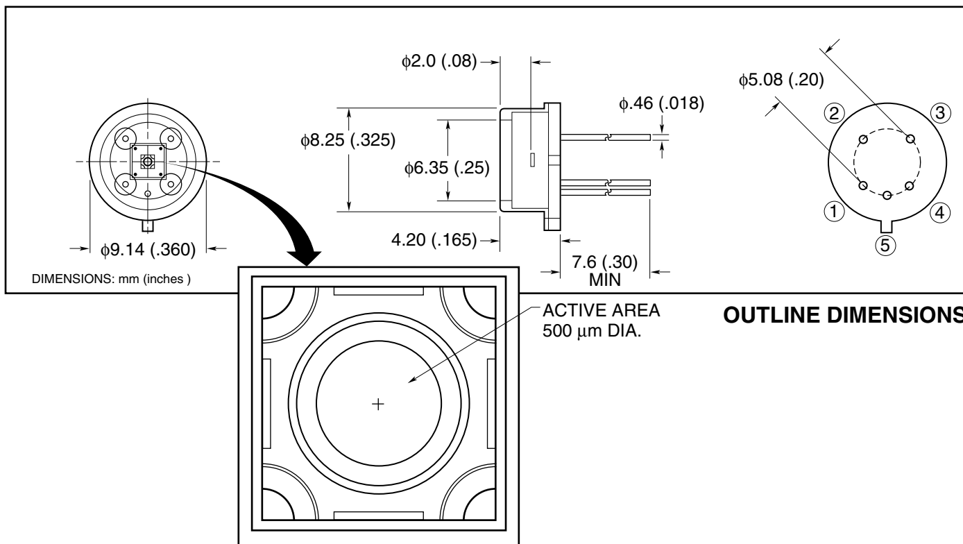
APD CHIP
