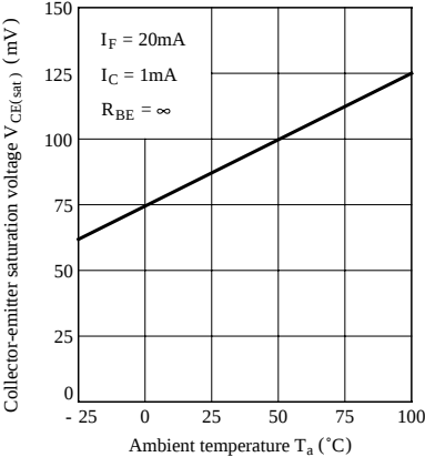
Fig.10 Collector-emitter Saturation Voltage vs. Ambient Temperature
