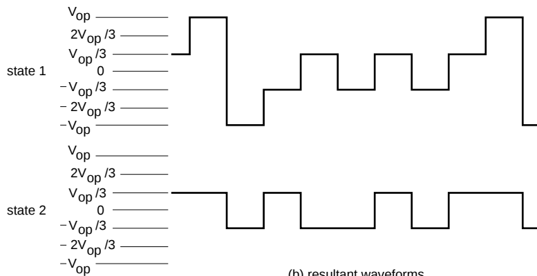
(b) resultant waveforms at LCD segment
