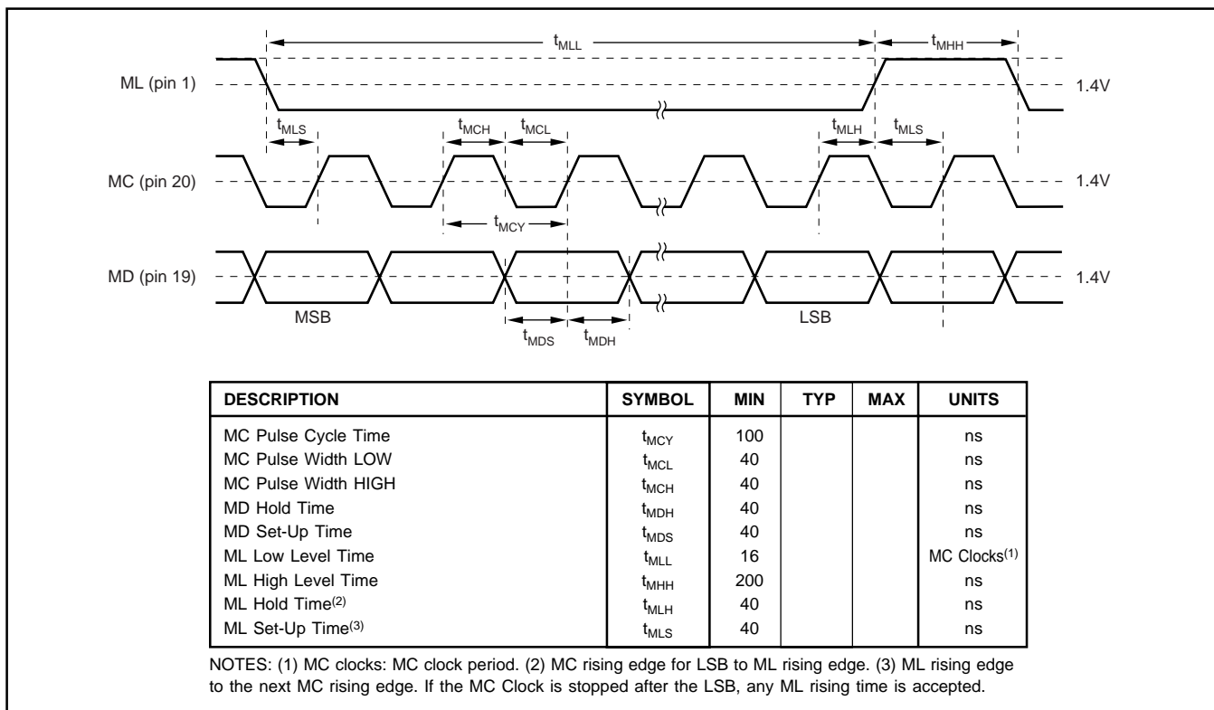
FIGURE 9. Control Data Input Timing.
