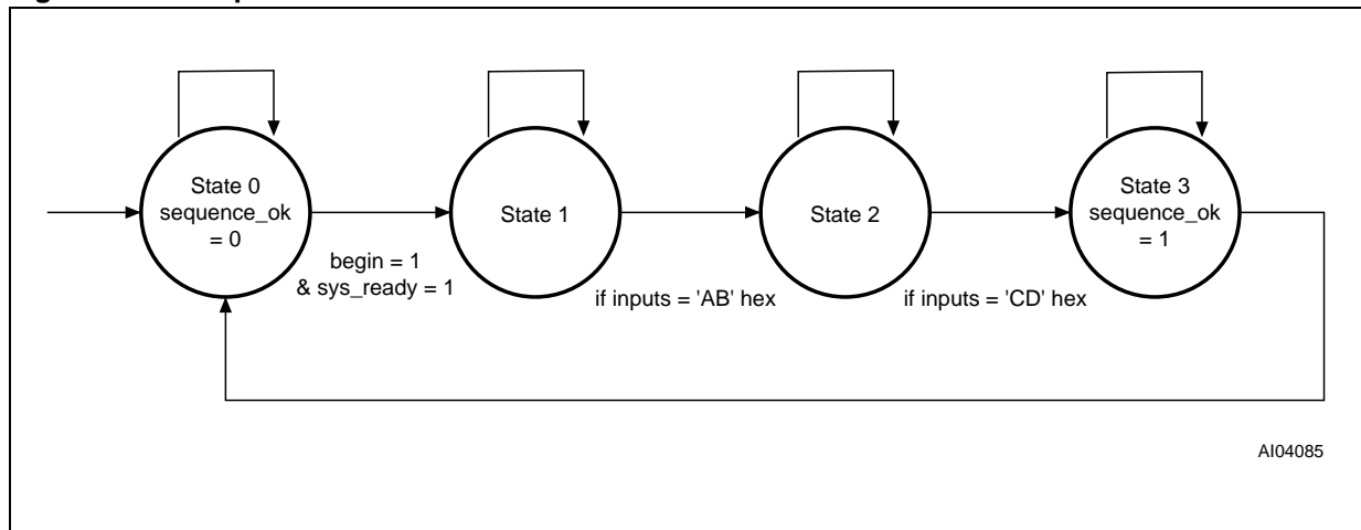
Figure 44. Example State Machine
