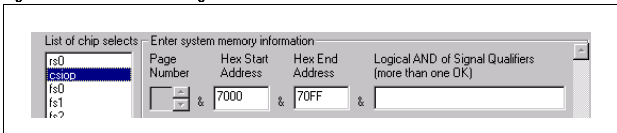
Figure 11. CSIOP Address Range
