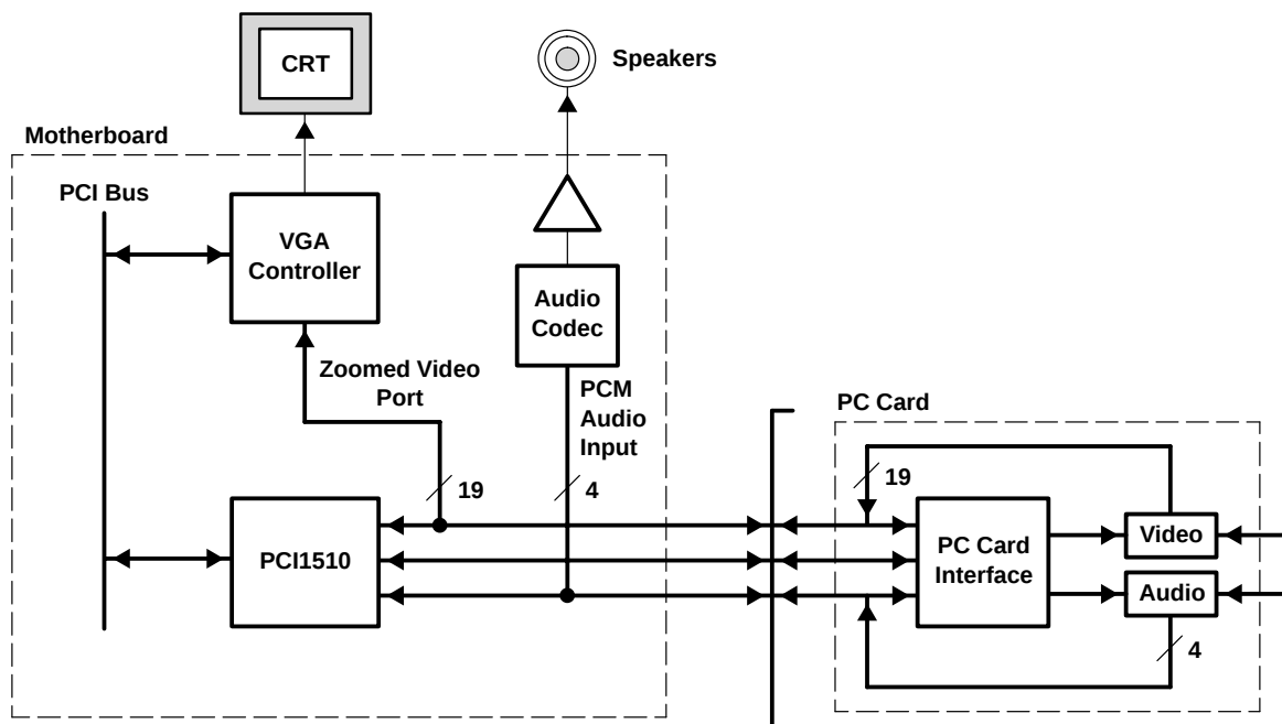
Figure 3-4. Zoomed Video Implementation Using the PCI1510
