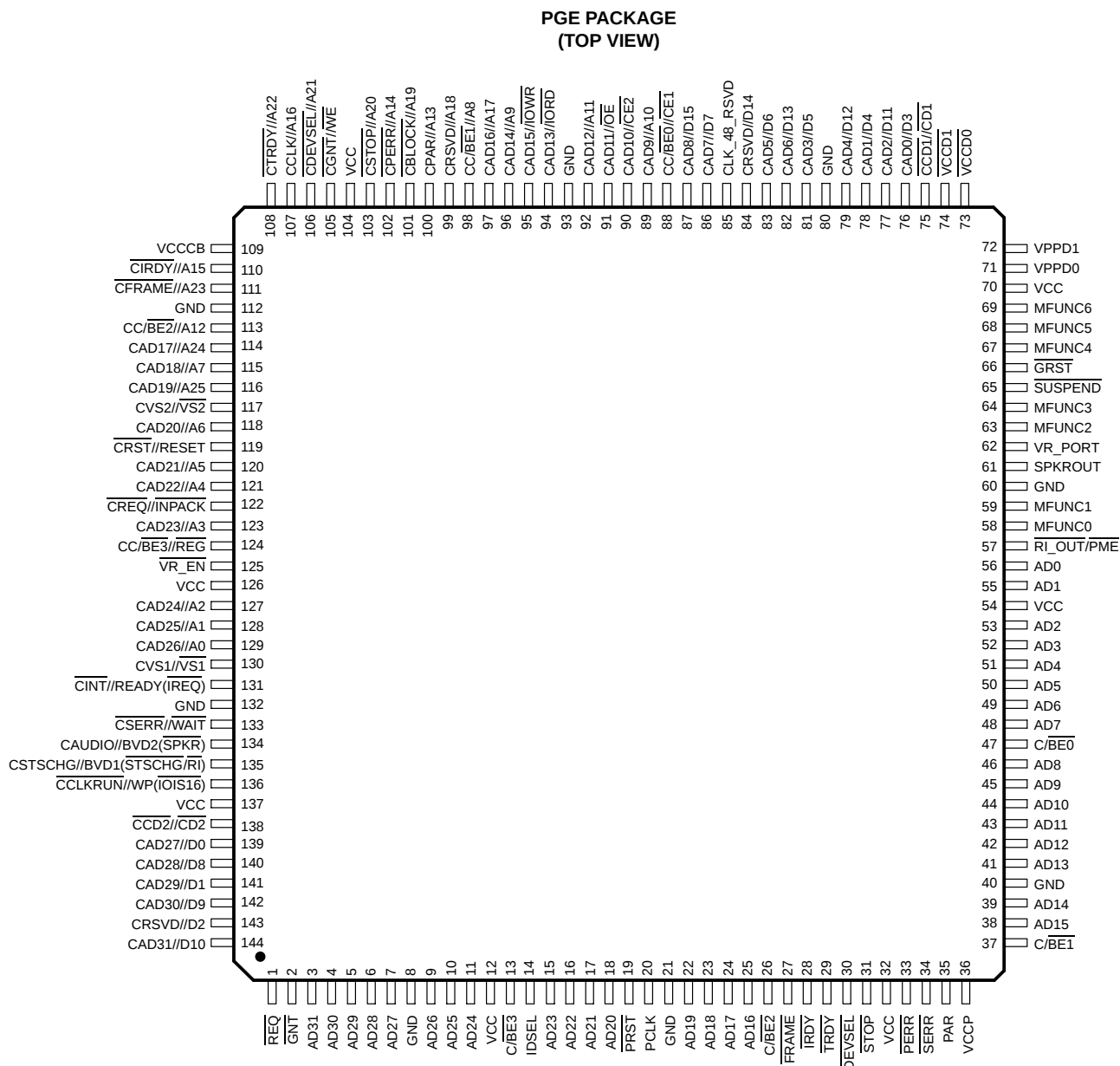
Figure 2–2. PCI1510 PGE-Package Terminal Diagram
