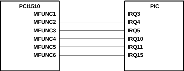
Figure 3–14. IRQ Implementation
