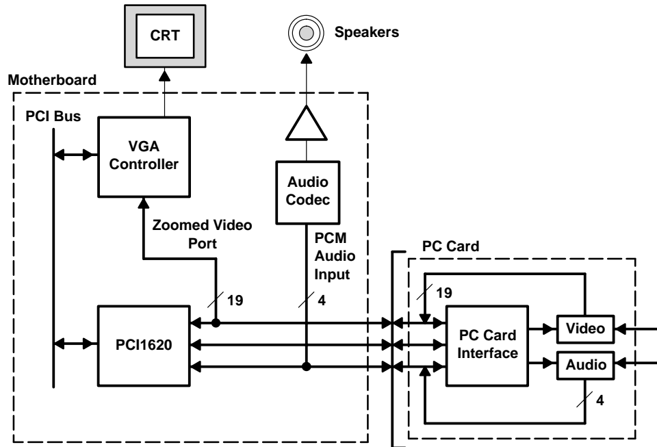
Figure 3-6. Zoomed Video Implementation Using PCI1620
