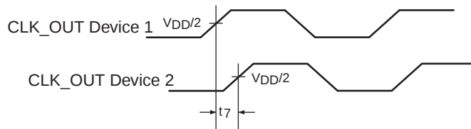
Device-Device Skew
