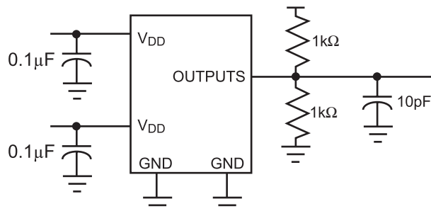
Test Circuit #2
