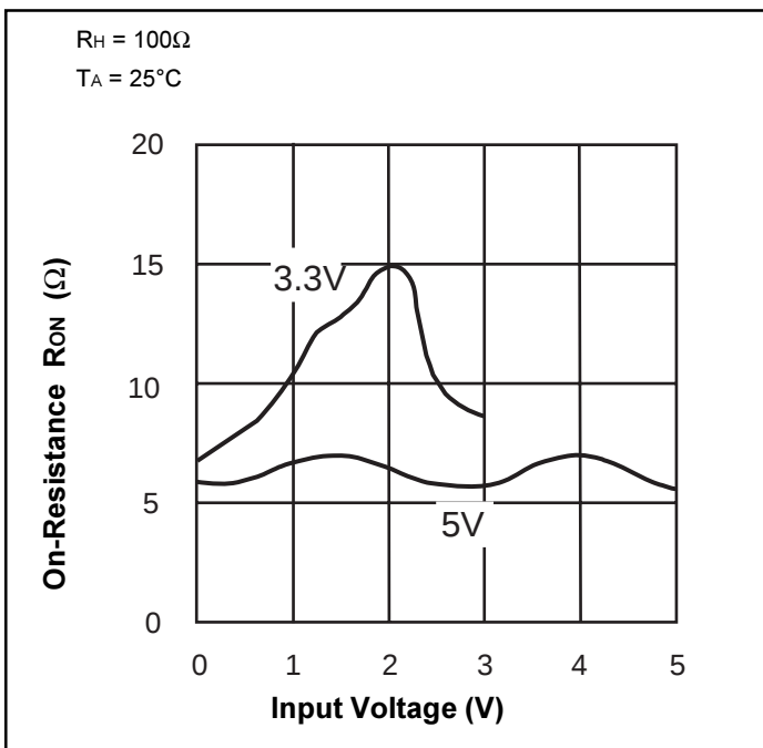
Figure 7. On-Resistance vs Input Voltage
