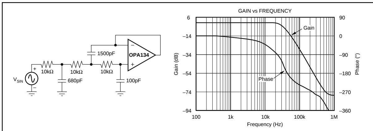
FIGURE 9. 3rd-Order LPF.
