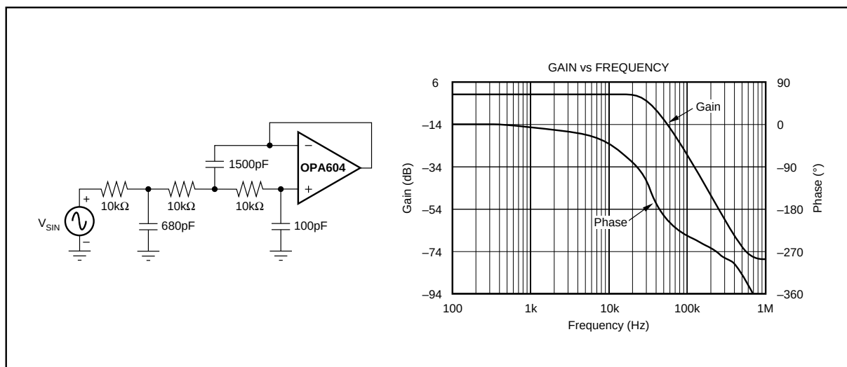
FIGURE 12. 3rd-Order LPF.
