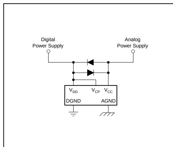
FIGURE 15. Latch-up Prevention Circuit.
