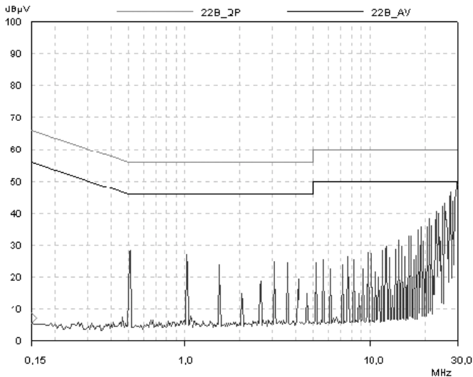
PKF 4928A with 51μH common mode and 10 μH series inductor
