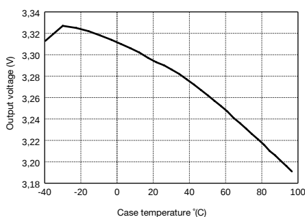
Temperature coefficient
