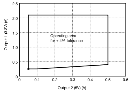
Cross regulation output 1 (3.3V)
