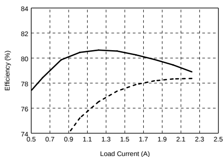
Efficiency (typ) @ T_A = +25^\circ\text{C}
