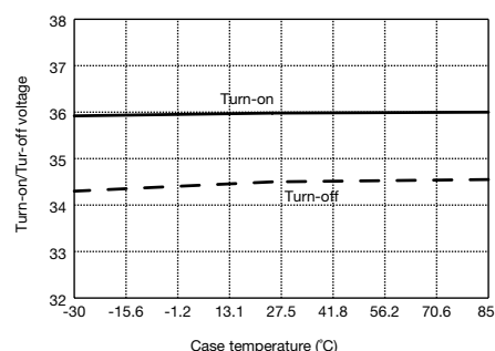
Turn-on/turn-off input voltage
