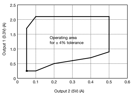
Cross regulation output 2 (5V)
