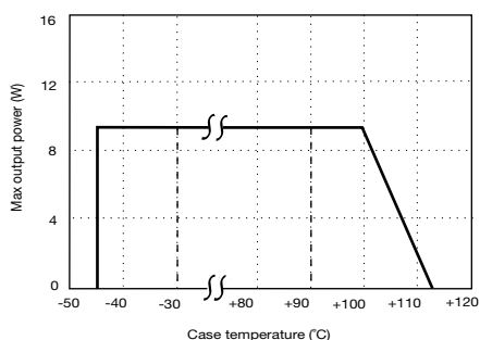
Power derating
