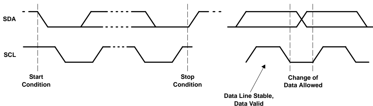
Figure 3–10. Serial Bus Start/Stop Conditions and Bit Transfers
