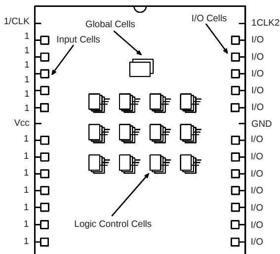
Figure 2. Block Diagram
