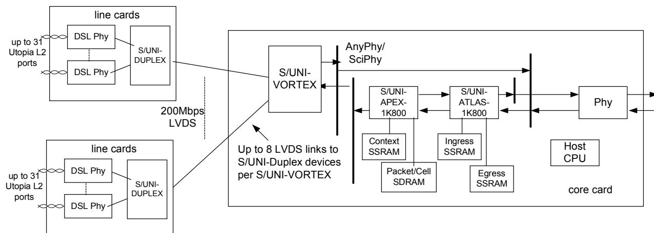
Figure 1 S/UNI-ATLAS-1K800 in OC3 mini-DSLAM Application
