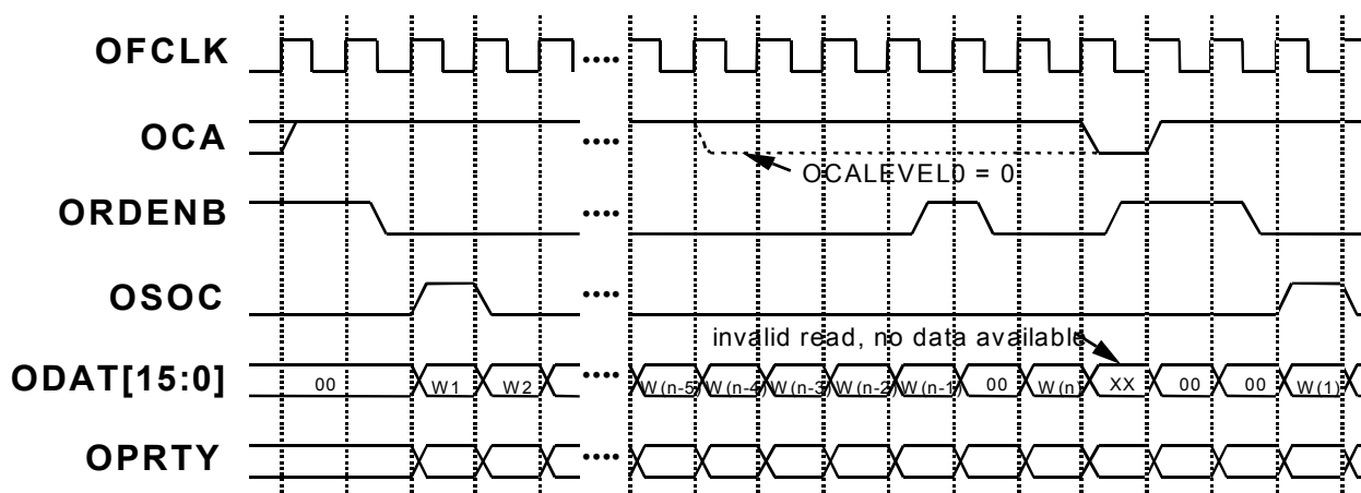
Figure 43 Ingress Output Cell Interface (OTSEN=0)
