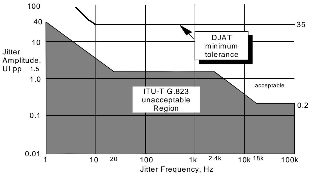
Figure 3 - DJAT Jitter Tolerance
