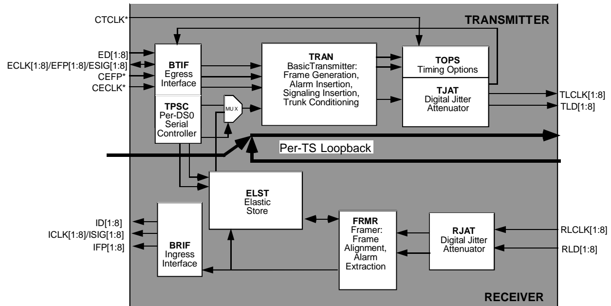
Figure 26 - Per-TS Loopback
