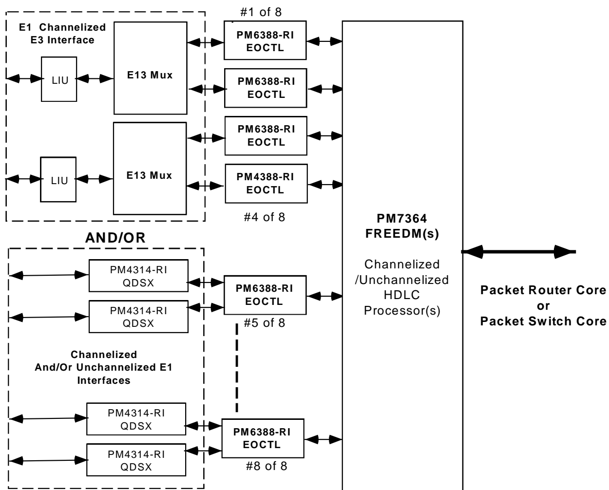
Figure 1 - High Density Channelized Port Card Application
