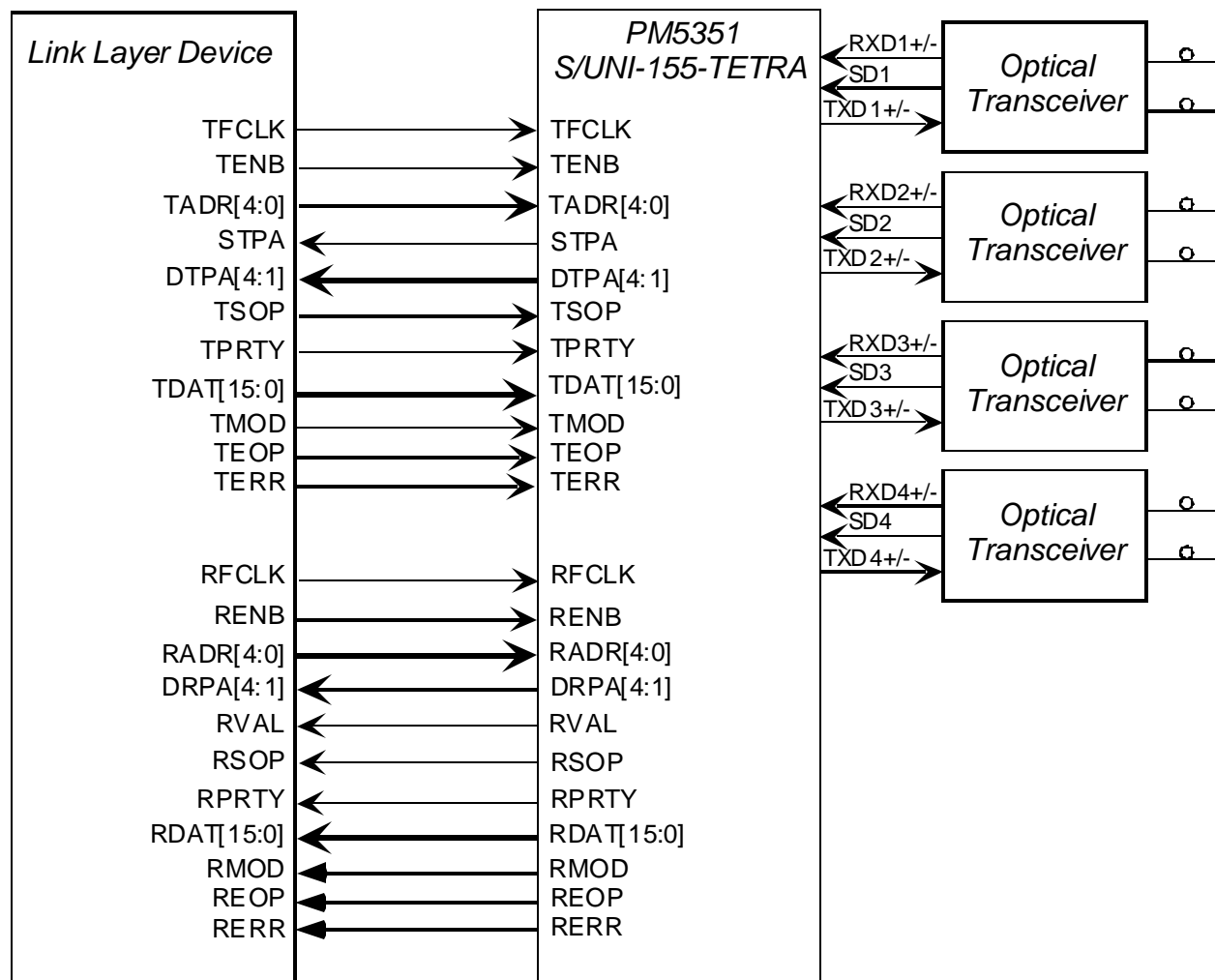
Figure 2: Typical STS-3c (STM-1) Packer over SONET/SDH (PPP) Application
