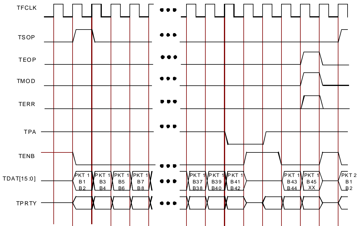
Figure 37: Transmit POS System Interface Timing
