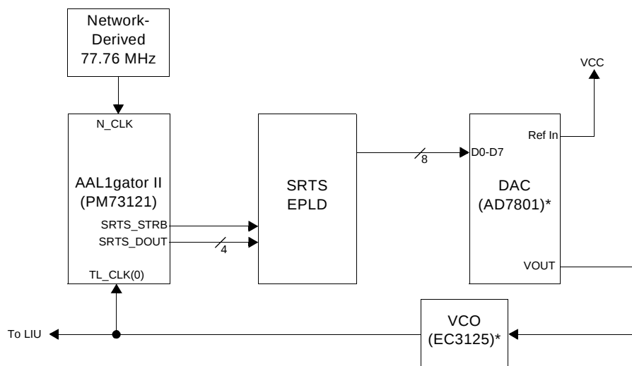
Figure 92. SRTS-Based Clock Recovery Circuit
