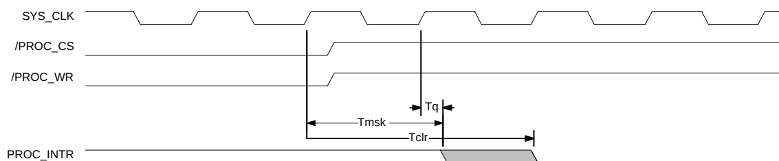
Figure 77. Interrupt Timing
