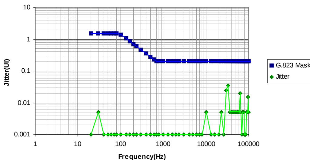
Figure 98. Nominal E1 Clock with no Jitter Attenuator
