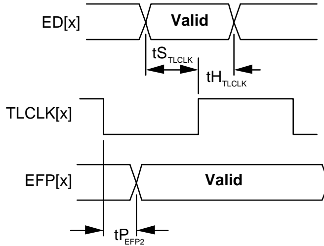
Figure 42 - Egress Interface Timing - Clock Master: Full DS1 Mode
