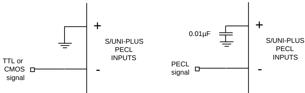
Figure 11 - Single Ended Driving Differential Inputs
