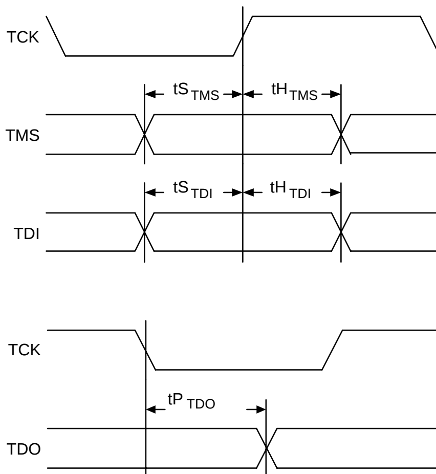
Fig. 21 JTAG Port Interface Timing
