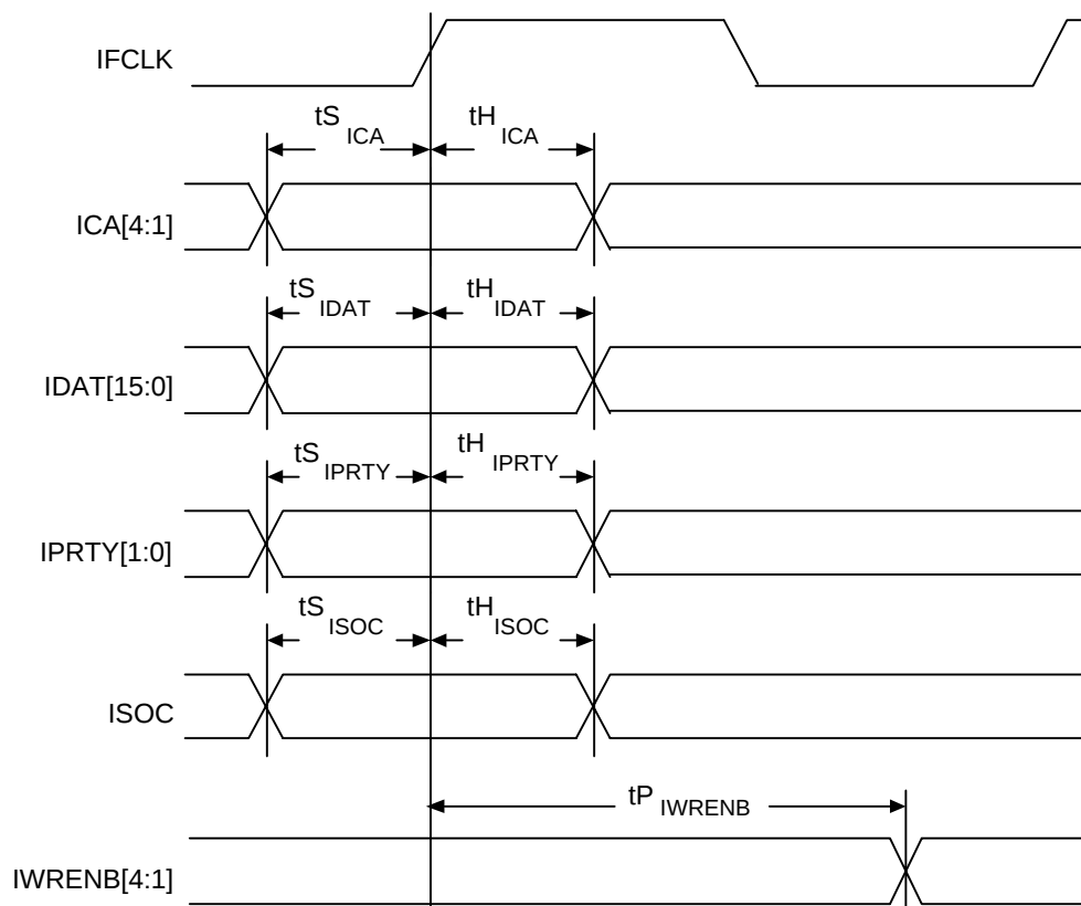
Fig. 17 Input Cell Interface Master (IPOLL=0) Timing
