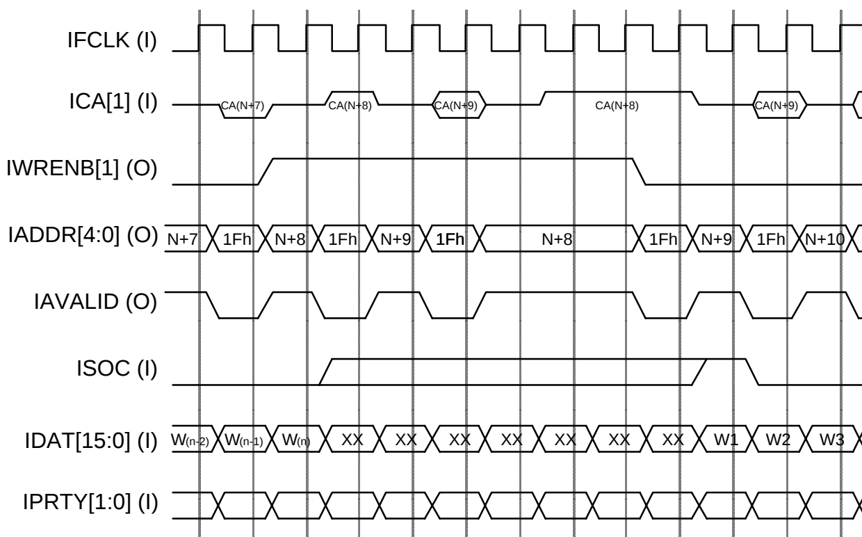
Fig. 12 Input Cell Interface Address Line Polling Master Configuration (IPOLL=1) – Example 2
