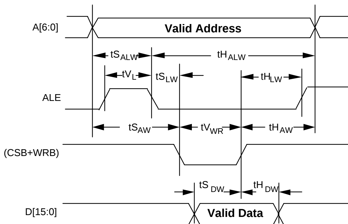
Fig. 16 Microprocessor Interface Write Timing
