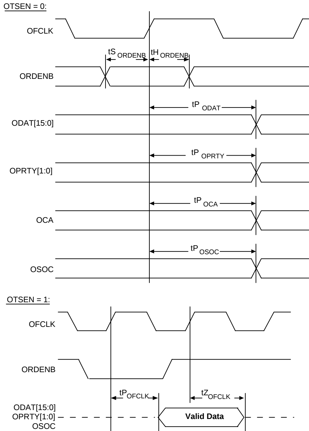
Fig. 19 Output Cell Interface Slave Timing
