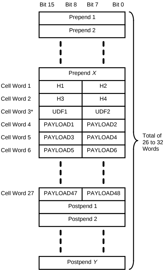
Fig. 7 Sixteen Bit Wide Cell Format
