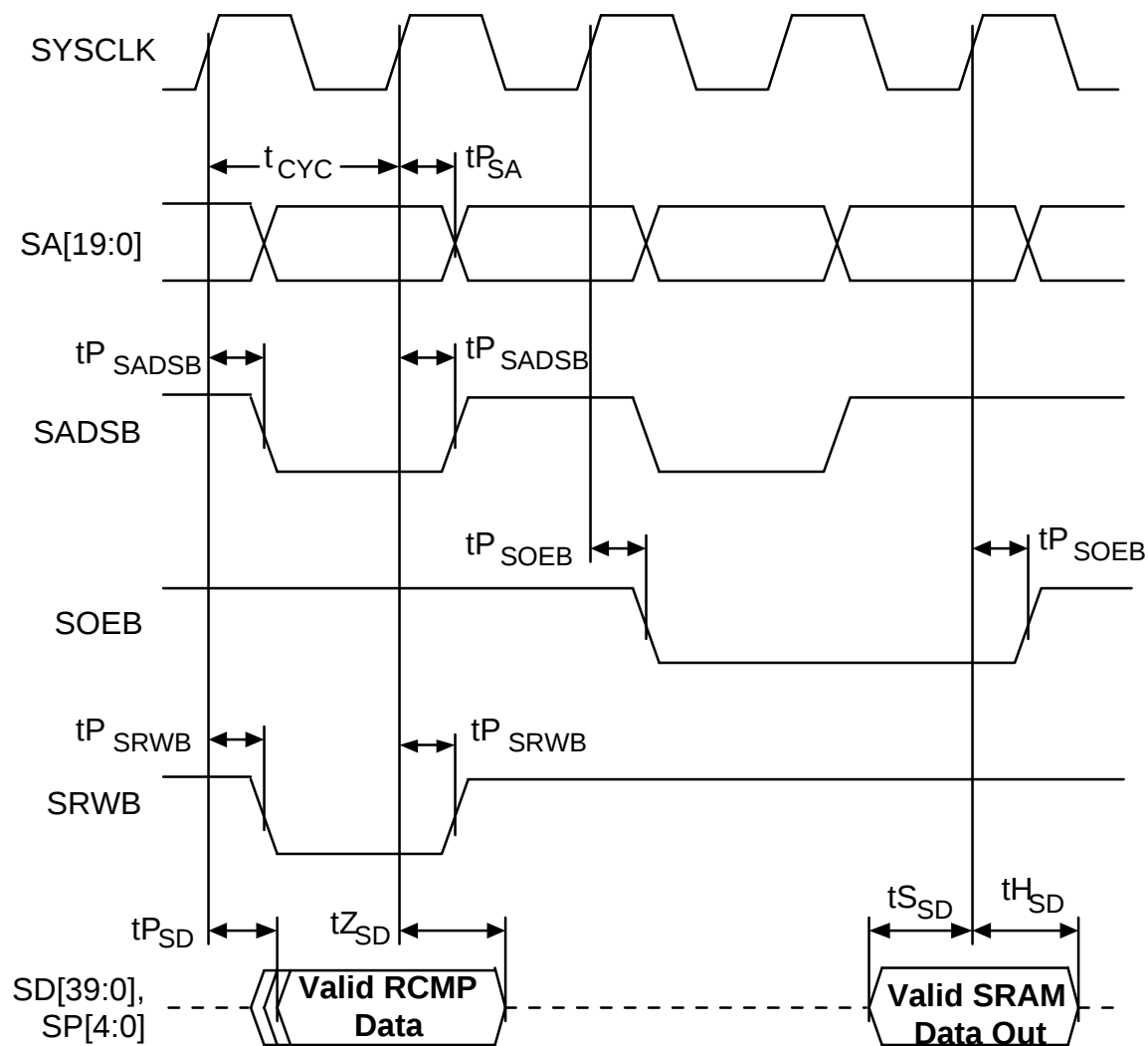
Fig. 20 Synchronous SRAM Interface Timing
