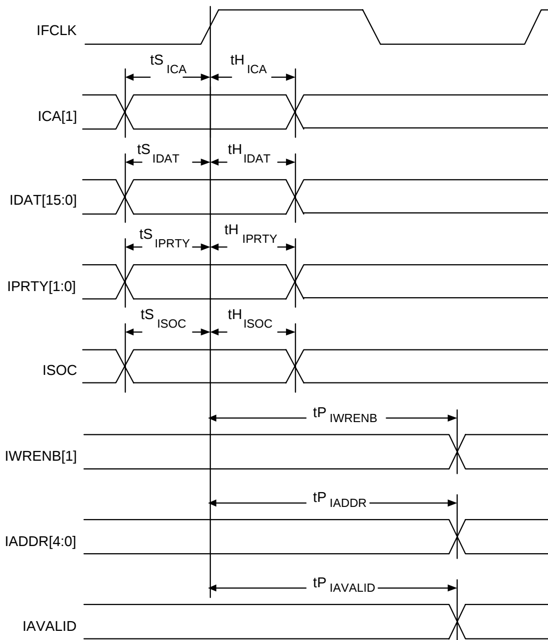
Fig. 18 Input Cell Interface Master (IPOLL=1) Timing
