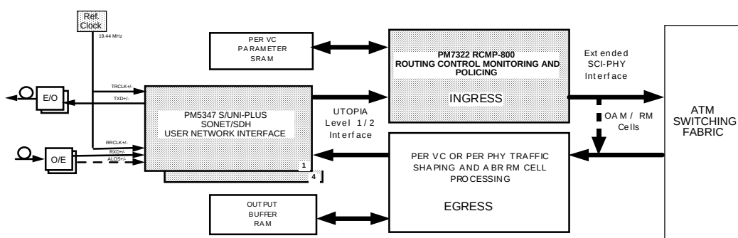
Fig. 1 OC-3 Switch Port Application
