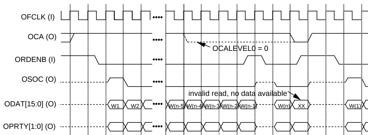
Fig. 14 Output Cell Interface Single-PHY Slave ( OTSEN=1)
