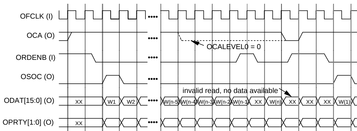
Fig. 13 Output Cell Interface Single-PHY Slave ( OTSEN=0)
