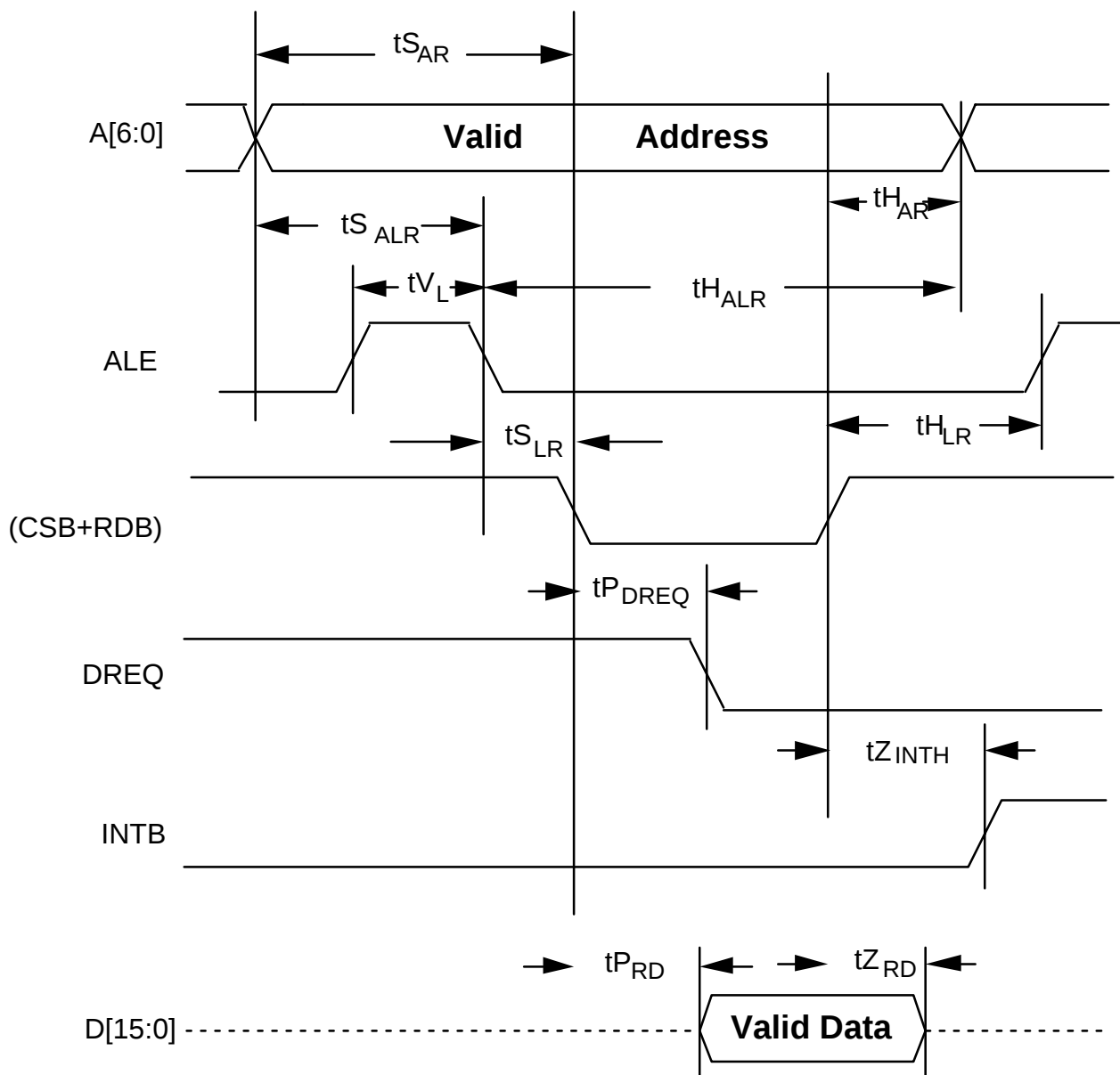
Fig. 15 Microprocessor Interface Read Timing
