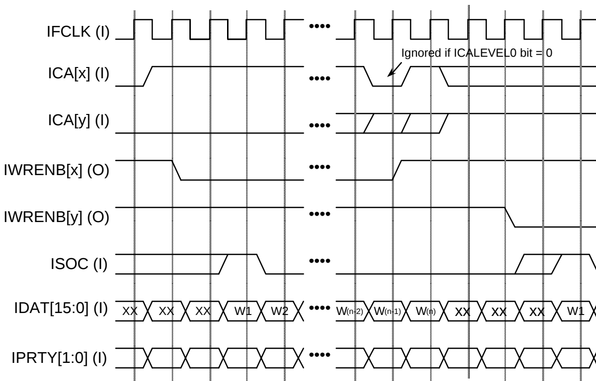
Fig. 10 Input Cell Master Interface (IPOLL=0)
