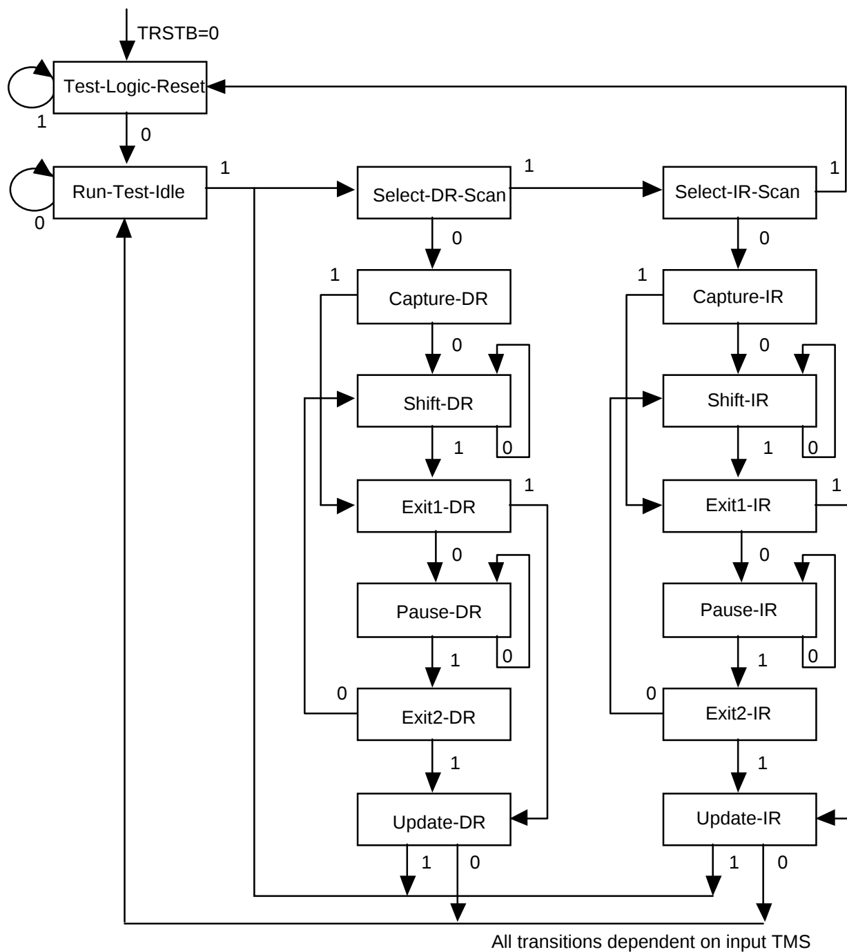
Fig. 9 TAP Controller Finite State Machine
