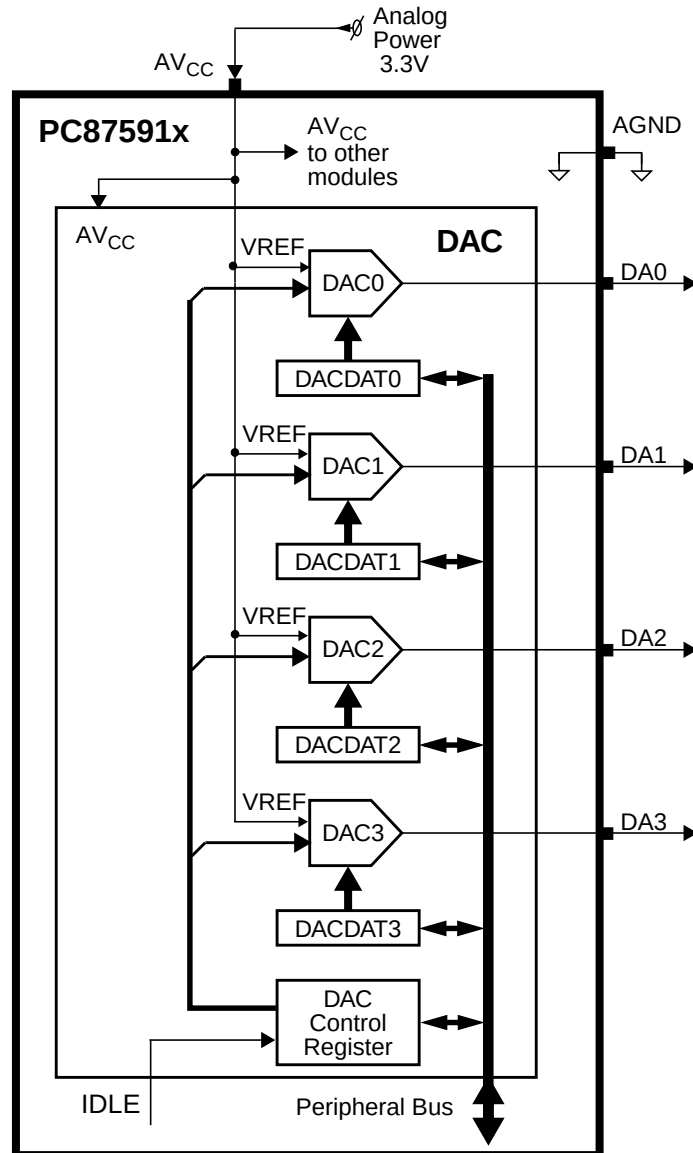
Figure 65. DAC Functional Diagram
