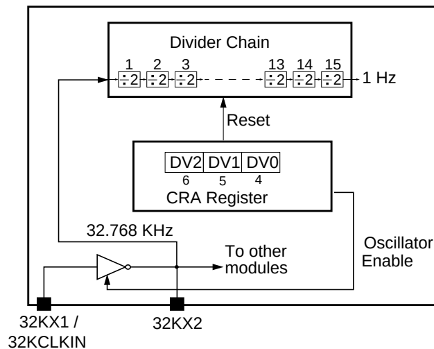
Figure 113. Divider Chain Control
