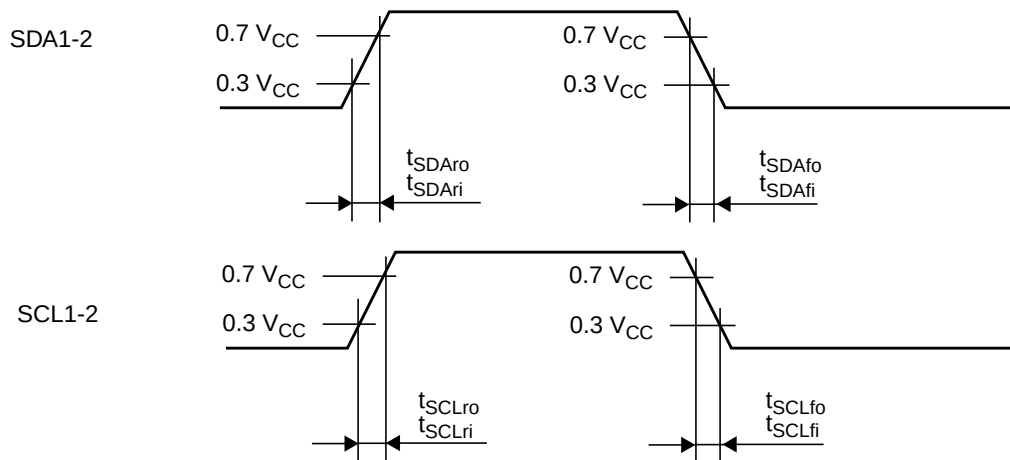
Figure 145. ACB Signals (SDA and SCL) Rising Time and Falling Time
