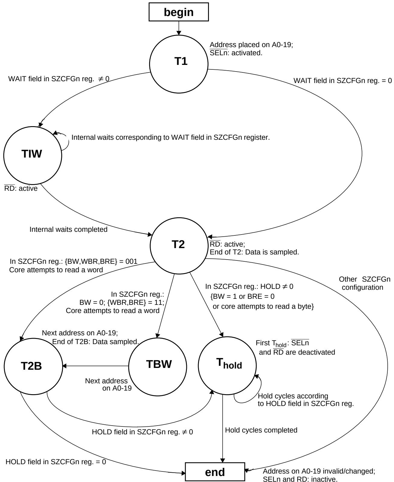
Figure 18. Normal Read Bus Cycle
