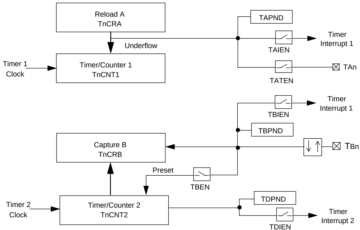
Figure 48. Mode 4, Input Capture and Timer
