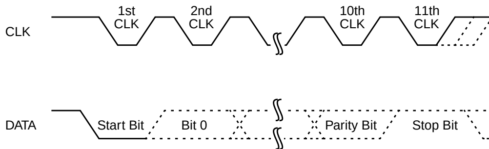
Figure 40. PS/2 Receive Data Byte Timing
