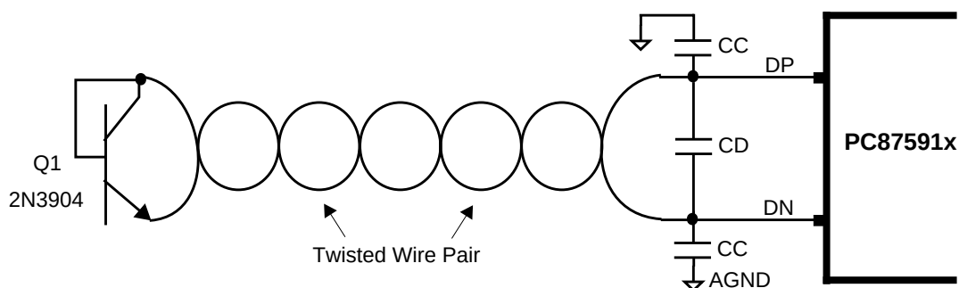
Figure 62. Typical Remote Diode Circuit (TBD)
