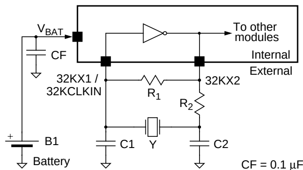
Figure 111. Recommended Oscillator External Circuitry
