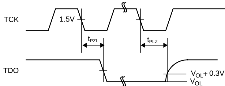
Figure 158. TDO TRI-STATE Output Low Enable and Disable Times
