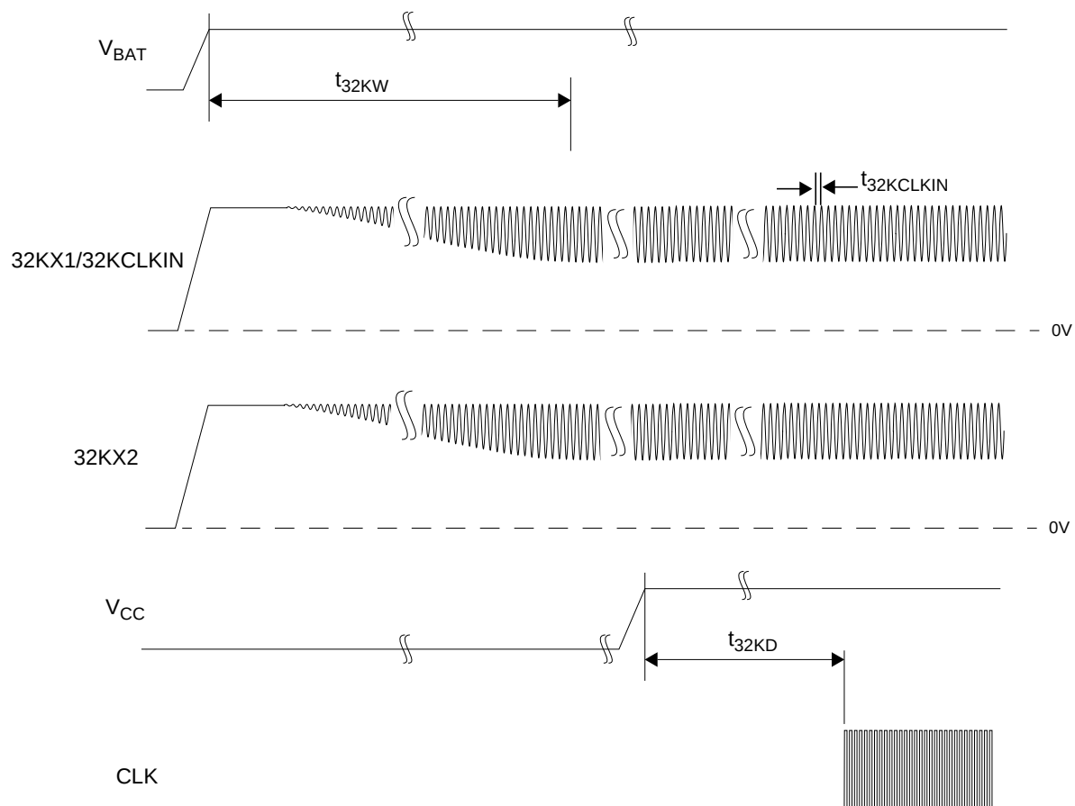
Figure 129. 32K Waveforms
