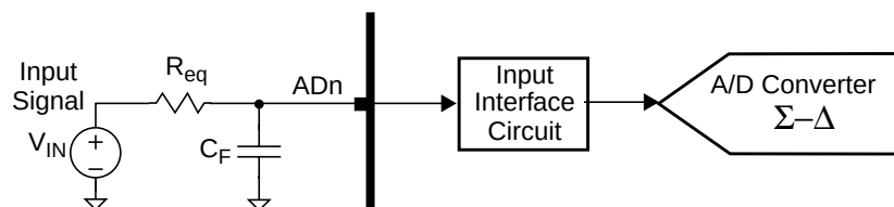
Figure 60. Filtered Voltage Input Equivalent Circuit
