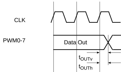
Figure 140. Output Signal Timing for PWM Signals
