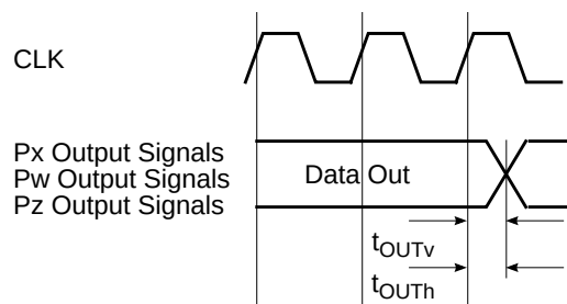
Figure 139. Output Signal Timing for Output and I/O Port Signals
