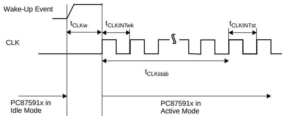
Figure 131. Internal Clock Generator
