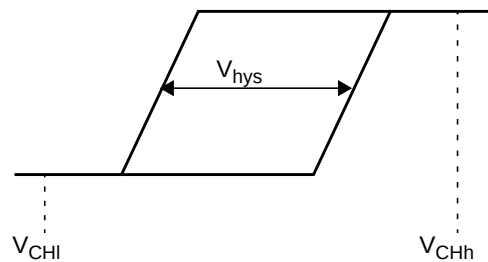
Figure 125. CMOS with Hysteresis Inputs
