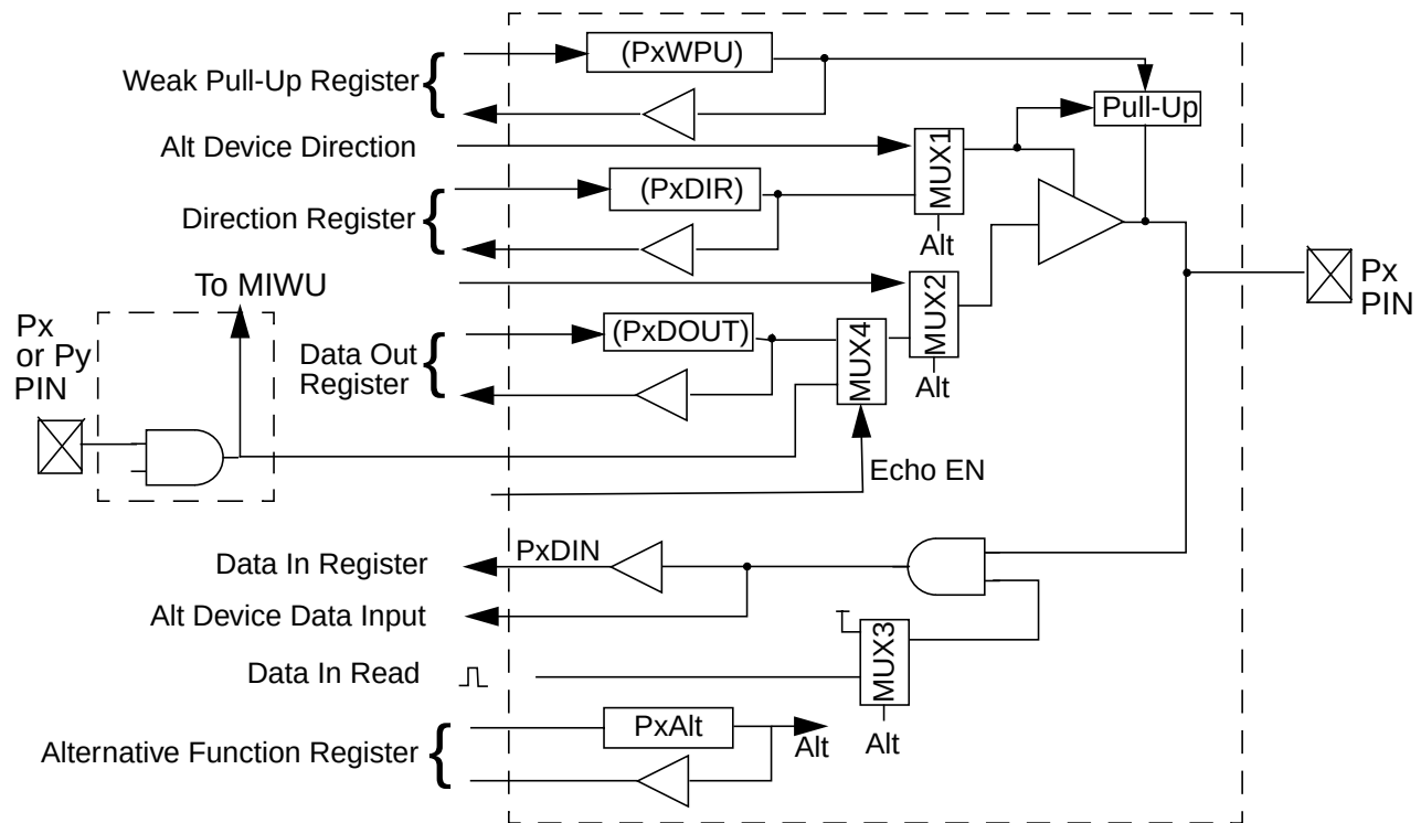
Figure 32. GPIO Port Px Output with Echo Schematic Diagram
