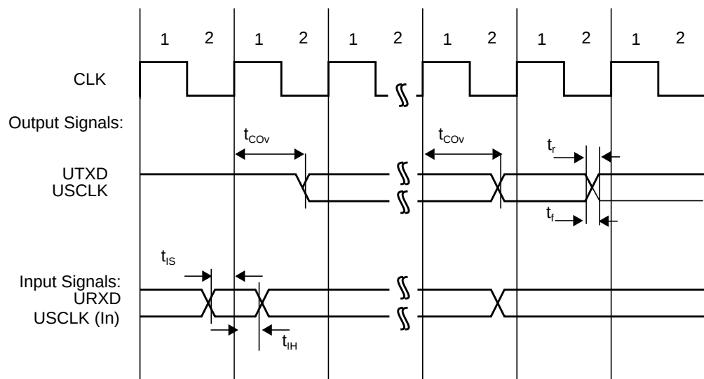
Figure 160. USART Asynchronous Mode Timing
