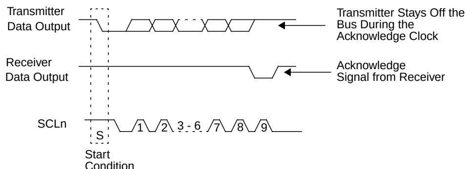
Figure 70. ACCESS.bus Acknowledge Cycle
