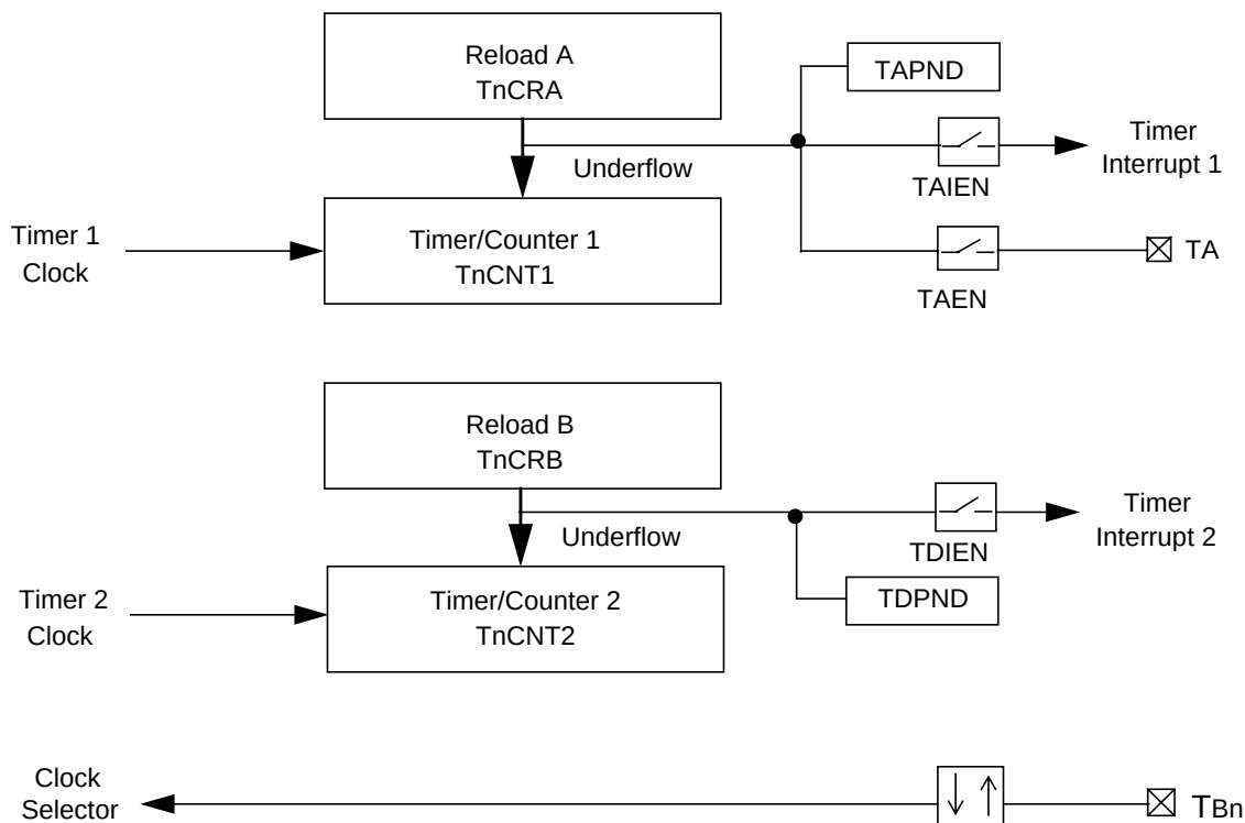
Figure 47. Mode 3, Dual Independent Timer
