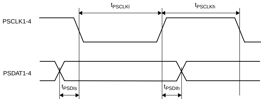
Figure 142. PS/2 Receive Timing
