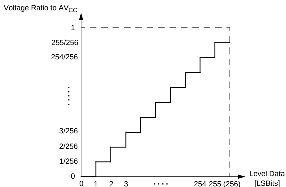
Figure 64. Channel Data to Output Voltage Ratio Conversion
