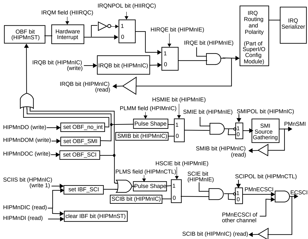
Figure 96. IRQ, SCI and SMI Control, Enhanced PM Mode
