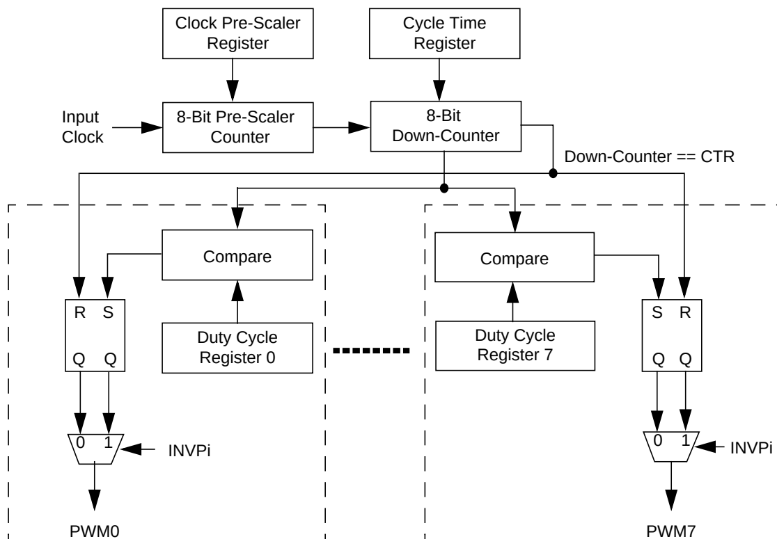
Figure 49. PWM Block Diagram
