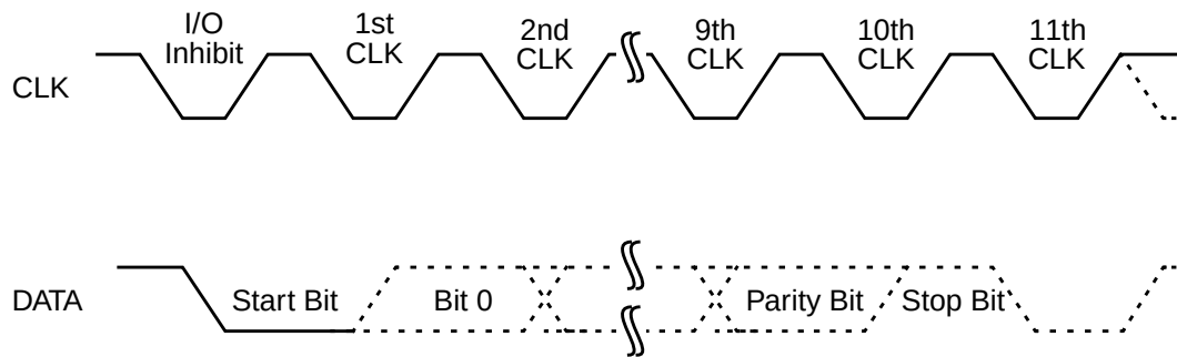
Figure 41. PS/2 Transmit Data Byte Timing
