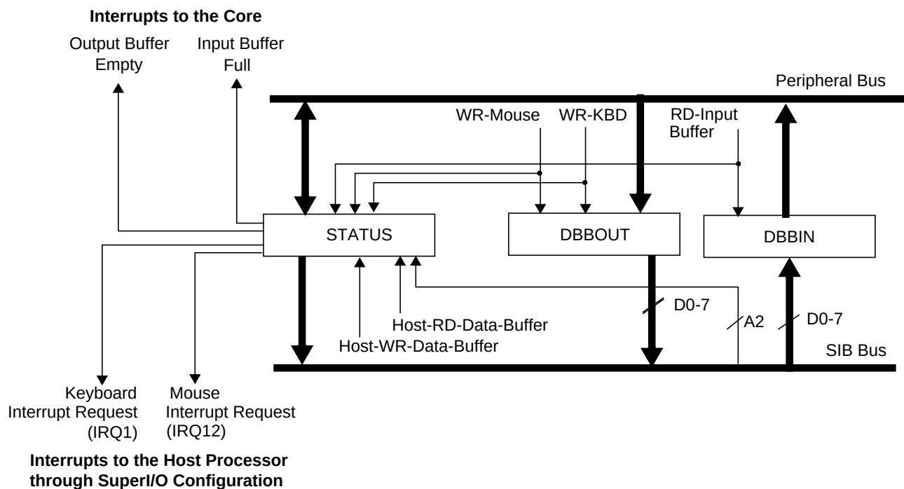
Figure 92. Host Interface Keyboard/Mouse Channel (Ports 60,64) Block Diagram
