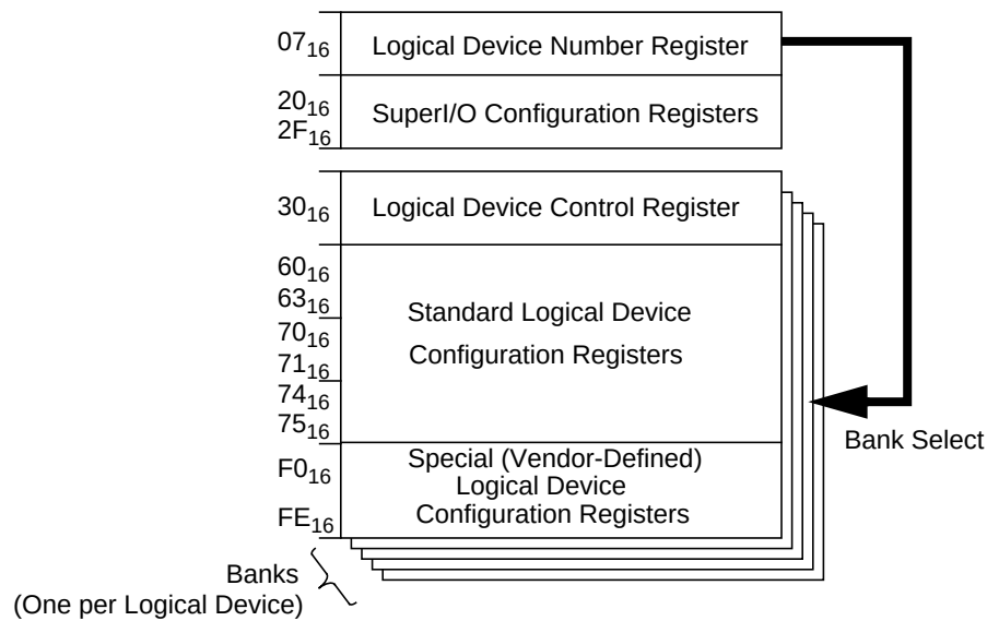
Figure 107. Structure of Standard Configuration Register File
