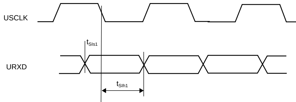
Figure 163. USART Synchronous Mode Timing (USCLK)
