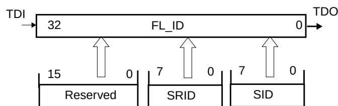
Figure 86. Flash Identification Register
