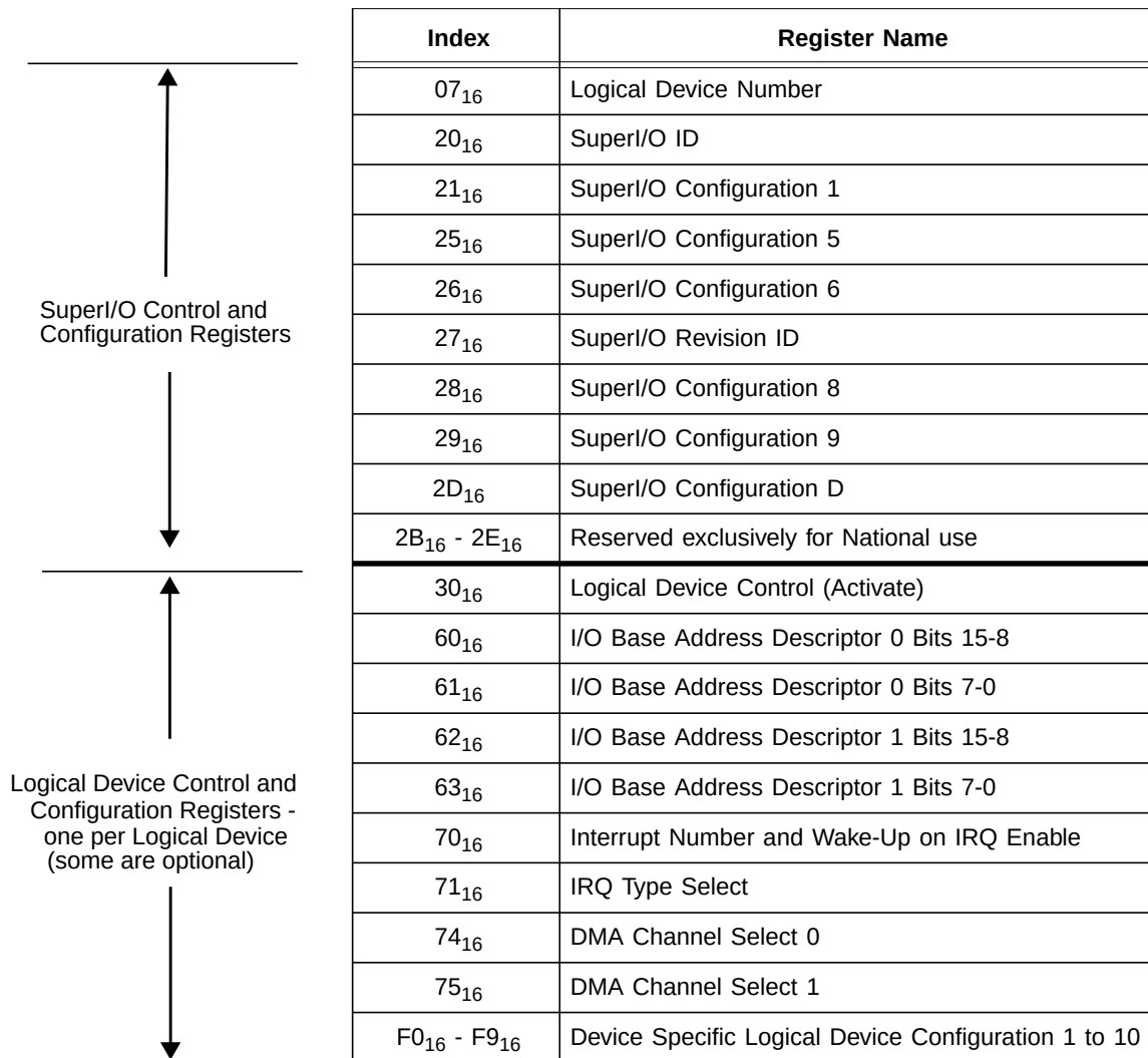
Figure 108. Configuration Register Map
