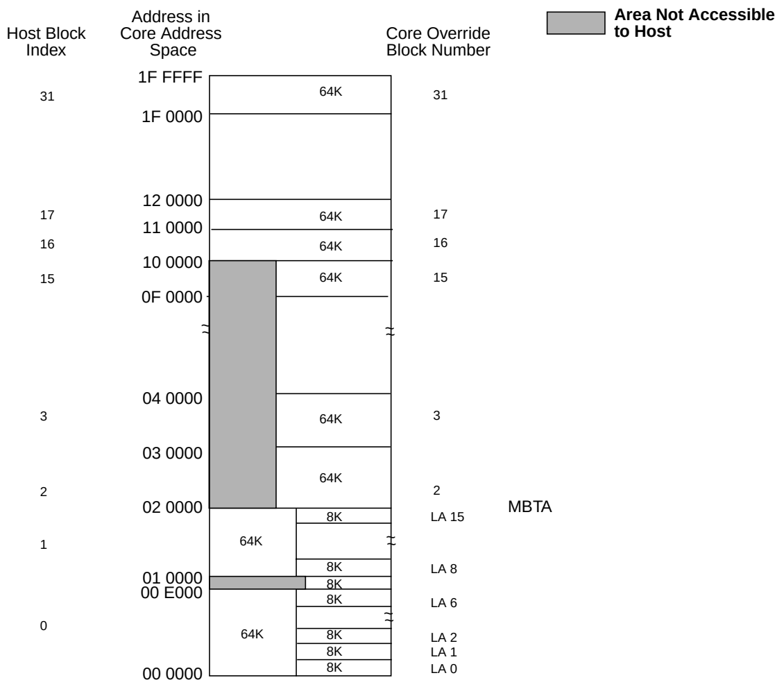
Figure 100. Protection Blocks for Protection Bits and Override Protection Bits
