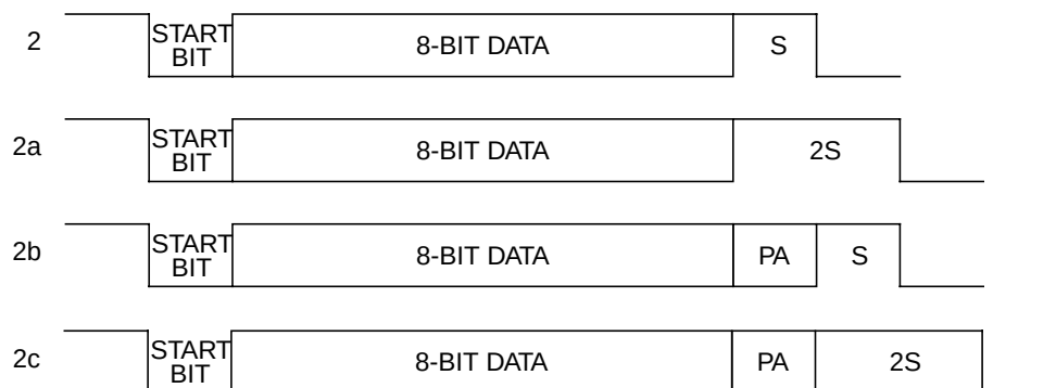
Figure 54. Eight Data Bit Frame Options
