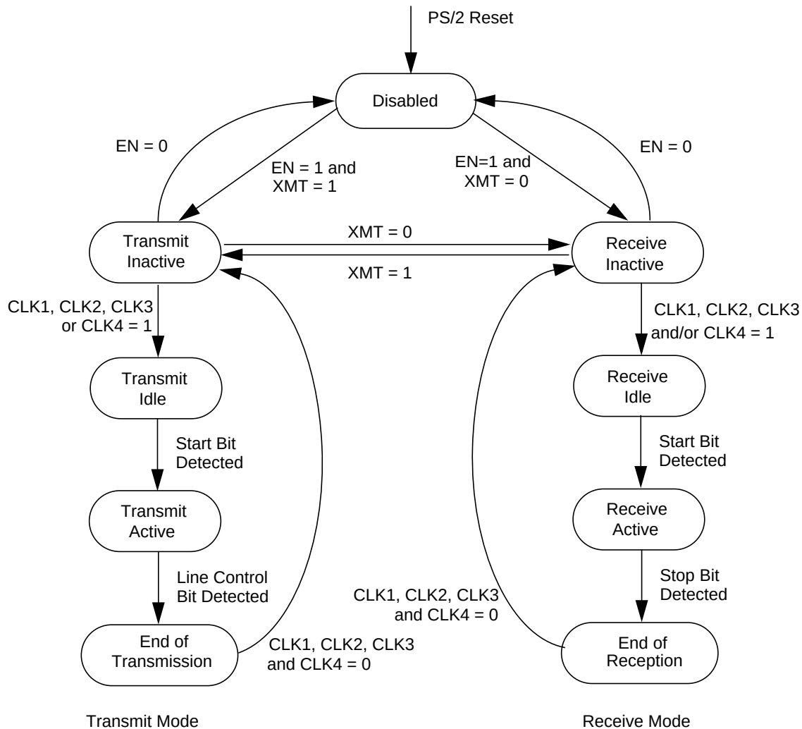
Figure 39. Shift Mechanism State Diagram
