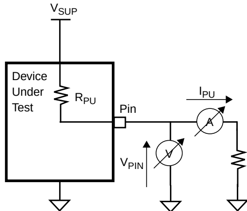
Figure 121. Internal Resistor Test Conditions, T_A = 0^{\circ}\text{C} to 70^{\circ}\text{C} , V_{SUP} = 3.3\text{V}
