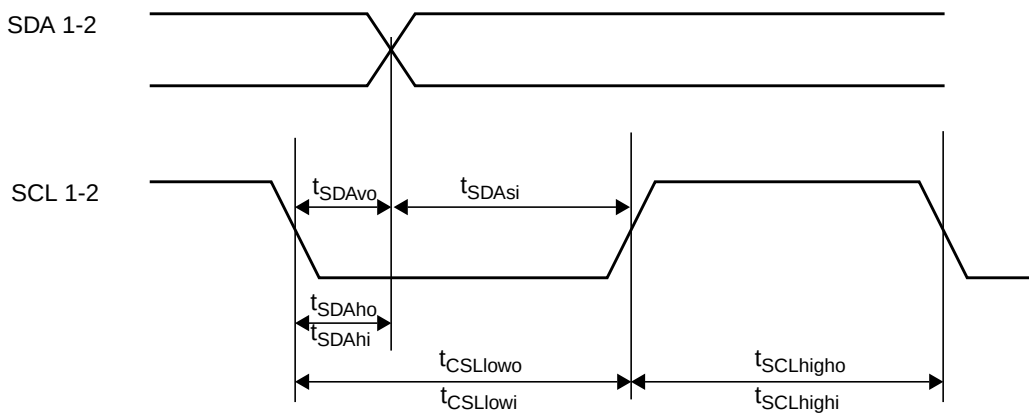
Figure 148. ACB Data Bit Timing
