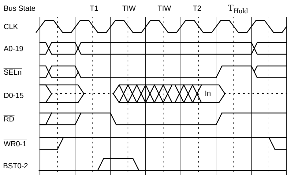
Figure 17. Normal Read Bus Cycle with 2 Internal Waits and 1 Hold
