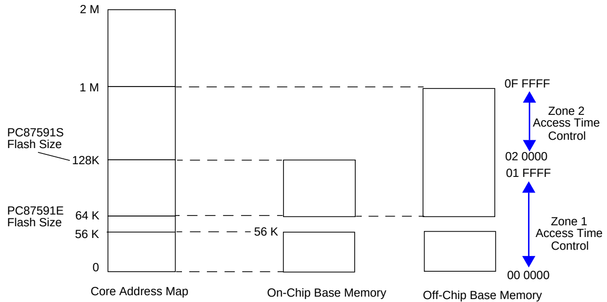
Figure 6. Base Memory Address Mapping
