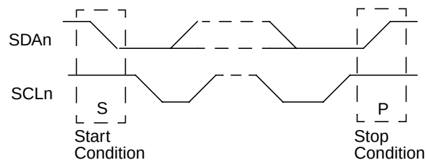
Figure 68. Start and Stop Conditions
