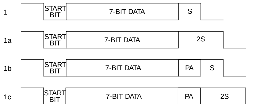
Figure 53. Seven Data Bit Frame Options
