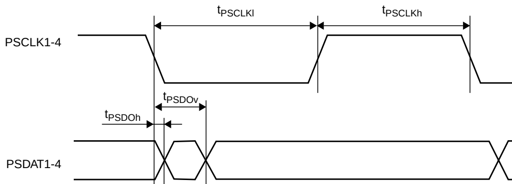
Figure 143. PS/2 Transmit Timing
