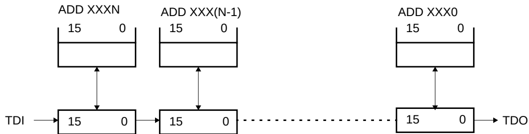
Figure 82. Bit Allocation Arrangement
