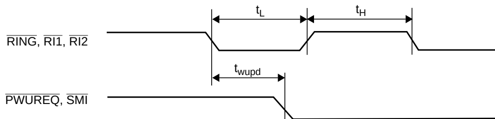
Figure 141. Wake-Up Timing
