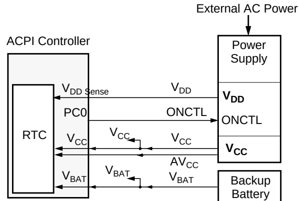
Figure 114. Power Supply Connections
