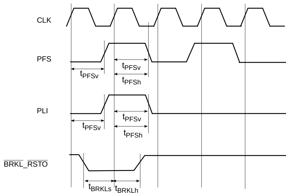
Figure 151. Pipe Status Signal (PFS and PLI) Timing
