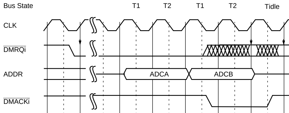
Figure 26. Indirect Bus Cycle (DIR=0) - External Access
