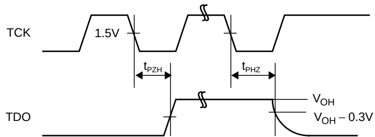
Figure 157. TDO TRI-STATE Output High Enable and Disable Times
