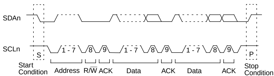
Figure 71. A Complete ACCESS.bus Data Transaction
