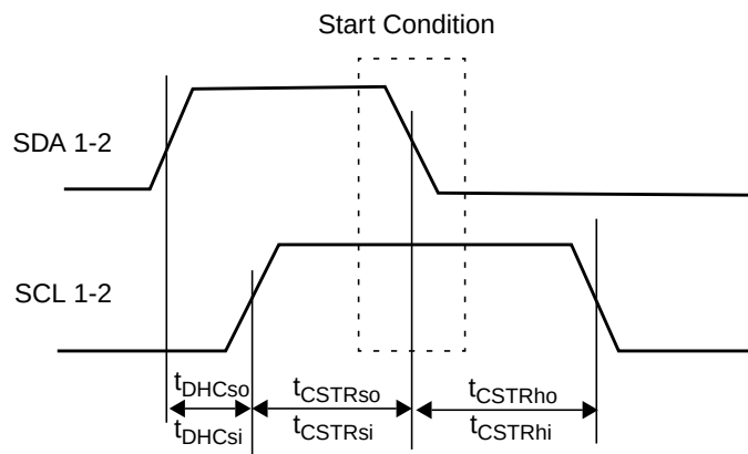
Figure 147. ACB Start Condition Timing
