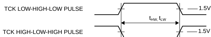
Figure 155. TCK Pulse Width
