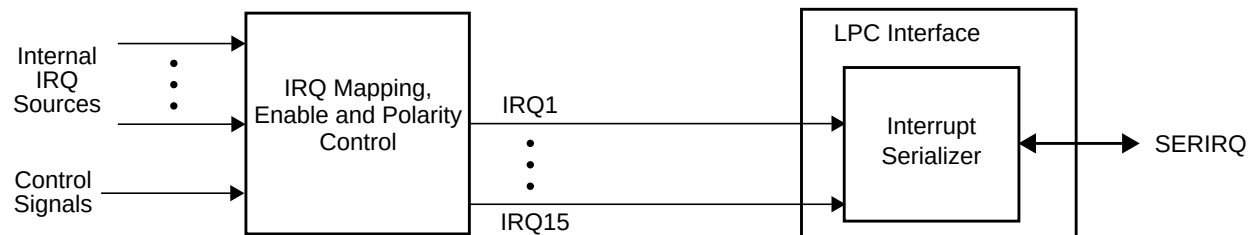
Figure 109. Interrupt Serialization Mechanism
