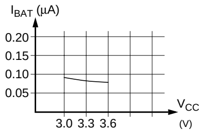
Figure 118. Typical Battery Current During Normal Operation Mode
