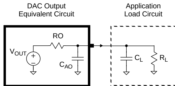
Figure 66. DAC Output Equivalent Circuit
