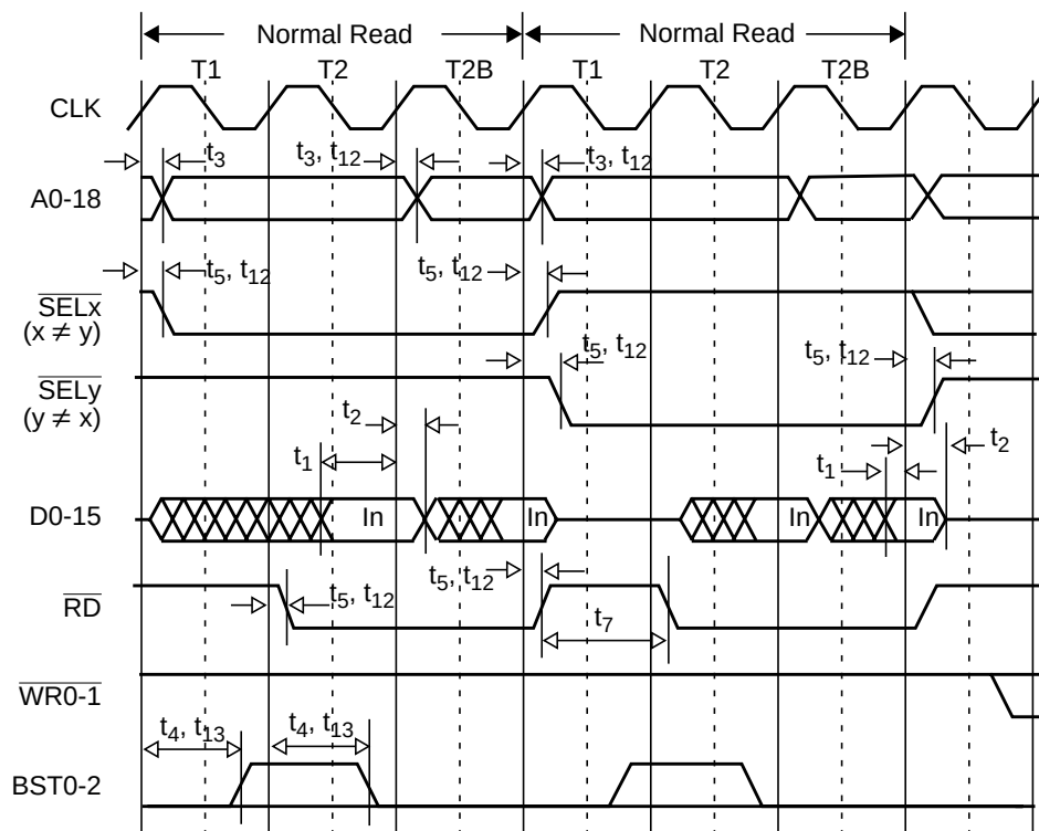
Figure 134. Two Consecutive Normal Read Bus Cycles with Burst, 0 Wait, AC Timing
