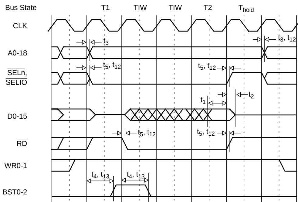
Figure 135. Normal Read Bus Cycle (2 Internal Waits, and 1 Hold), AC Timing
