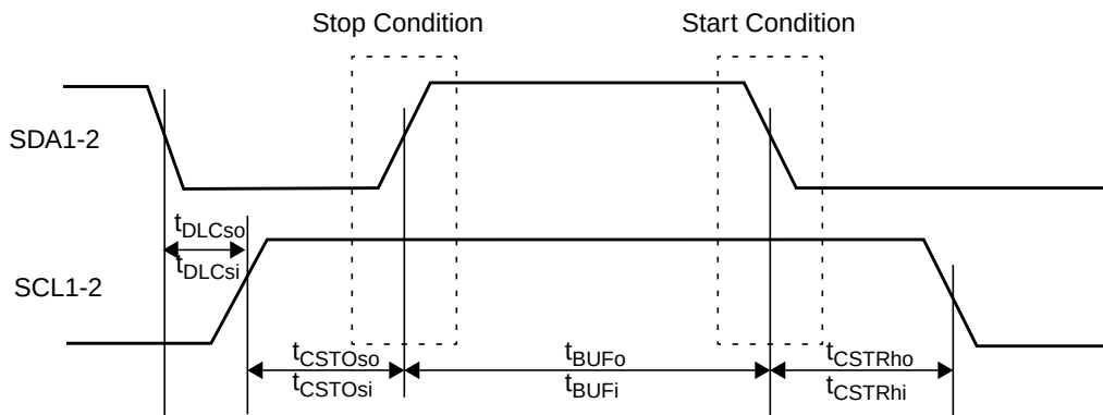
Figure 146. ACB Start and Stop Condition Timing
