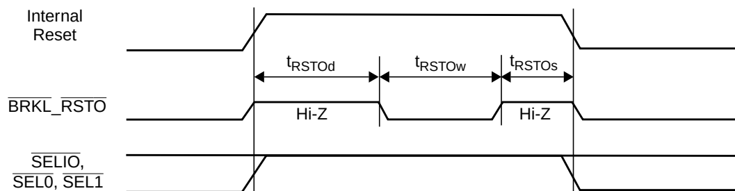
Figure 152. Reset Out Signal Timing
