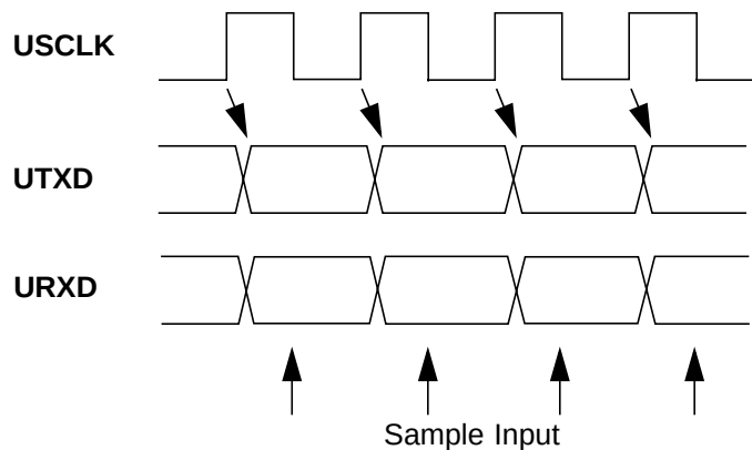
Figure 52. USART Synchronous Communication
