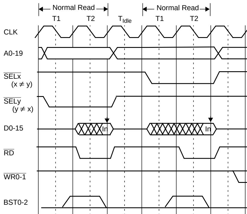
Figure 16. Two Basic Normal Read Bus Cycles with Idle in between (IPST Bit in SZCFGy Register = 1, IPRE Bit in SZCFGx Register = 1)
