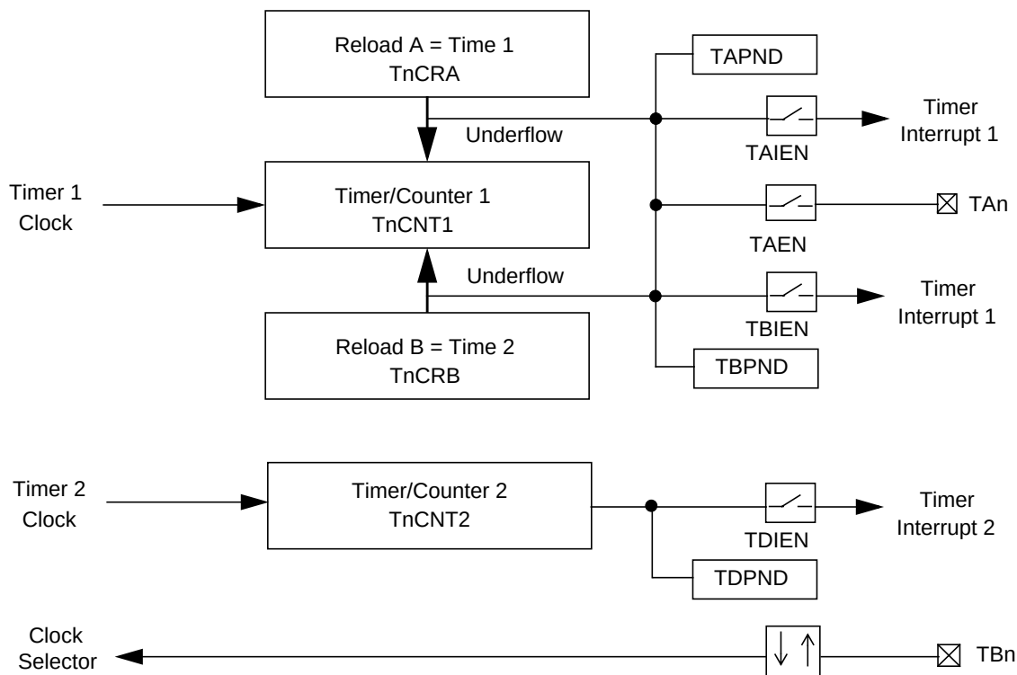
Figure 45. Mode 1, PWM and Counter
