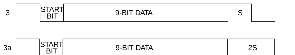
Figure 55. Nine Data Bit Frame Options
