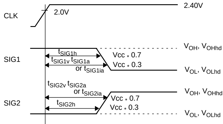
Figure 123. CMOS Output Signals Specification Conventions
