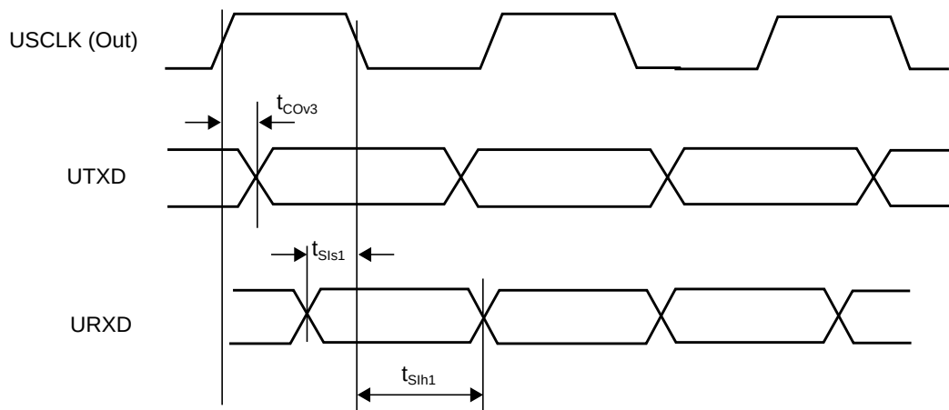
Figure 162. USART Synchronous Mode Timing (USCLK Out)
