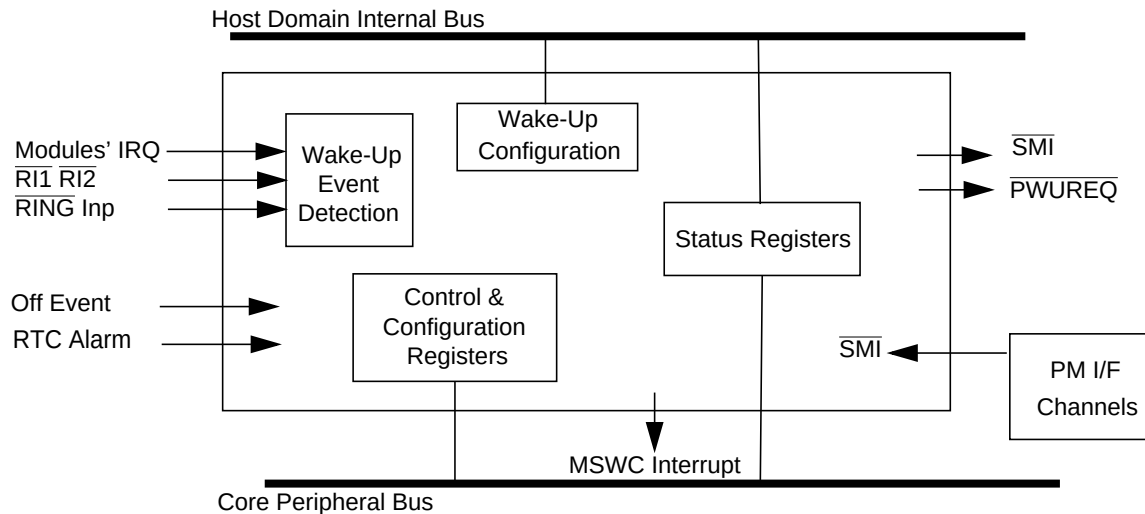
Figure 102. MSWC Block Diagram
