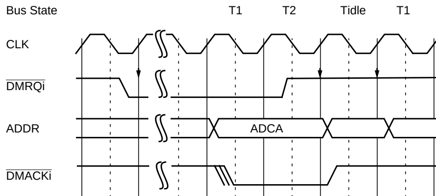
Figure 25. DMAC Direct Bus Cycle Followed by a Core Bus Cycle
