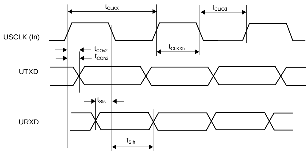
Figure 161. USART Synchronous Mode Timing (USCLK Input)
