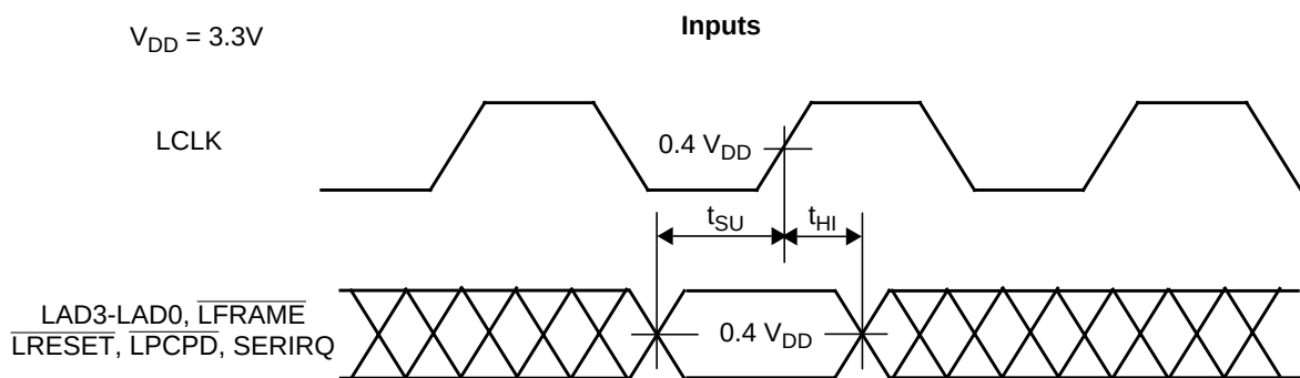
Figure 166. LPC/SERIRQ Interface Input Timing
