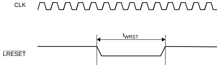
Figure 128. Warm Hardware Reset
