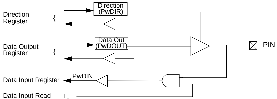
Figure 35. GPIO Port Pw Schematic Diagram
