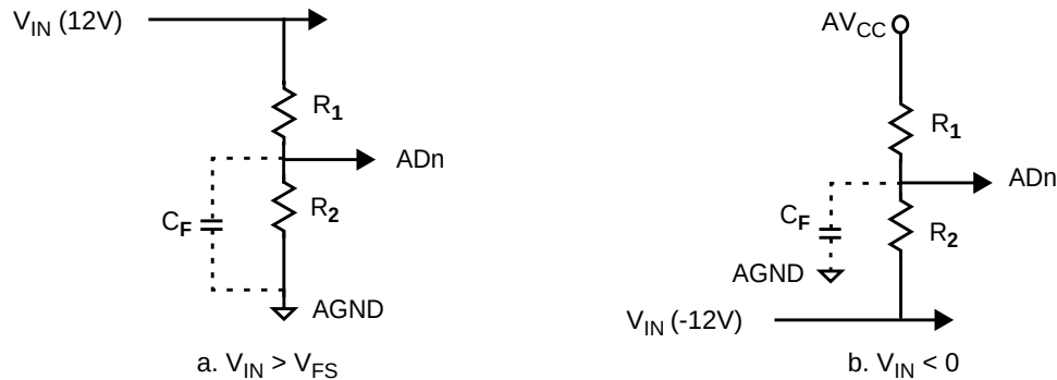
Figure 59. Measurement of Positive and Negative Voltages
