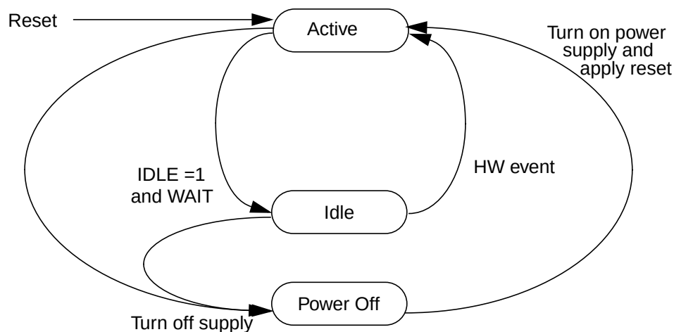
Figure 75. Power Modes and Transitions
