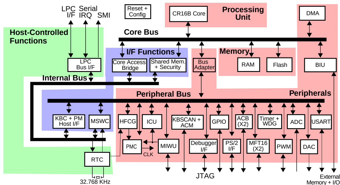
Figure 2. PC87591x Functional Block Diagram
