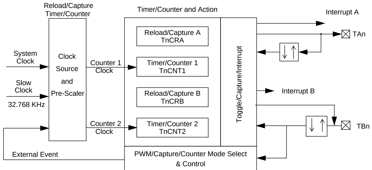
Figure 42. MFT16 Functional Diagram
