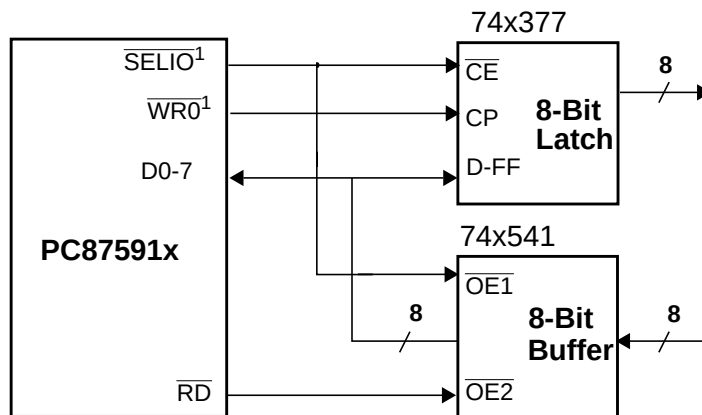
Figure 23. Example of an Implementation of Two Ports Using I/O Expansion
