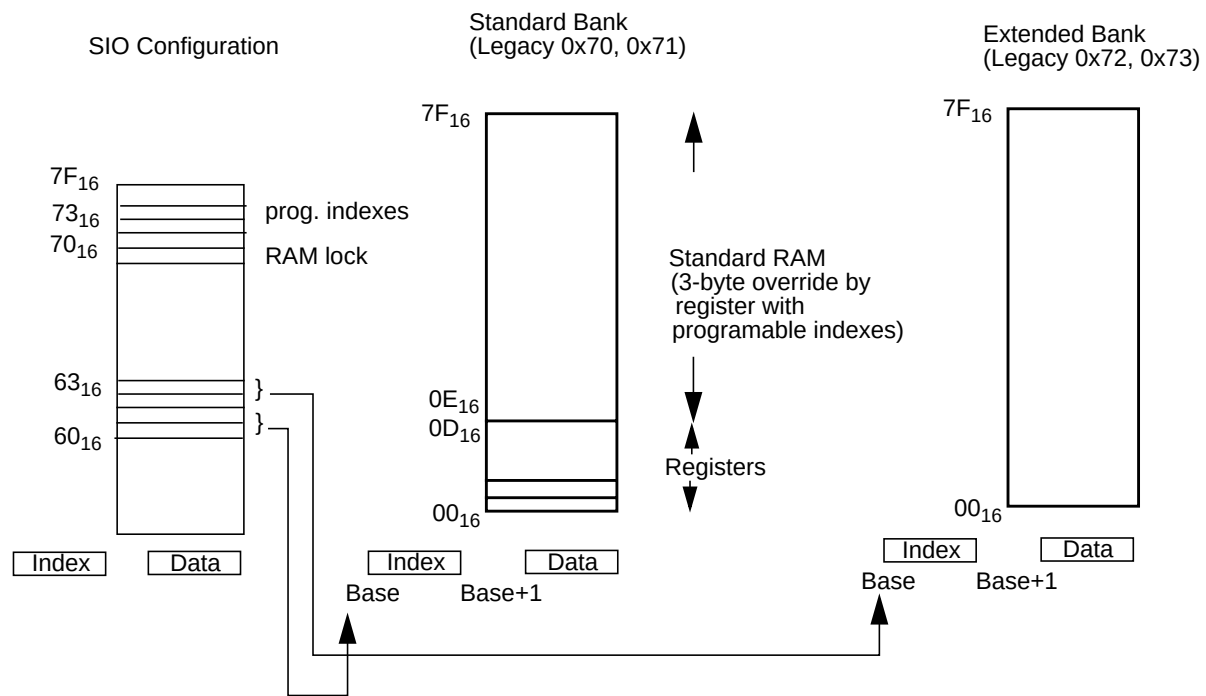
Figure 120. RTC Module Registers Mapping
