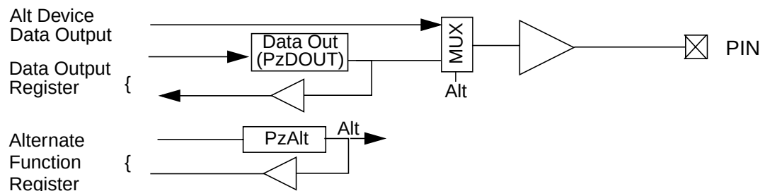
Figure 34. GPO Port Pz Schematic Diagram
