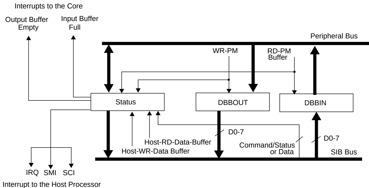
Figure 93. Host Interface PM Channel n Block Diagram
