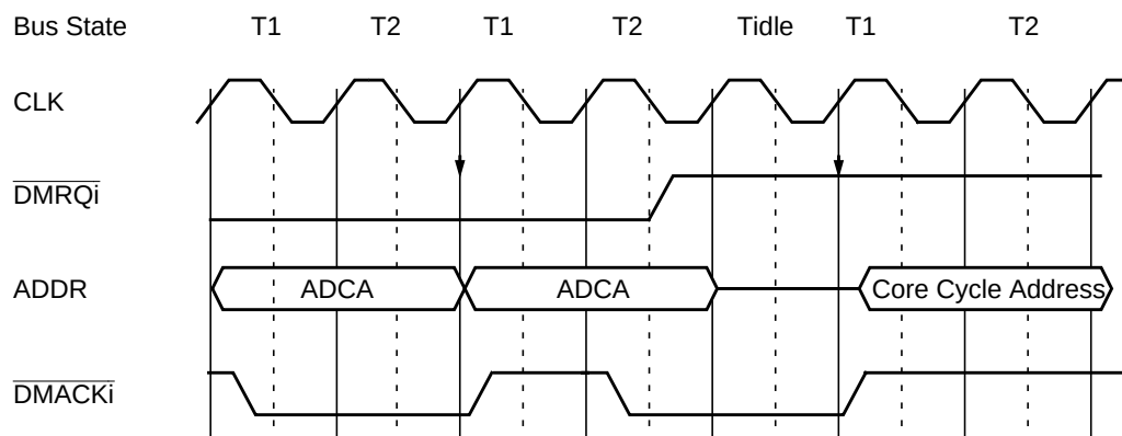
Figure 29. DMAC Direct Bus Cycles in Continuous Mode - External Bus
