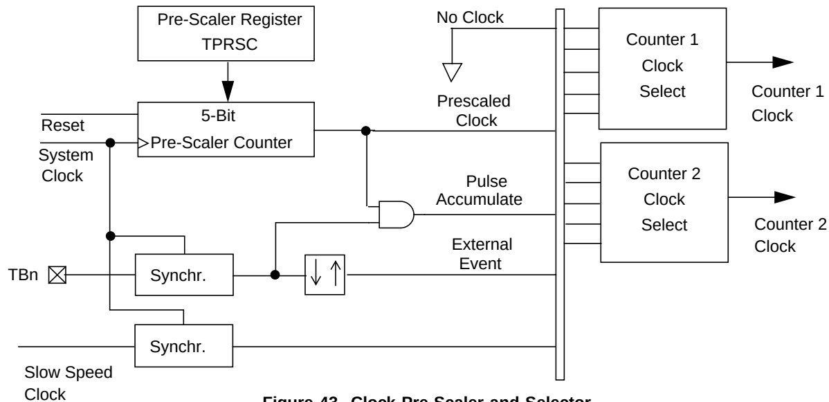
Figure 43. Clock Pre-Scaler and Selector
