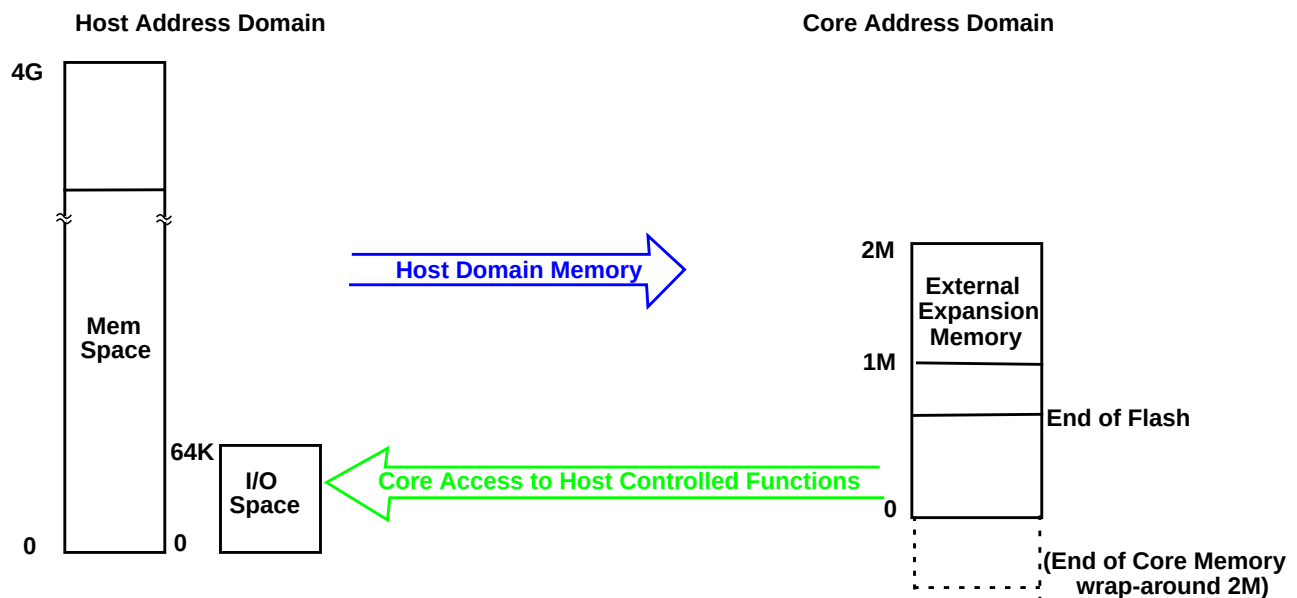
Figure 5. PC87591x Memory Domains
