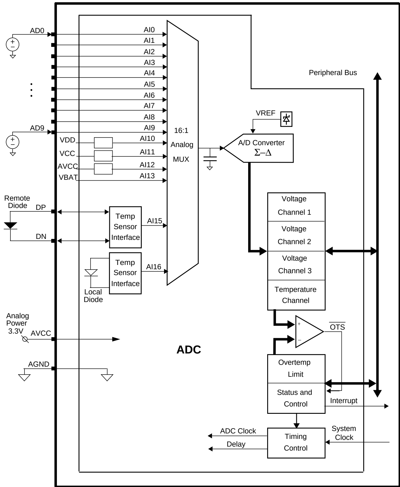
Figure 58. ADC Functional Diagram
