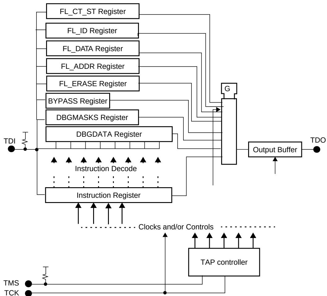
Figure 79. TAP Block Diagram
