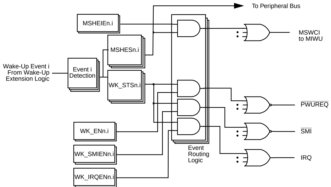
Figure 103. Wake-Up Event Routing Scheme
