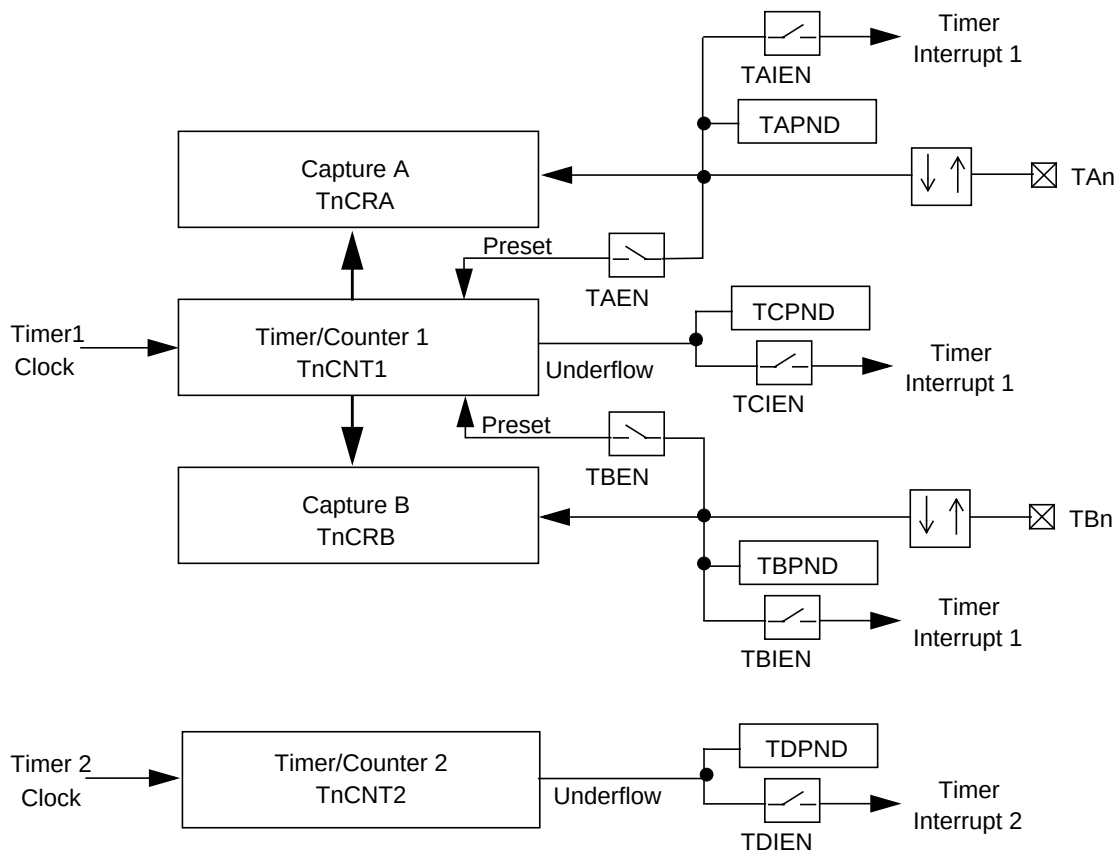
Figure 46. Mode 2, Dual Input Capture
