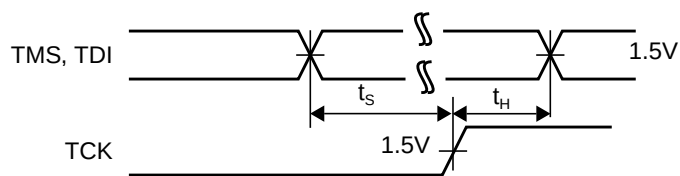
Figure 154. Debugger I/F Setup Time, Hold Time and Recovery Time
