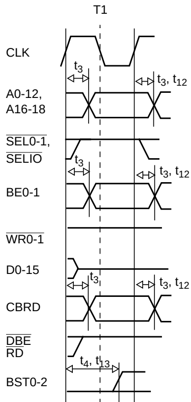
Figure 137. Core Bus Monitoring Bus Cycle, AC Timing
