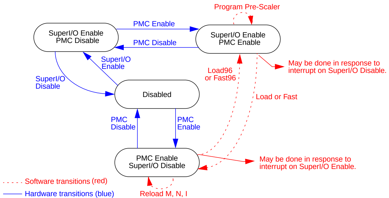
Figure 77. HFCG States and Transitions
