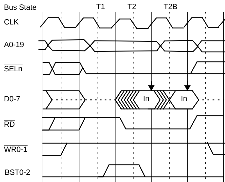
Figure 19. Normal Read Bus Cycle with 0 Wait on Burst
