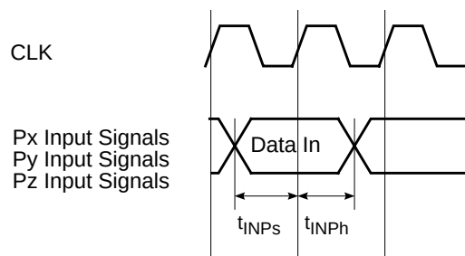
Figure 138. Input Signal Timing for Input and I/O Port Signals
