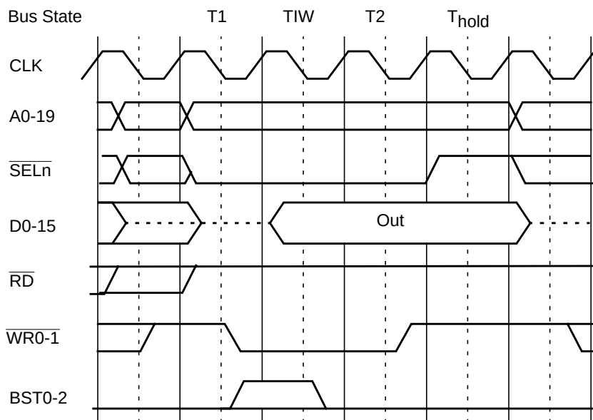
Figure 15. Late Write Bus Cycle with 1 Internal Wait and 1 Hold
