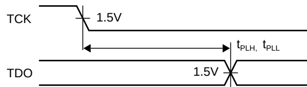
Figure 156. Debugger Interface Propagation Delay
