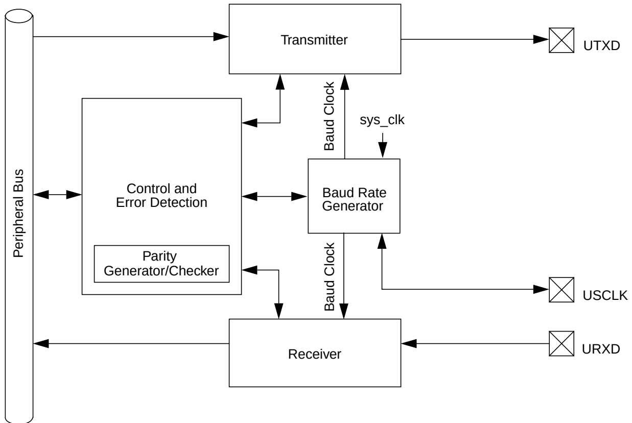
Figure 50. USART Block Diagram
