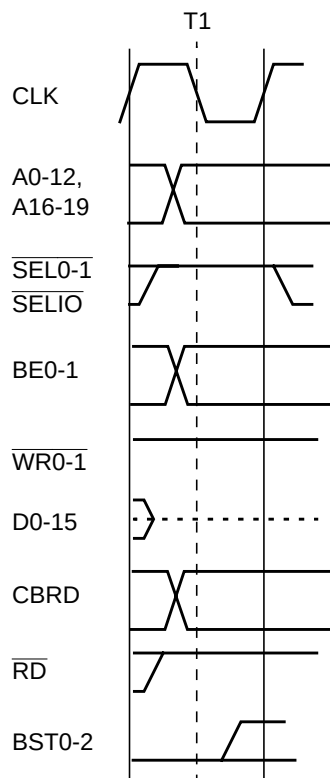
Figure 24. Core Bus Monitoring Bus Cycle
