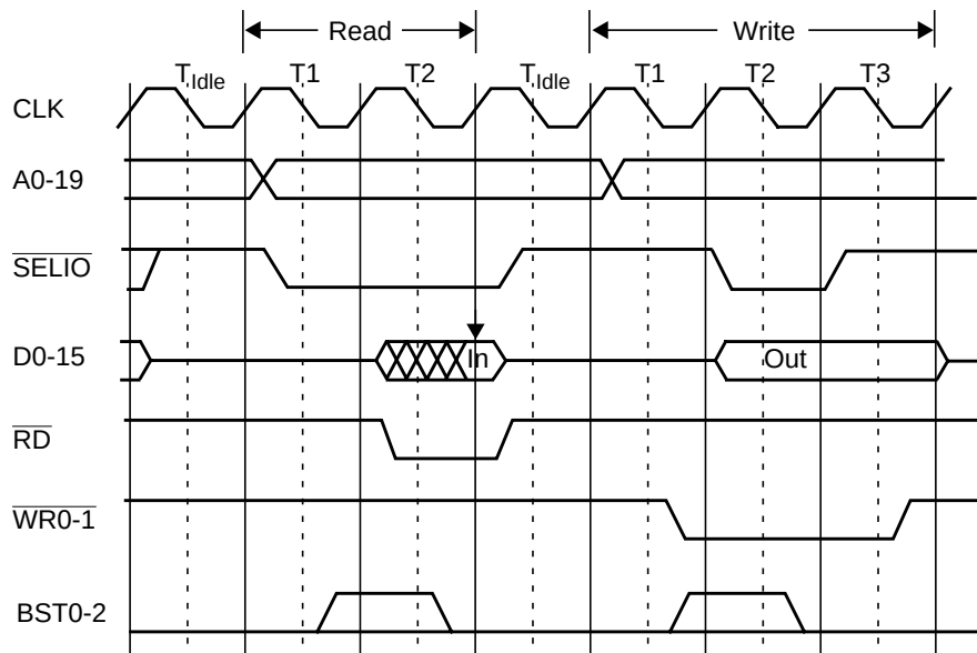
Figure 22. I/O Expansion Bus Cycles (EWR bit in BCFG Register = 1)
