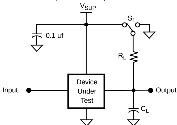
Figure 122. AC Test Conditions, T_A = 0^\circ\text{C} to 70^\circ\text{C} , V_{SUP} = 3.3\text{V} \pm 10\%
