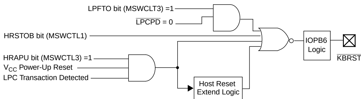
Figure 105. \overline{\text{KBRST}} Generation Scheme
