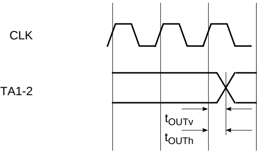
Figure 150. Multi-Function Timer (MFT16) Output Timing
