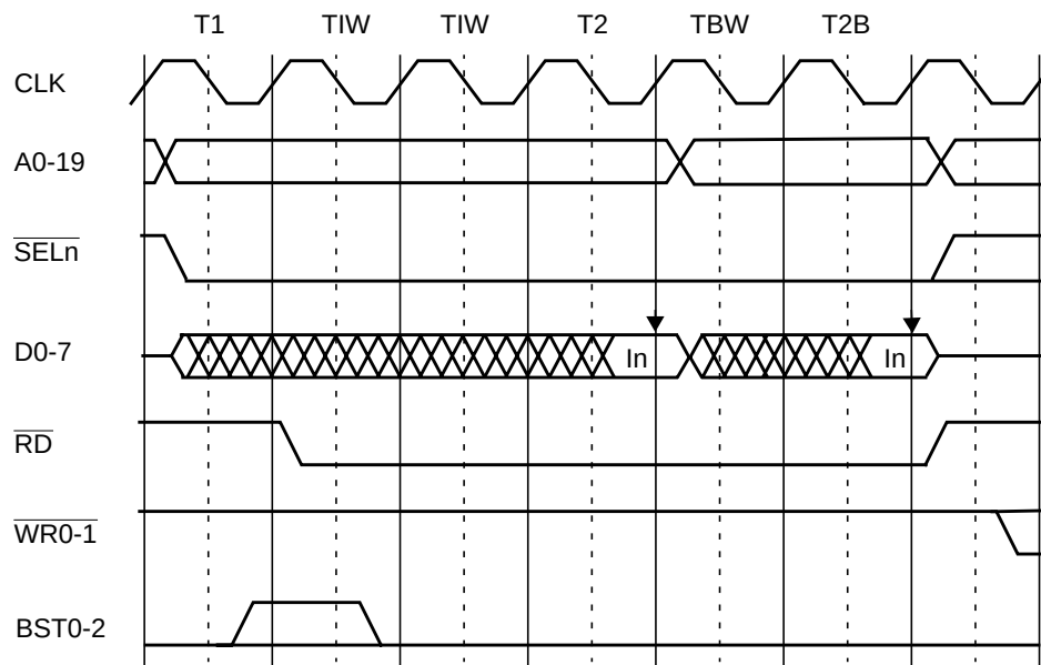
Figure 20. Normal Read Bus Cycle with 2 Internal Waits and 1 Wait on Burst
