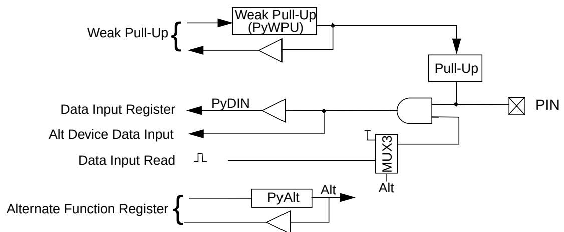
Figure 33. GPI Port Py Schematic Diagram
