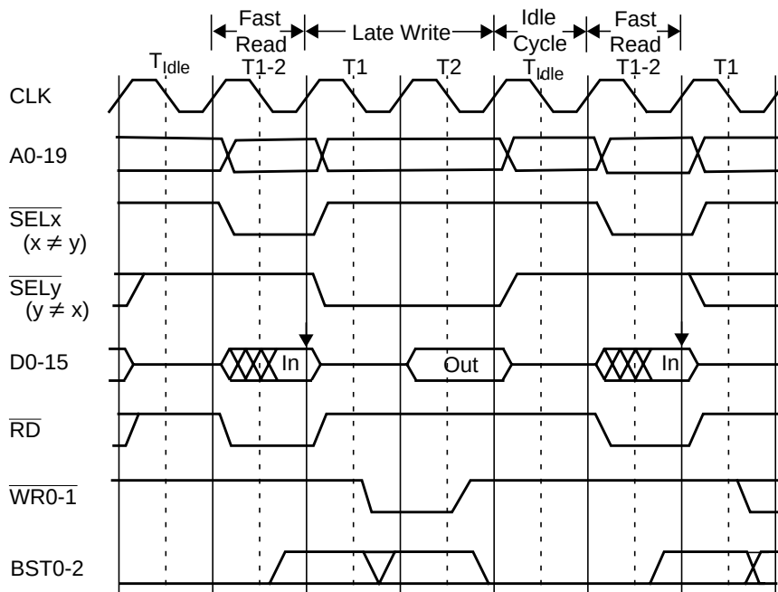
Figure 21. Fast Read Bus Cycle
