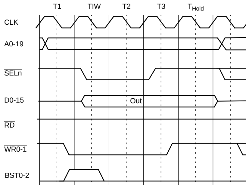
Figure 12. Early Write Bus Cycle with 1 Internal Wait and 1 Hold
