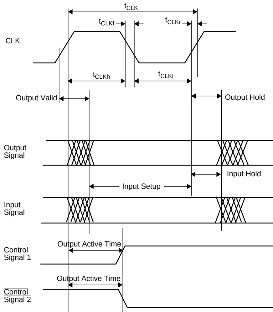
Figure 130. Clock Waveforms
