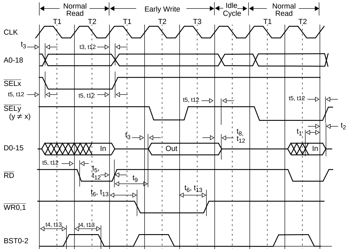
Figure 132. Early Write Between Normal Read Bus Cycles
