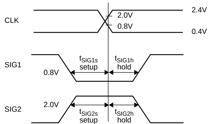
Figure 124. TTL: Input Signal Specification Standard
