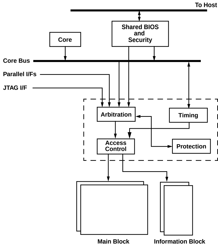
Figure 74. On-Chip Flash Block Diagram
