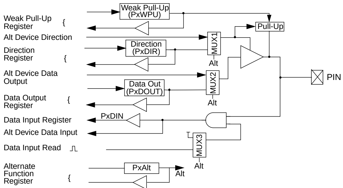
Figure 31. GPIO Port Px Schematic Diagram
