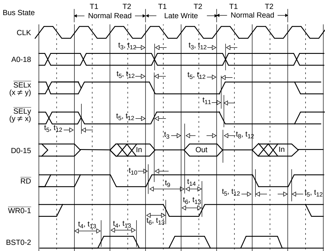
Figure 133. Late Write between Two Normal Read Bus Cycles, 0 Wait, AC Timing
