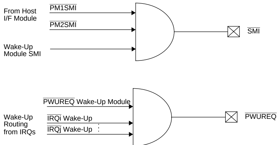
Figure 104. \overline{\text{SMI}} and \overline{\text{PWUREQ}} Source Gathering Scheme
