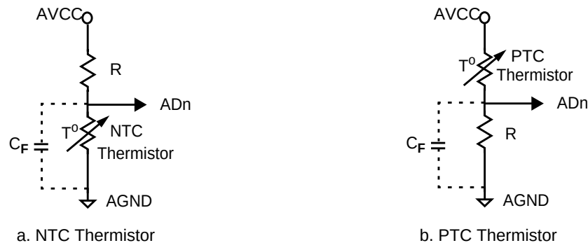
Figure 61. Measuring Temperature Using Thermistors
