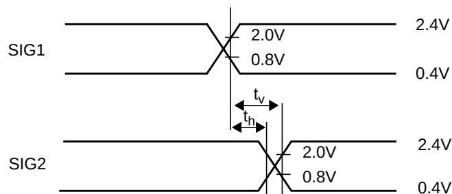
Figure 126. Signal to Signal Delay
