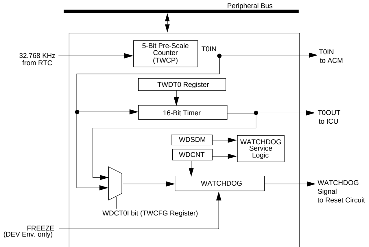
Figure 57. Timer and WATCHDOG Block Diagram
