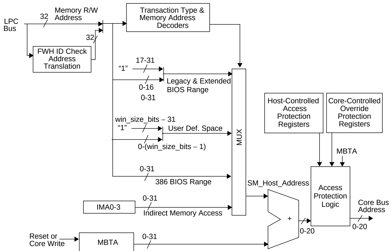
Figure 97. Address Translation Mechanism for 512 Kbyte On-Chip Flash
