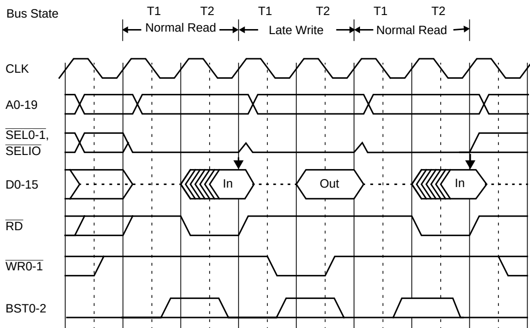
Figure 14. Late Write Bus Cycle Between Normal Read Bus Cycles with 0 Wait
