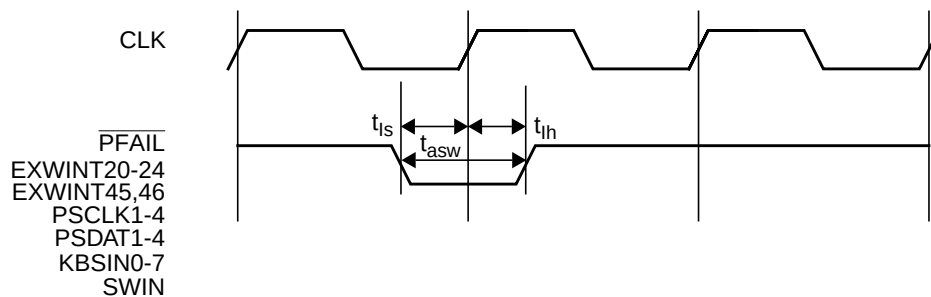
Figure 153. \overline{ISE} , \overline{PFAIL} , EXINTn and MIWU Input Signal Timing
