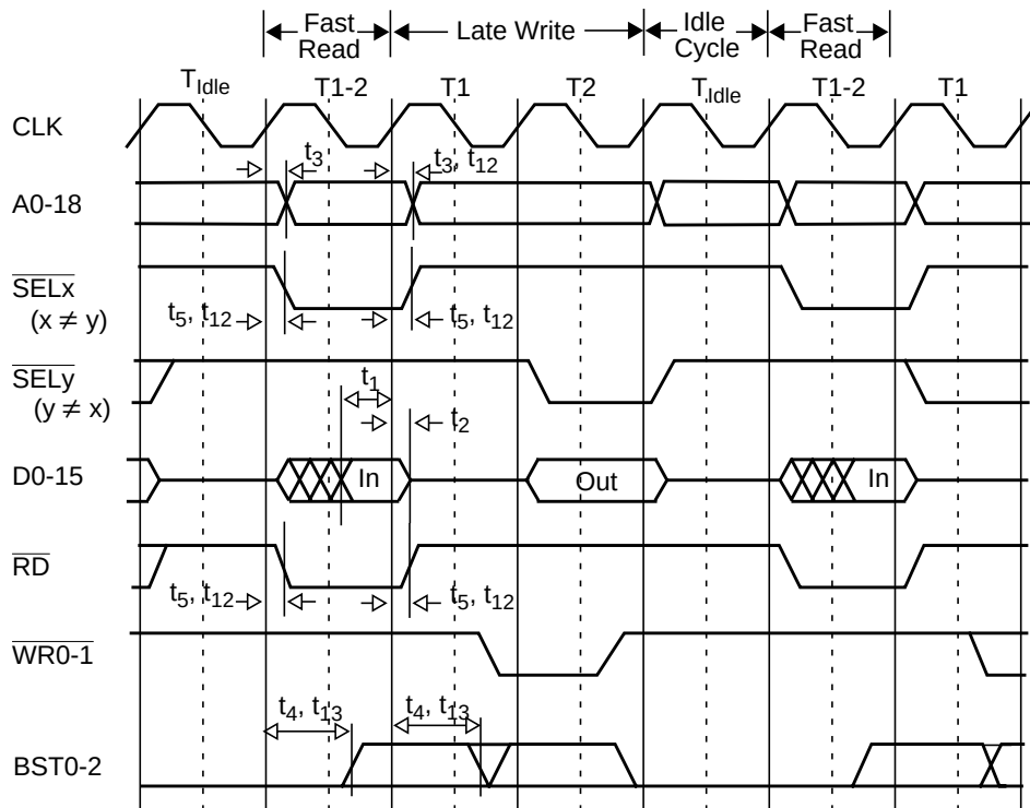
Figure 136. Fast Read Bus Cycle, AC Timing
