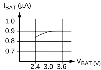
Figure 117. Typical Battery Current During Battery-Backed Power Mode
