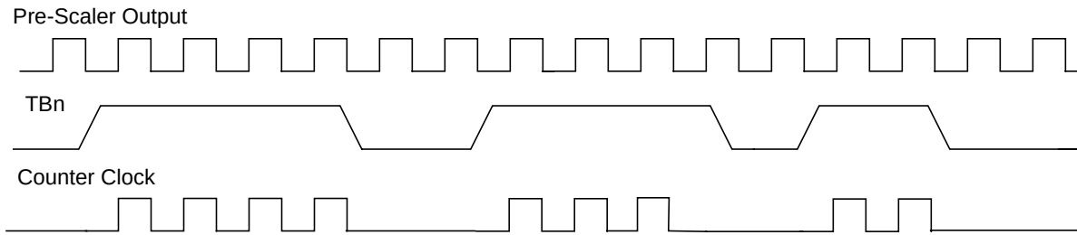
Figure 44. Pulse Accumulate Mode
