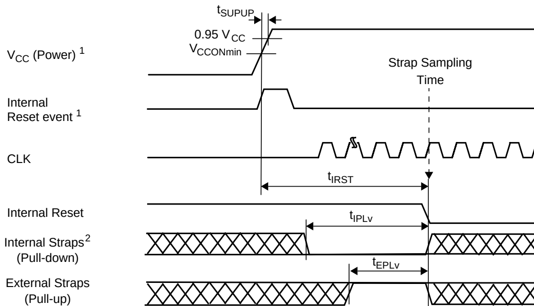
Figure 127. Internal Power-Up Reset
