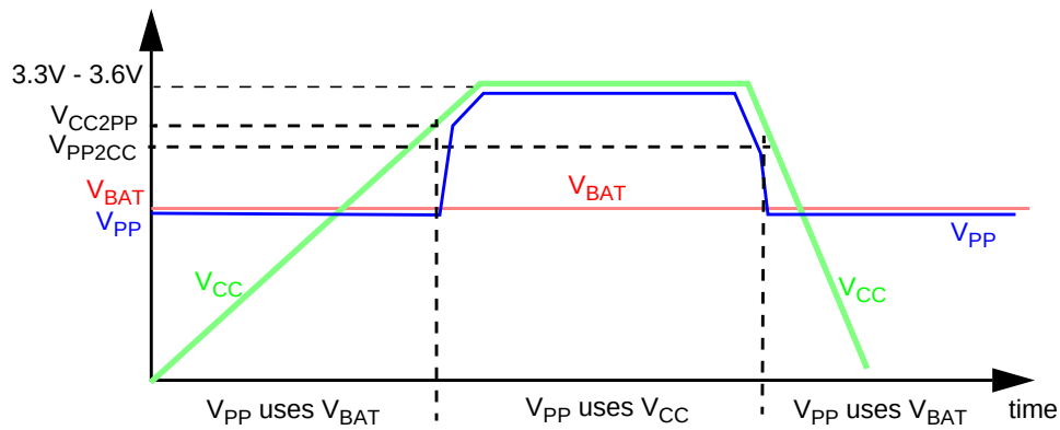
Figure 116. V_{PP} Generation Using V_{CC} or V_{BAT}
