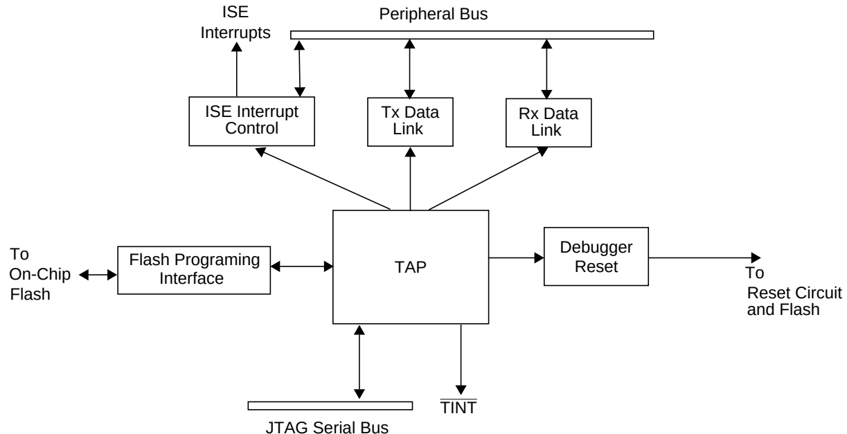
Figure 78. The Debugger Interface
