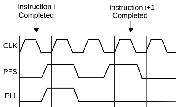
Figure 90. Pipe Status Signal (PFS and PLI)
