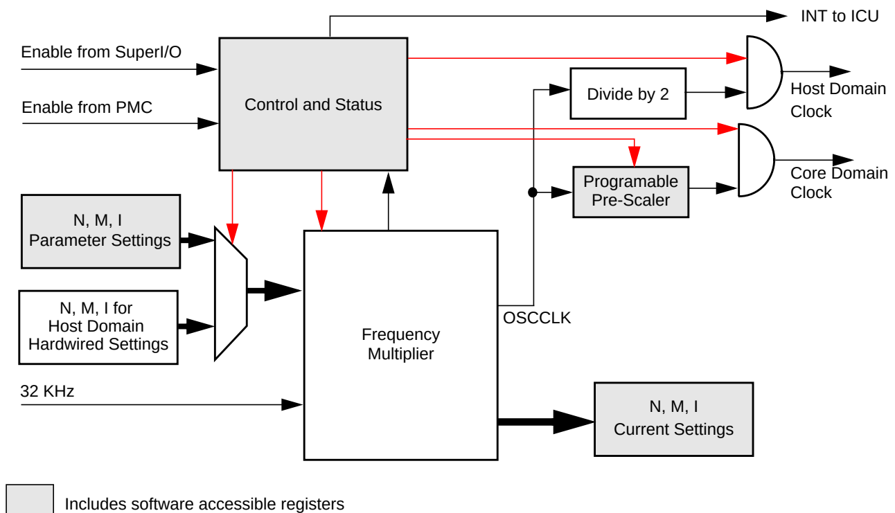
Figure 76. HFCG Schematic Diagram
