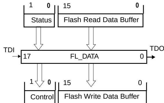
Figure 88. Flash Data Register
