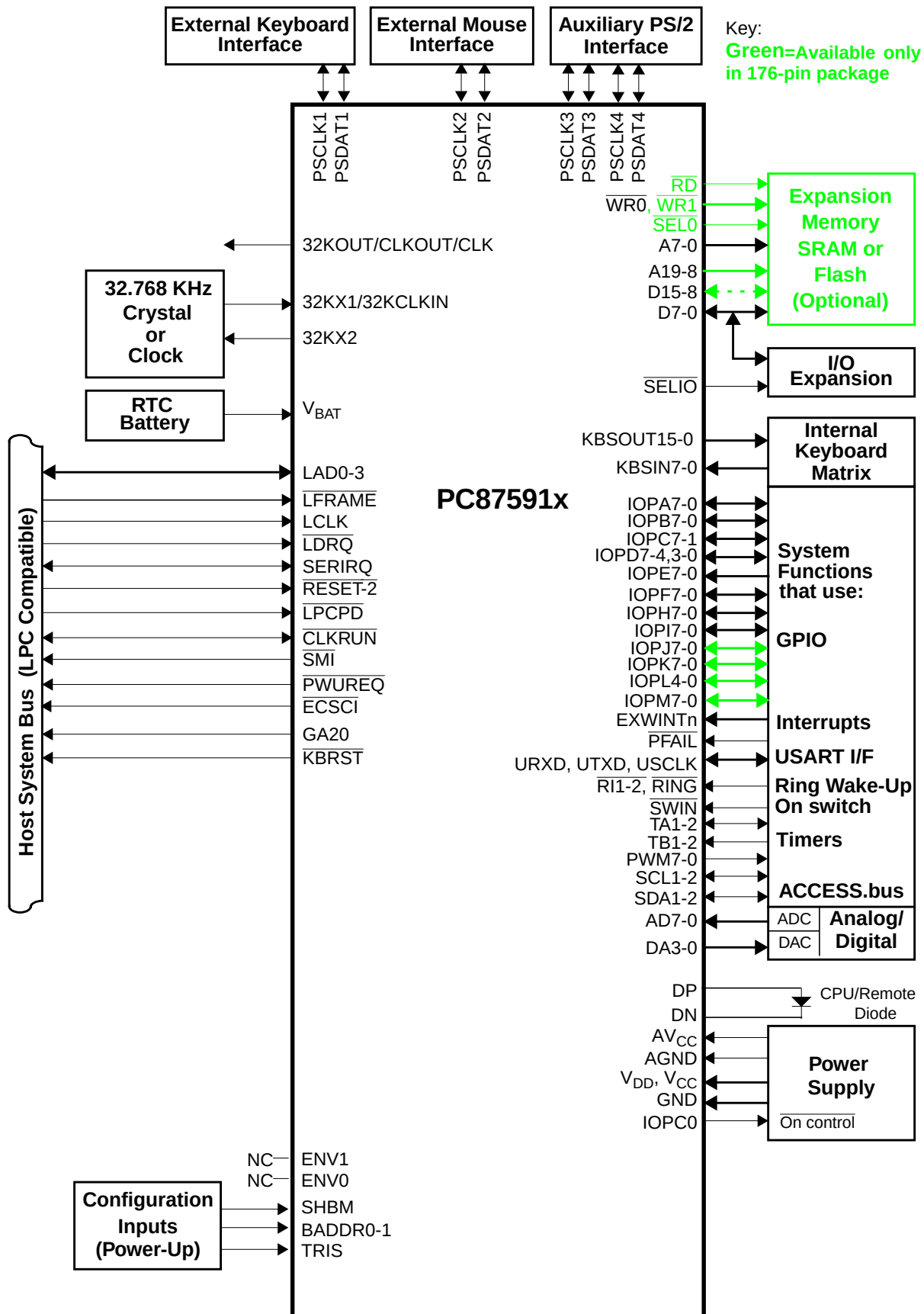
Figure 1. PC87591x System Connections Diagram, 128-Pin and 176-Pin Package
