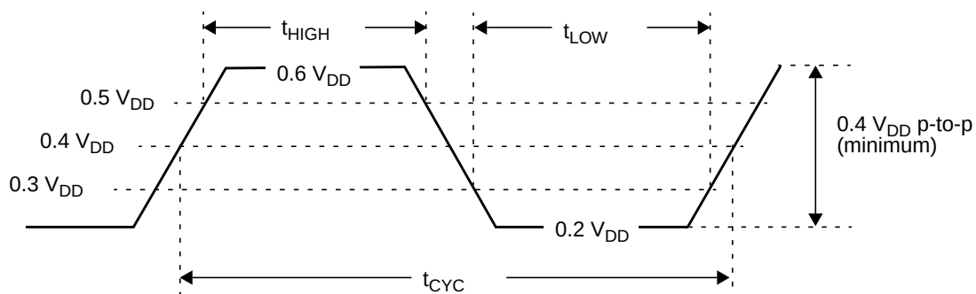
Figure 164. LCLK Waveform
