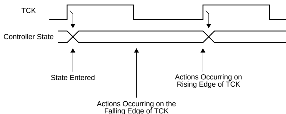
Figure 81. Timing of Actions in a Controller State
