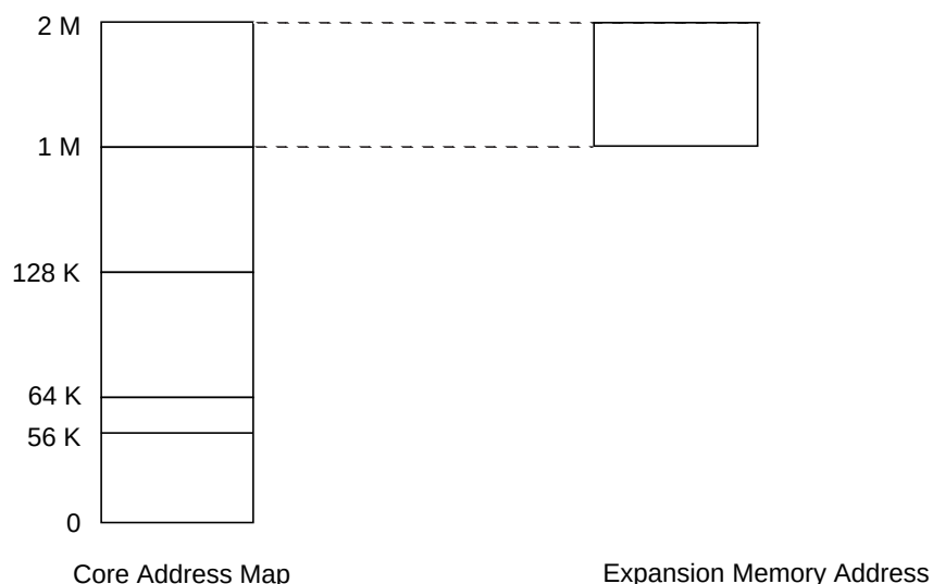
Figure 7. Expansion Memory (Zone 0) Address Range
