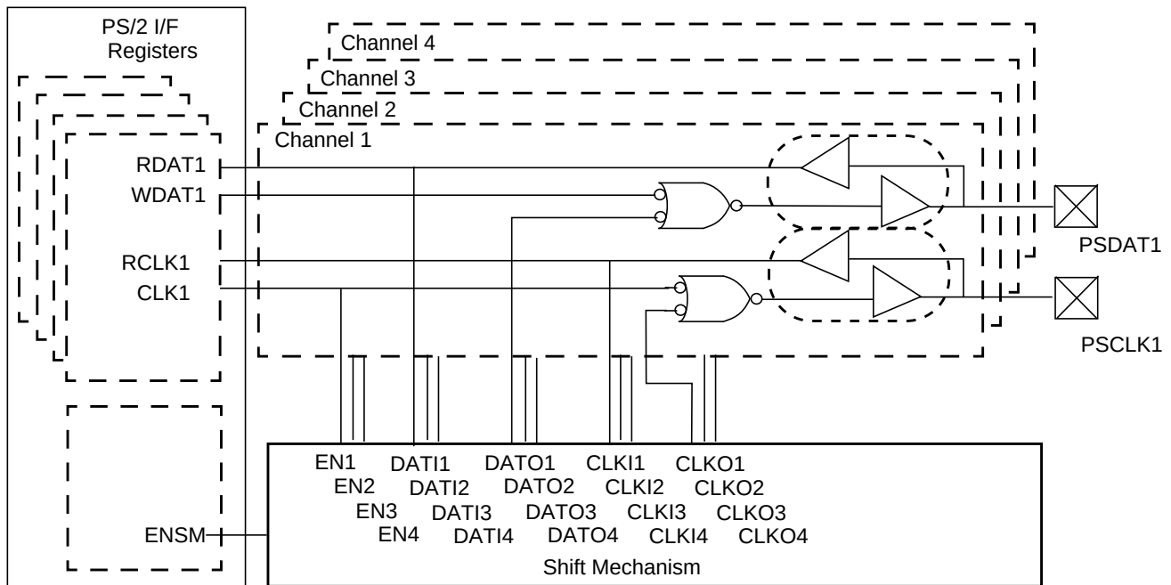
Figure 36. PS/2 Interface Functional Diagram
