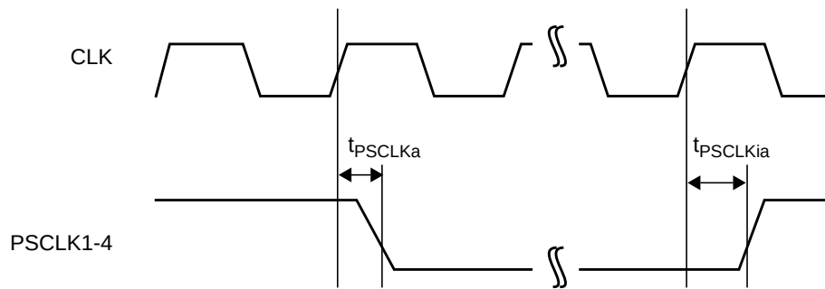
Figure 144. PS/2 Clock Signal Pulled Low by PC87591x
