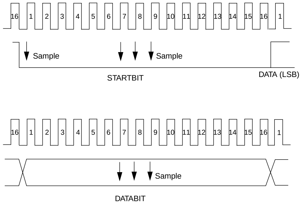
Figure 51. USART Asynchronous Communication
