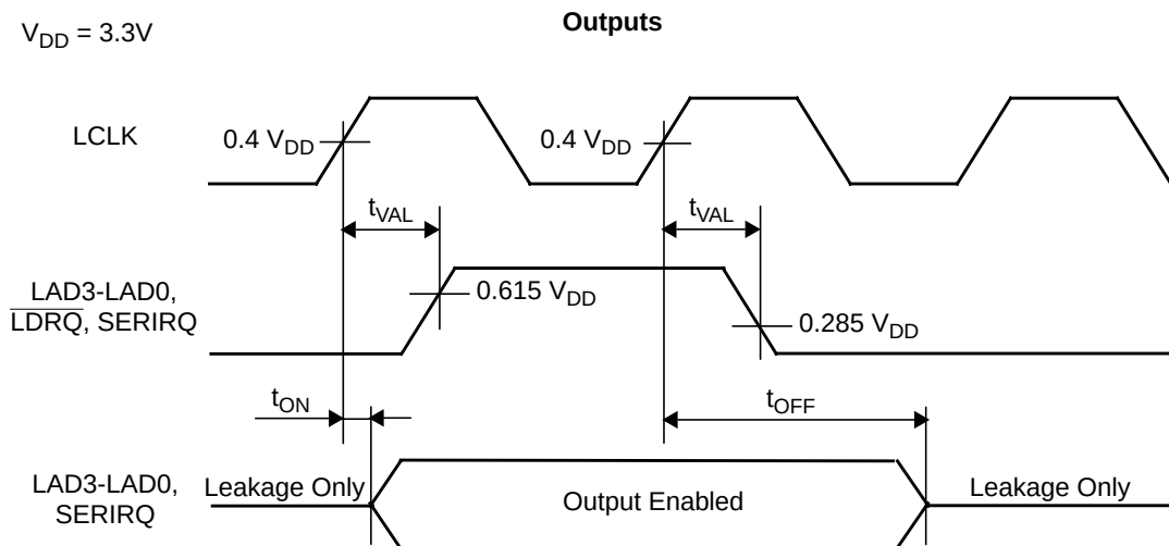
Figure 165. LPC/SERIRQ Interface Output Timing
