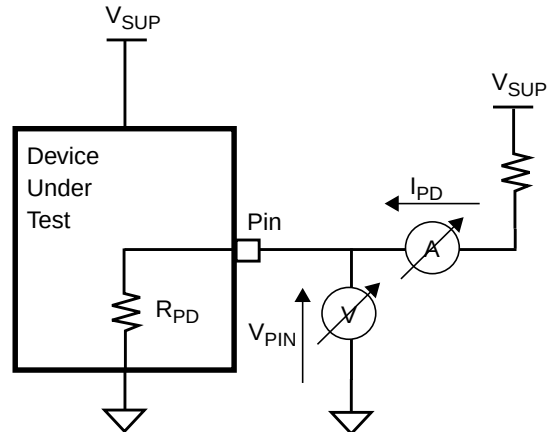
Figure 121. Internal Resistor Test Conditions, T_A = 0^{\circ}\text{C} to 70^{\circ}\text{C} , V_{SUP} = 3.3\text{V}
