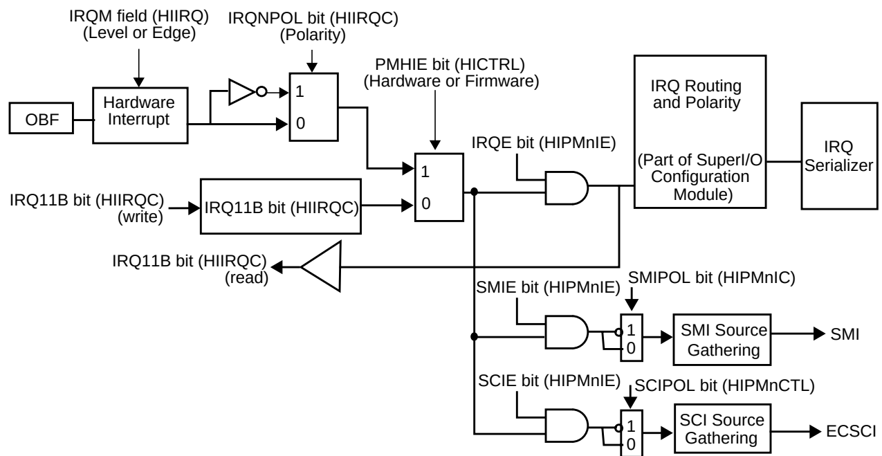
Figure 95. IRQ, SCI and SMI Control in PC87570 Compatible Mode (PM Channel 1 Only)
