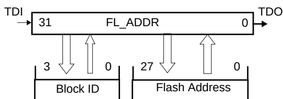
Figure 87. Flash Address Register
