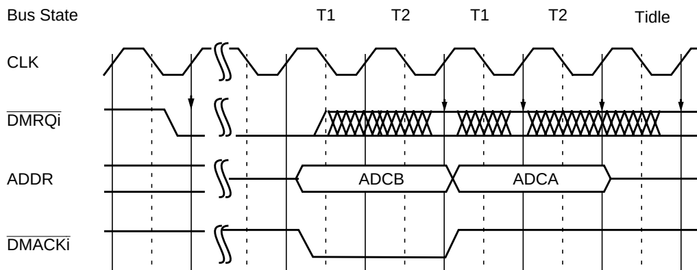
Figure 27. Indirect Bus Cycle (DIR=1) - External Bus
