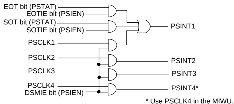
Figure 38. PS/2 Interface Interrupt Signals
