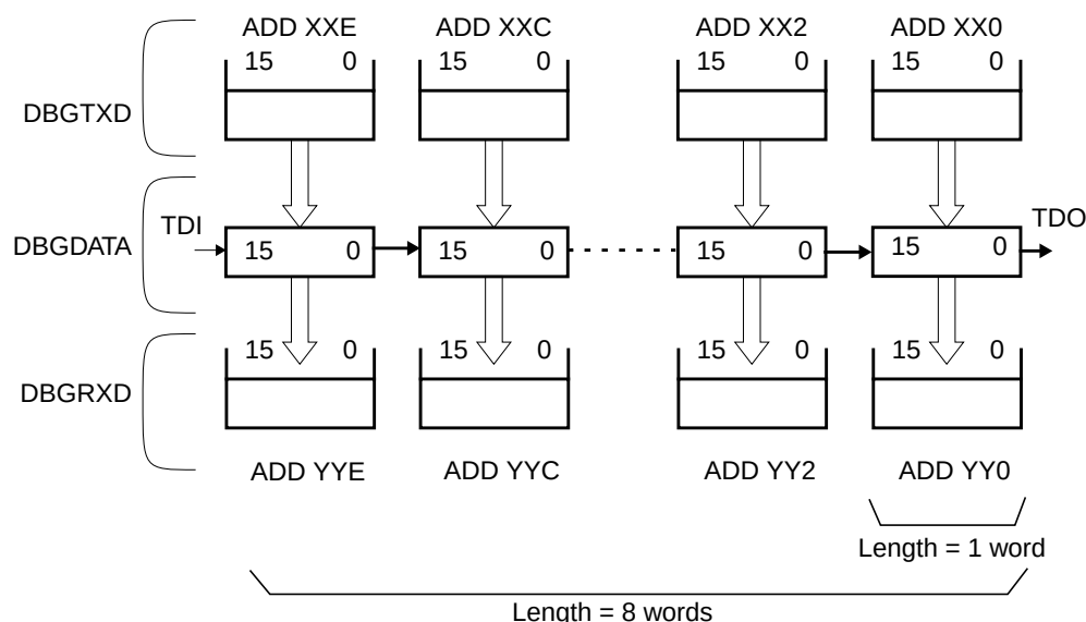
Figure 83. DBGDATA Connection to the Data Links
