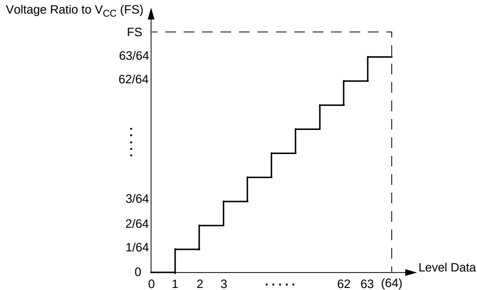
Figure 73. Level Data to Input Voltage Ratio Conversion
