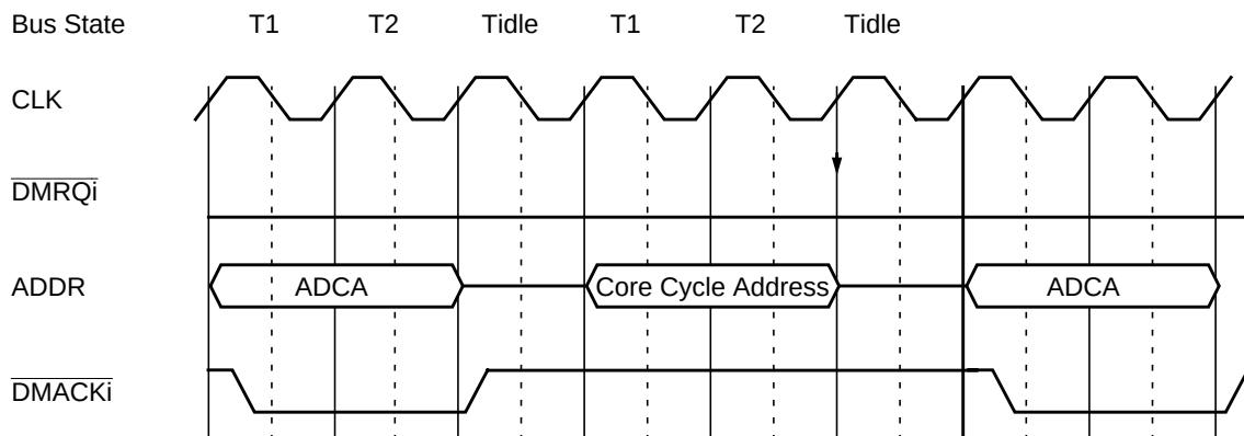
Figure 28. DMAC Direct Bus Cycles in Intermittent Mode, \overline{\text{DMRQ}} Asserted Constantly.
