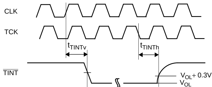
Figure 159. \overline{TINT} Output Timing
