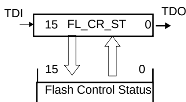
Figure 85. Flash Control and Status Register
