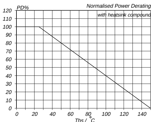
Fig.1. Normalised power dissipation. PD\% = 100 \cdot P_D / P_{D\ 25^\circ\text{C}} = f(T_{j\text{hs}})
