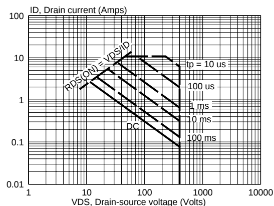
Fig.3. Safe operating area. T_{j\text{hs}} = 25^\circ\text{C} I_D & I_{DM} = f(V_{DS}) ; I_{DM} single pulse; parameter t_p
