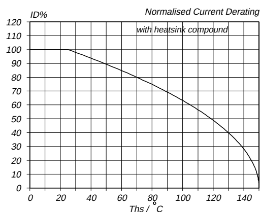
Fig.2. Normalised continuous drain current. ID\% = 100 \cdot I_D / I_{D\ 25^\circ\text{C}} = f(T_{j\text{hs}}) ; conditions: V_{GS} \geq 10\text{ V}
