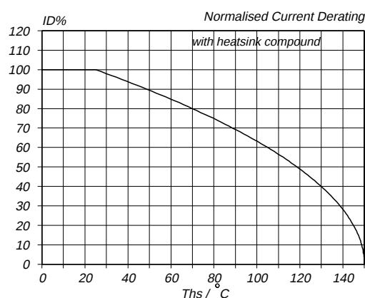
Fig.2. Normalised continuous drain current. ID\% = 100 \cdot I_D / I_{D\ 25^\circ\text{C}} = f(T_{hs}); \text{ conditions: } V_{GS} \geq 10\text{ V}
