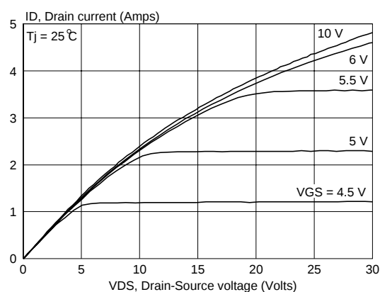
Fig.5. Typical output characteristics. I_D = f(V_{DS}); \text{ parameter } V_{GS}
