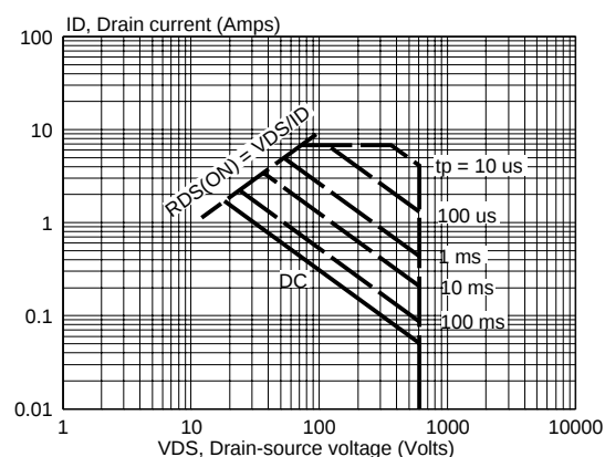
Fig.3. Safe operating area. T_{hs} = 25^\circ\text{C} I_D \text{ \& } I_{DM} = f(V_{DS}); I_{DM} \text{ single pulse; parameter } t_p
