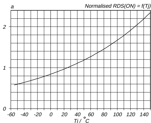
Fig. 9. Normalised drain-source on-state resistance. a = R_{DS(ON)}/R_{DS(ON)25^\circ\text{C}} = f(T_j) ; I_D = 6\text{ A} ; V_{GS} = 10\text{ V}
