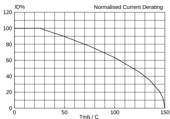
Fig.2. Normalised continuous drain current. ID\% = 100 \cdot I_D / I_{D\ 25\ ^\circ C} = f(T_{mb}) ; conditions: V_{GS} \geq 10\ V
