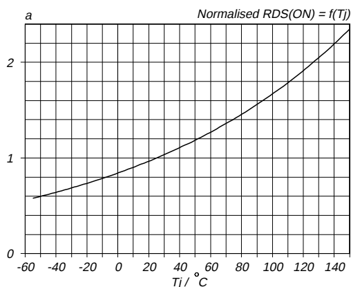
Fig. 9. Normalised drain-source on-state resistance. a = R_{DS(ON)}/R_{DS(ON)25 \text{ °C}} = f(T_j) ; I_D = 2 \text{ A} ; V_{GS} = 10 \text{ V}
